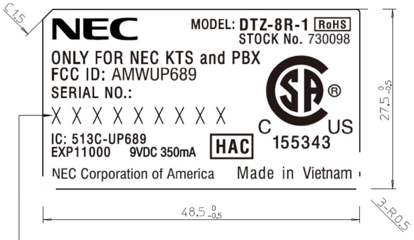
DTZ-8R-1 Base FCC ID (48.5 mm (W) x 27.5 mm (H))
