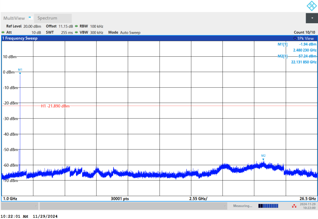
BLE_2M-Ant1-2480-1000~26500-PASS
