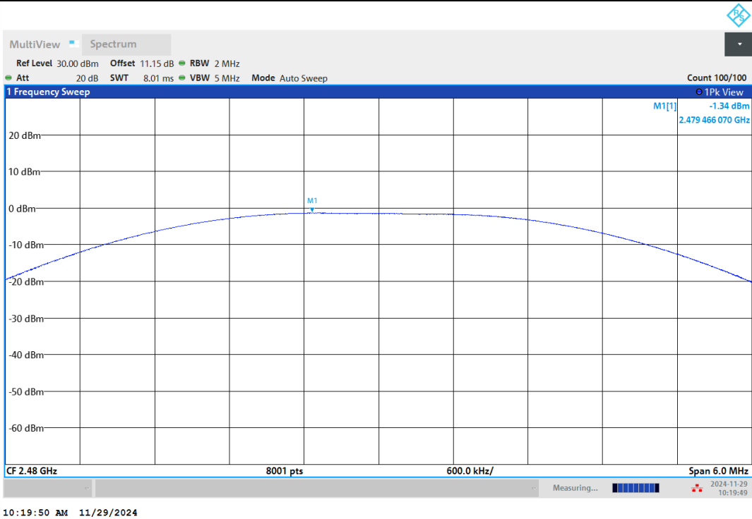
BLE_2M-Ant1-2480-PASS
