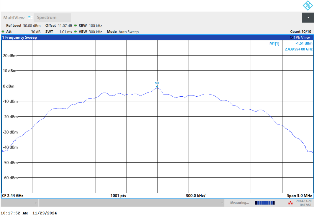
BLE_2M-Ant1-2440-0~Reference-PASS
