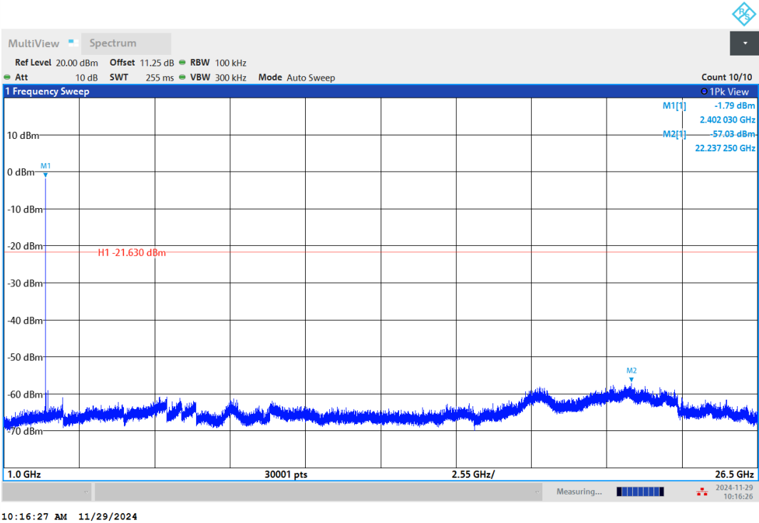
BLE_2M-Ant1-2402-1000~26500-PASS
