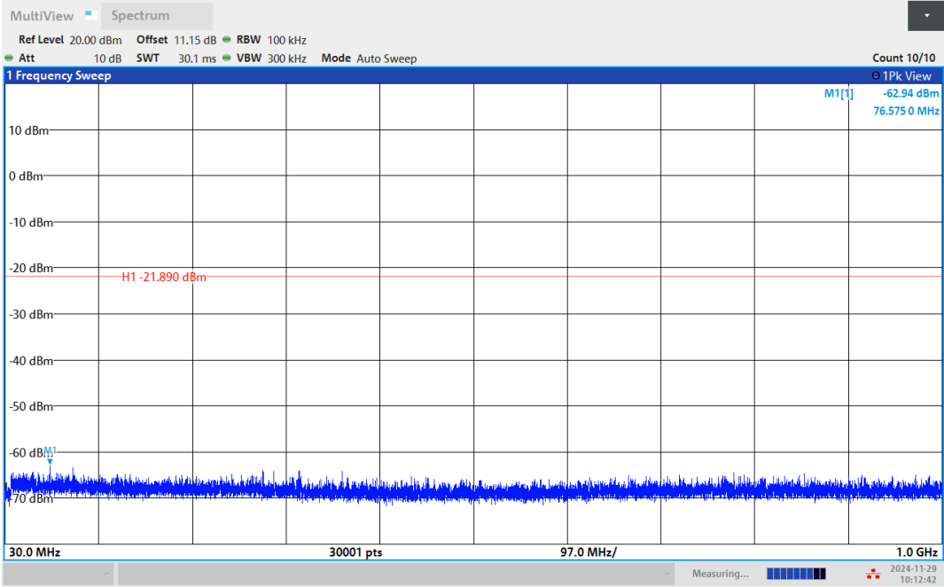
BLE_1M-Ant1-2480-30~1000-PASS
