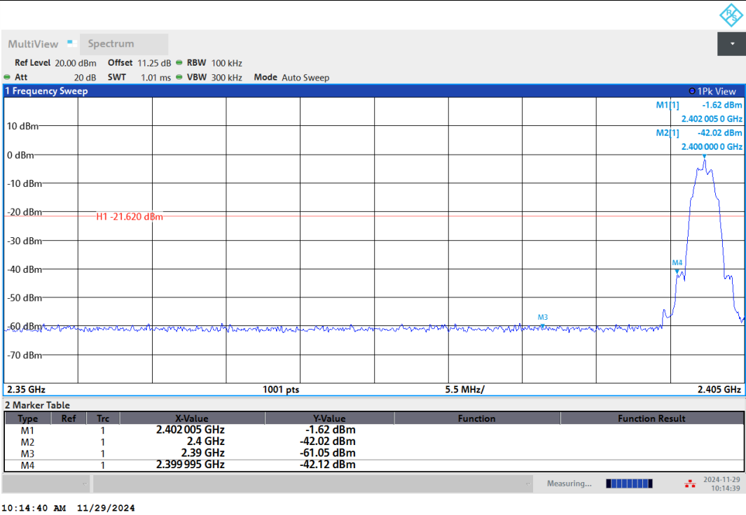
BLE_2M-Ant1-2402-PASS
