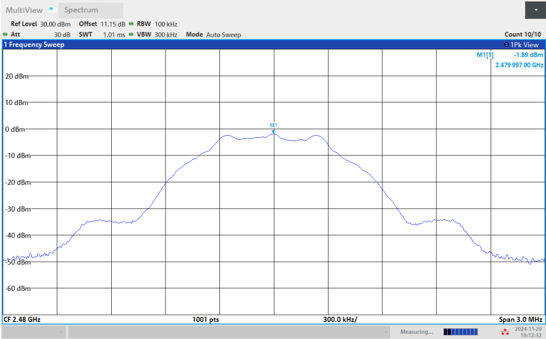
BLE_1M-Ant1-2480-0~Reference-PASS
