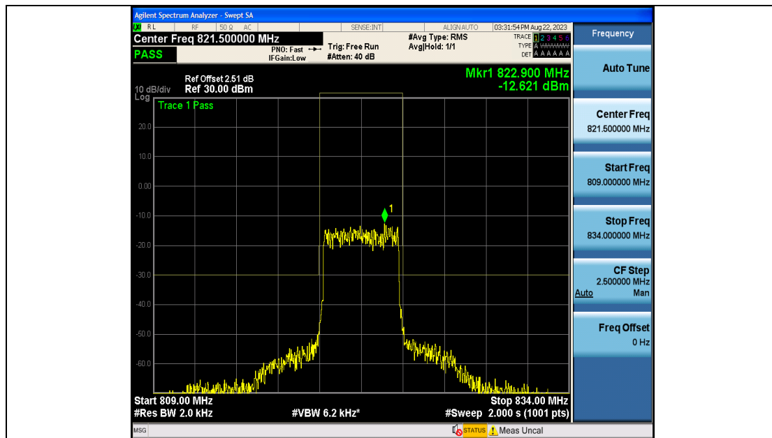
Band18_5MHz_QPSK_23915_25RB#0
