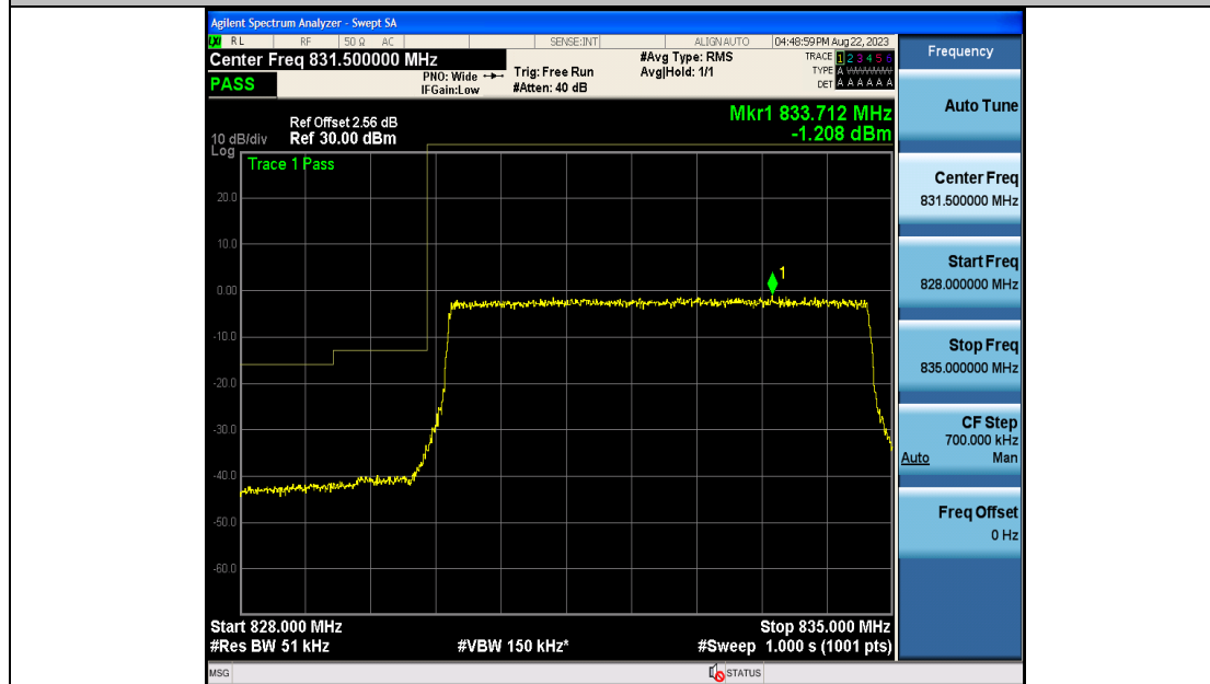
Band19_5MHz_16QAM_24025_25RB#0
