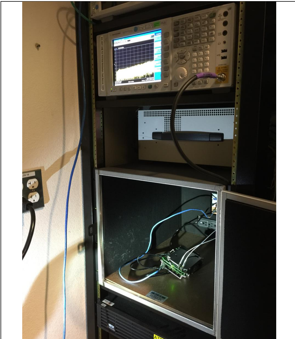
Title: Conducted Test Setup
