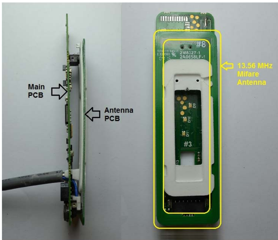
T15 Mifare - 13.56 MHz Mifare Antenna and Main PCB
