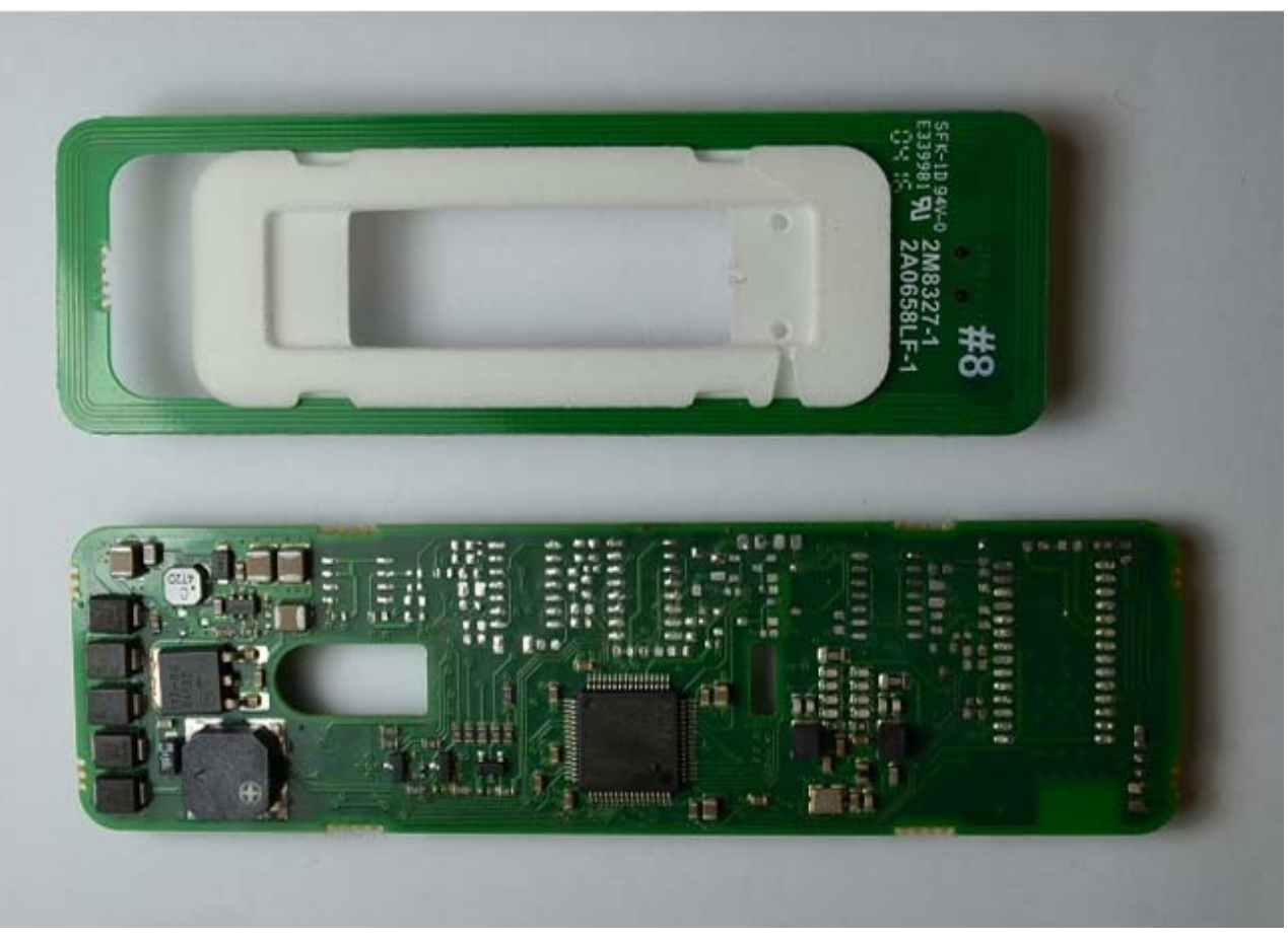
T15 Mifare - Main and Antenna PCB (Rear)
