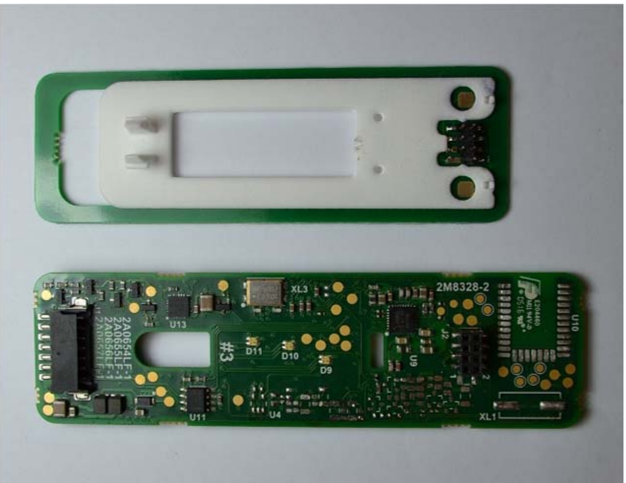
T15 Mifare - Main and Antenna PCB (Front)
