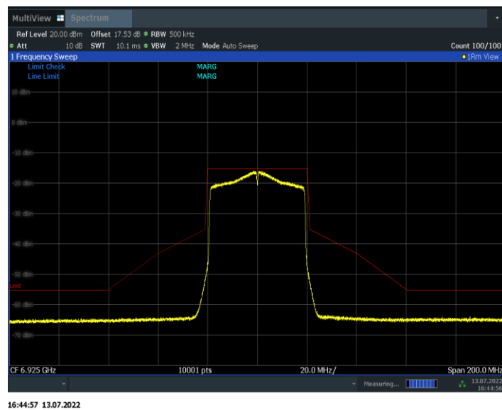
Fig.155 In-Band Emissions (802.11ax-HE40, 6925MHz)
