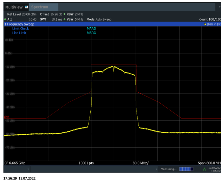
Fig.173 In-Band Emissions (802. 11ax-HE160, 6665MHz)
