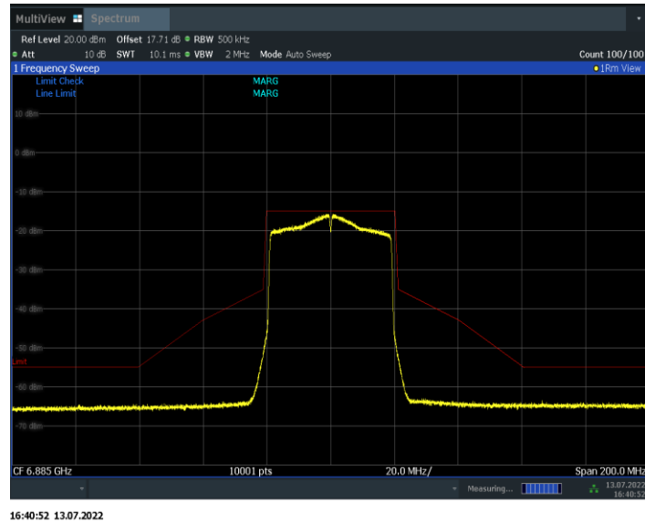
Fig.154 In-Band Emissions (802.11ax-HE40, 6885MHz)
