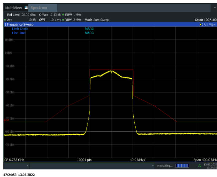
Fig.165 In-Band Emissions (802. 11ax-HE80, 6785MHz)
