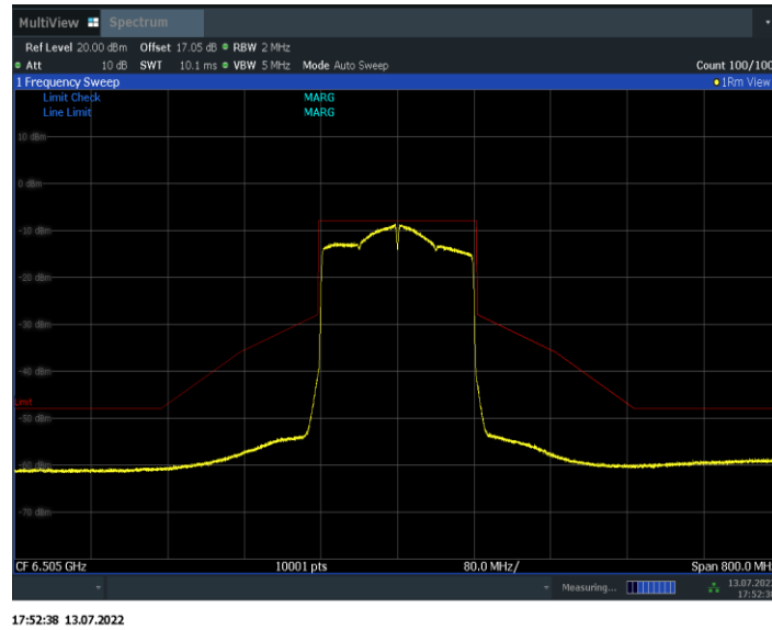
Fig.172 In-Band Emissions (802. 11ax-HE160, 6505MHz)
