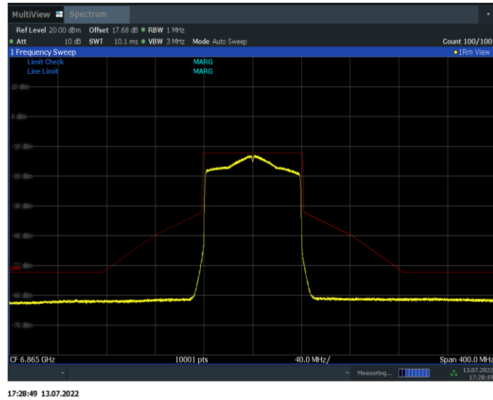
Fig.166 In-Band Emissions (802. 11ax-HE80, 6865MHz)
