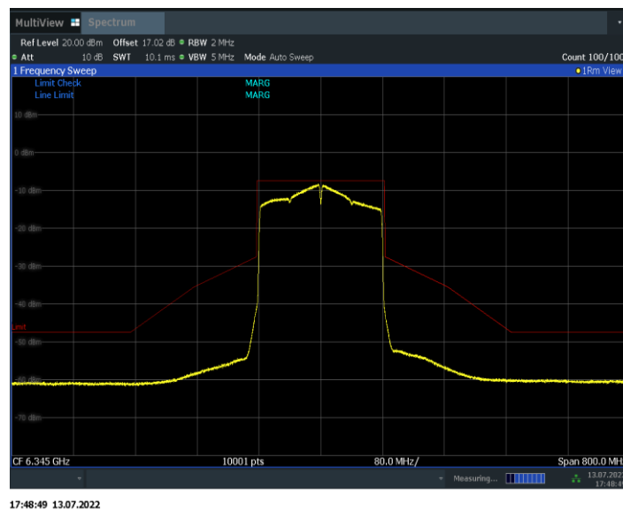
Fig.171 In-Band Emissions (802. 11ax-HE160, 6345MHz)
