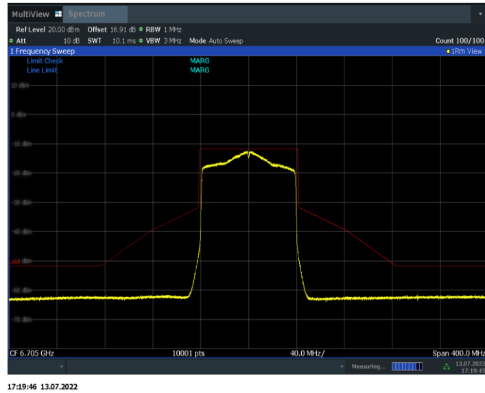
Fig.164 In-Band Emissions (802. 11ax-HE80, 6705MHz)
