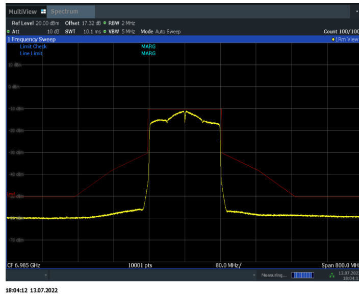
Fig.175 In-Band Emissions (802. 11ax-HE160 6985MHz)
