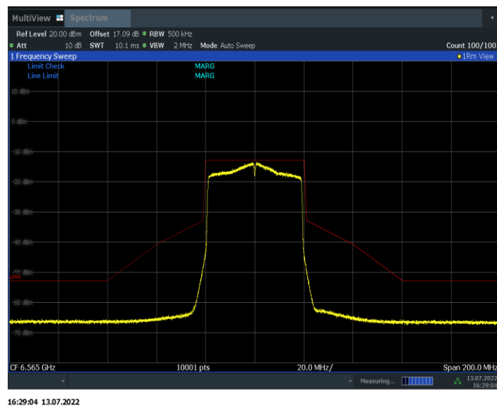
Fig.151 In-Band Emissions (802.11ax-HE40, 6565MHz)
