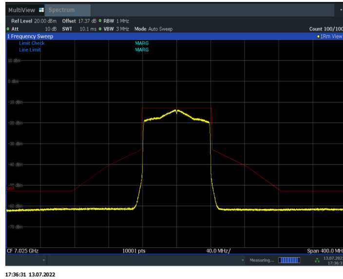
Fig.168 In-Band Emissions (802. 11ax-HE80, 7025MHz)
