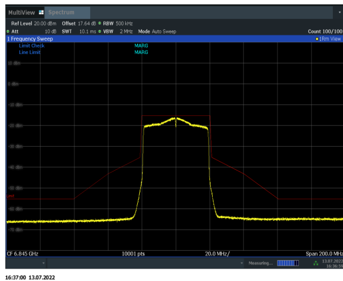
Fig.153 In-Band Emissions (802.11ax-HE40, 6845MHz)
