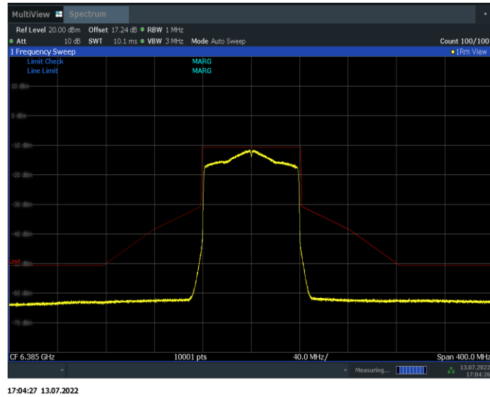
Fig.160 In-Band Emissions (802. 11ax-HE80, 6385MHz)
