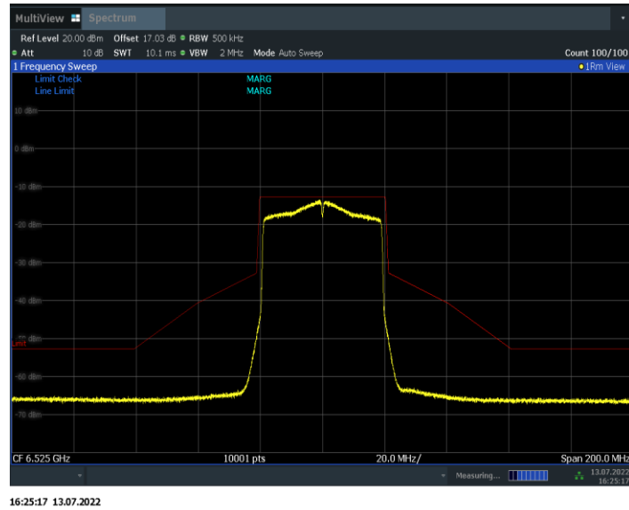
Fig.150 In-Band Emissions (802.11ax-HE40, 6525MHz)
