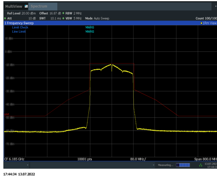
Fig.170 In-Band Emissions (802. 11ax-HE160, 6185MHz)
