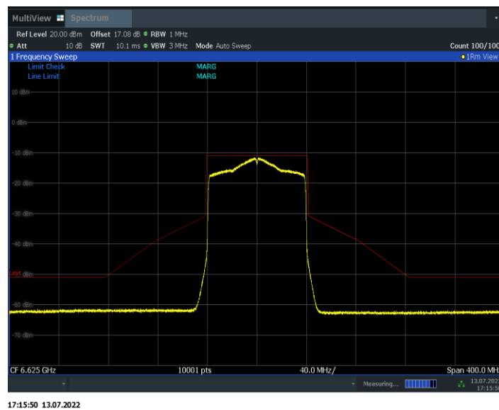
Fig.163 In-Band Emissions (802. 11ax-HE80, 6625MHz)
