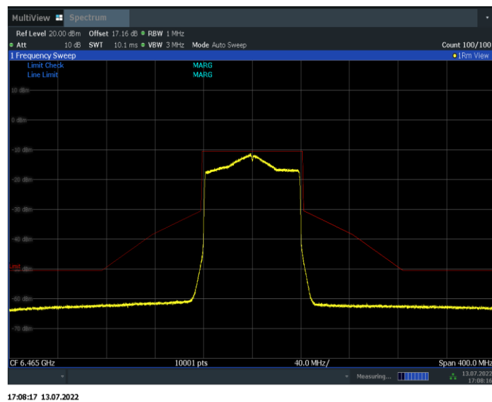
Fig.161 In-Band Emissions (802. 11ax-HE80, 6465MHz)
