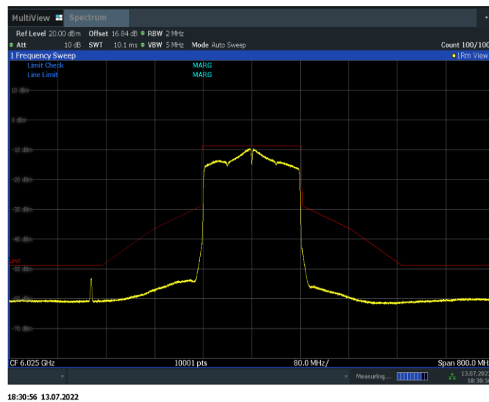
Fig.169 In-Band Emissions (802. 11ax-HE160, 6025MHz)
