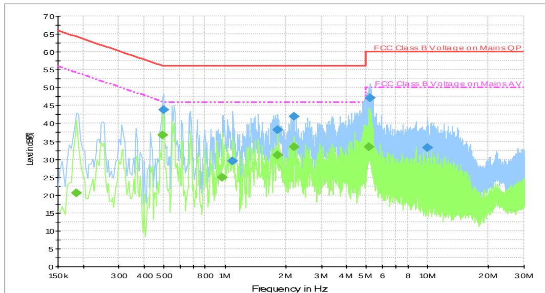
Fig. 187 AC Power line Conducted Emission-802.11a
