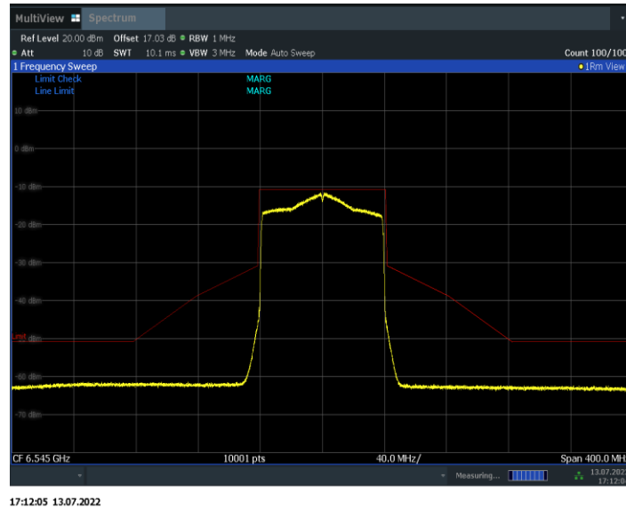
Fig.162 In-Band Emissions (802. 11ax-HE80, 6545MHz)
