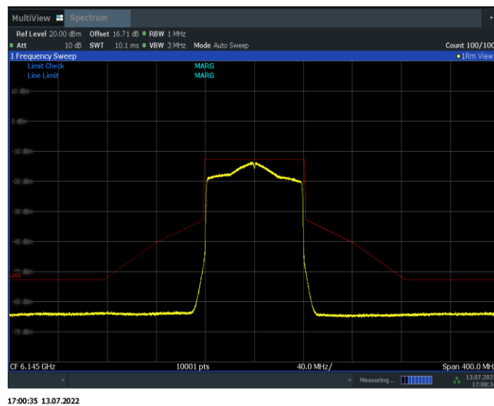
Fig.159 In-Band Emissions (802. 11ax-HE80, 6145MHz)
