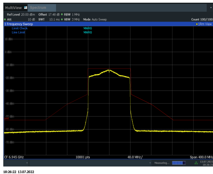
Fig.167 In-Band Emissions (802. 11ax-HE80, 6945MHz)
