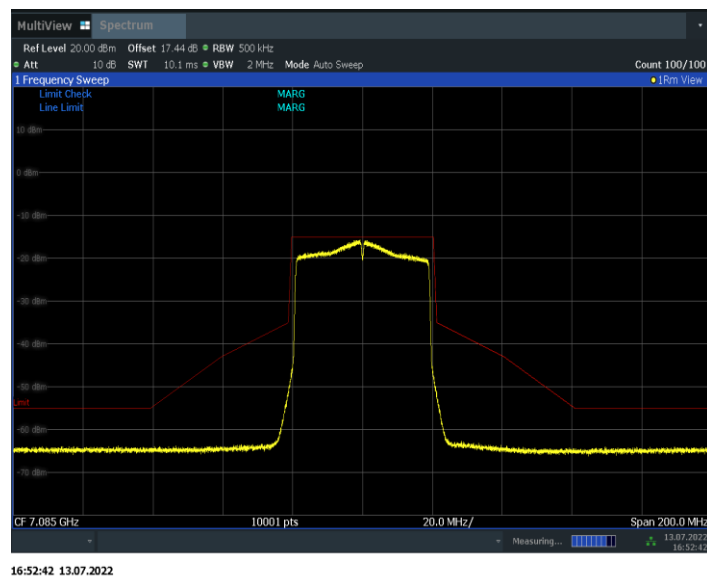
Fig.157 In-Band Emissions (802.11ax-HE40, 7085MHz)
