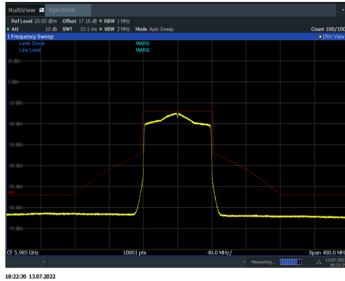
Fig.158 In-Band Emissions (802. 11ax-HE80, 5985MHz)
