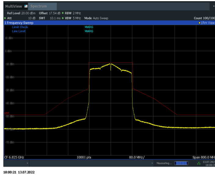
Fig.174 In-Band Emissions (802. 11ax-HE160, 6825MHz)
