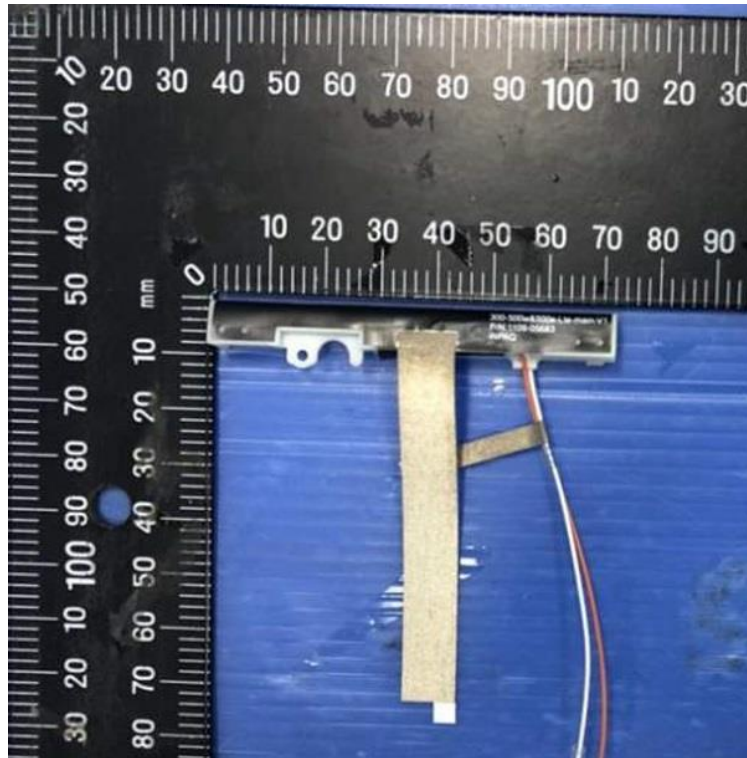
INPAQ Corporation WWAN antenna
