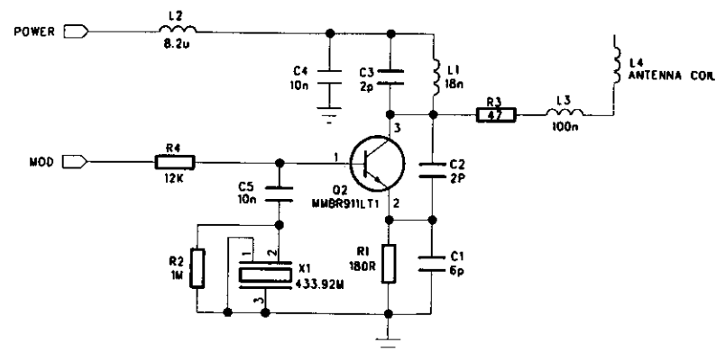
UHF TRANSMITTER
