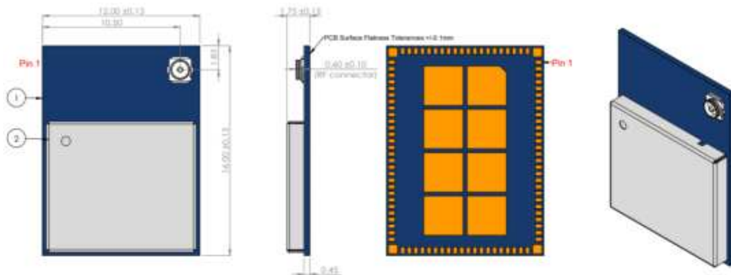
Figure 10: M.2 1216 (MHF4 variant)
