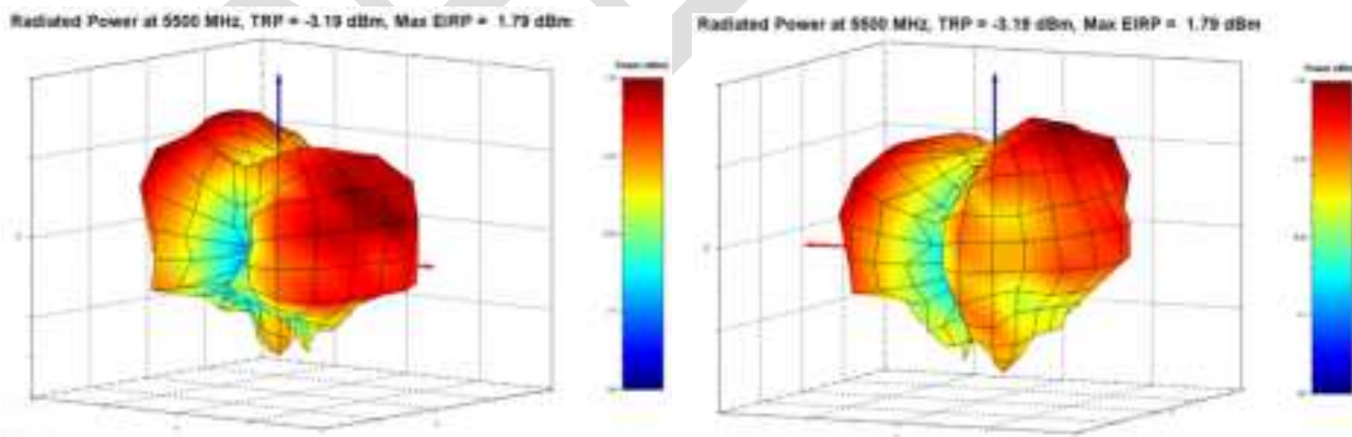
Figure 32: Sona TI351 Total Gain Radiated Pattern at 5500 MHz
