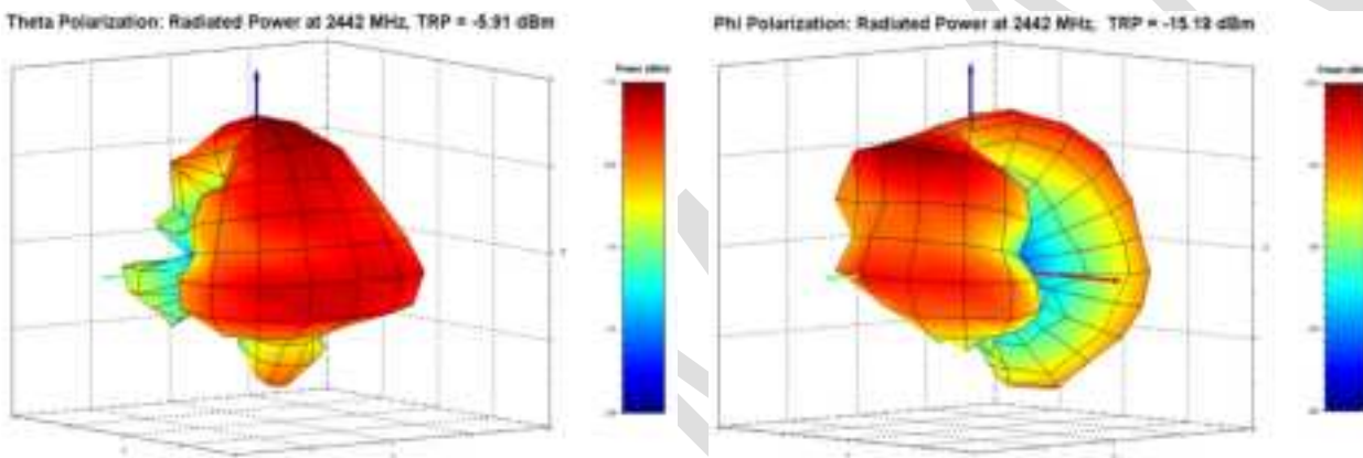
Figure 31: Sona TI351 Theta and Phi Polarization Radiated Patterns at 2442 MHz
