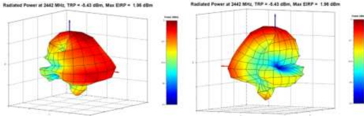
Figure 30: Sona TI351 Total Gain Radiated Pattern at 2442 MHz
