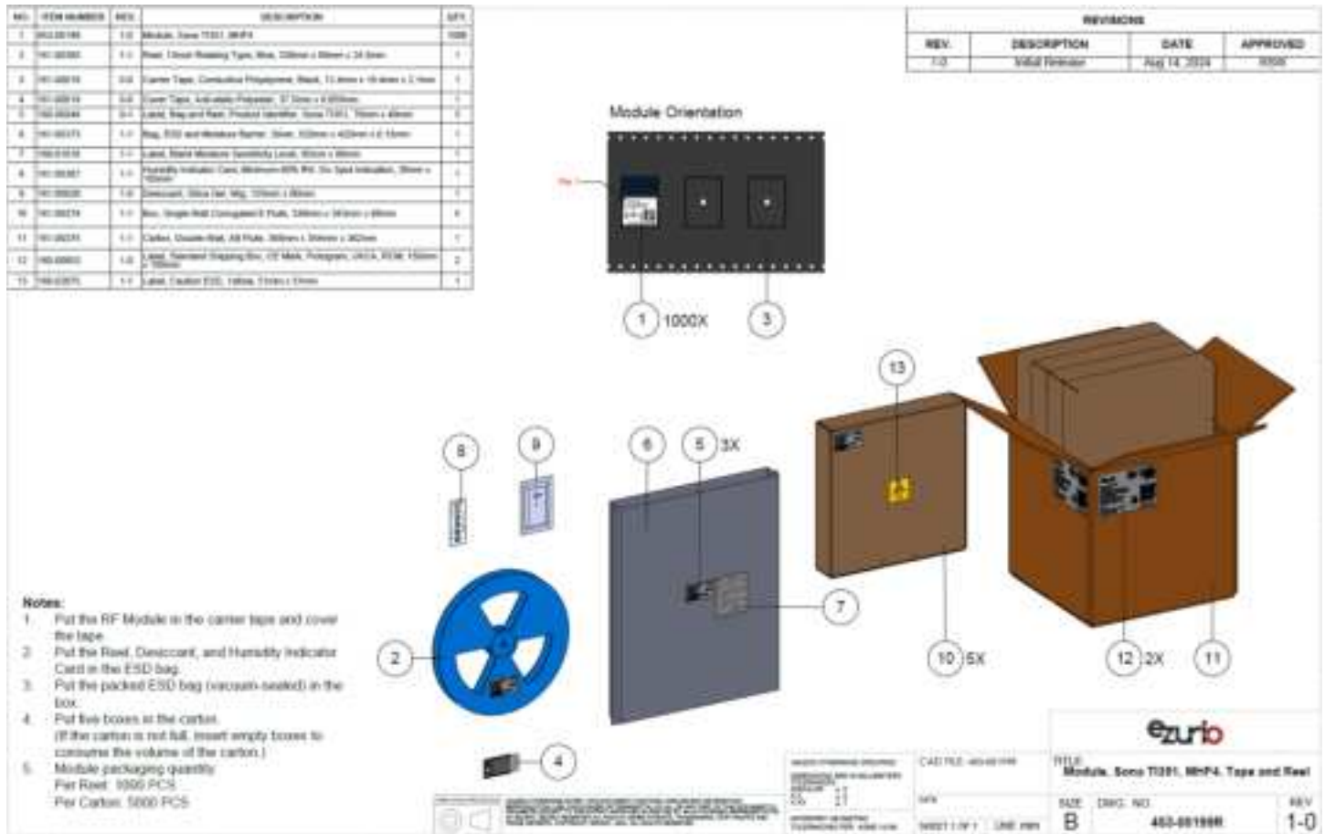
Figure 16: Sona TI351 packaging processes, 453-00199R
