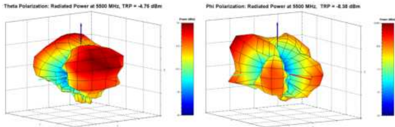
Figure 33: Sona TI351 Theta and Phi Polarization Radiated Patterns at 5500 MHz
