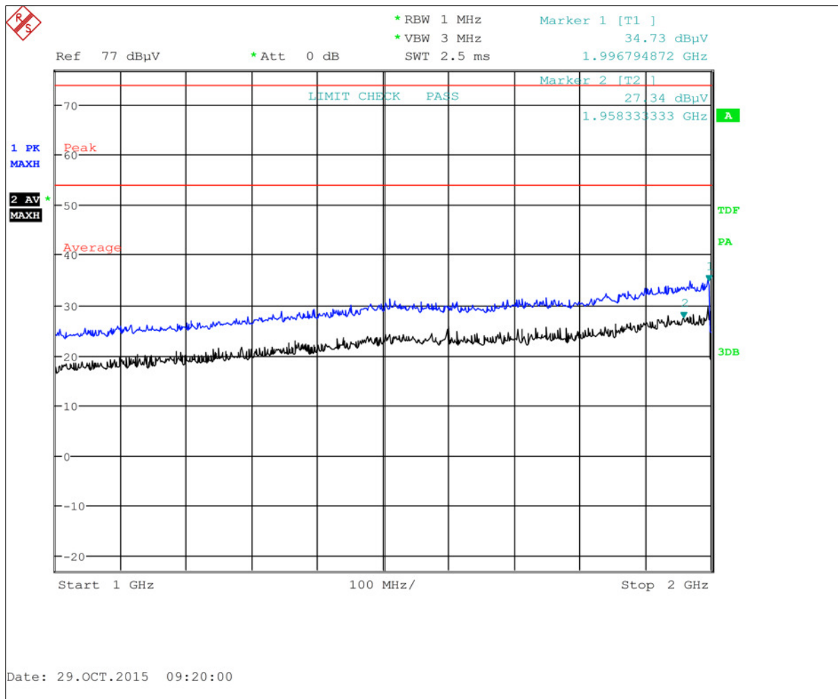
Plot 6-554: Radiated Emissions 1 GHz – 2 GHz Horizontal Peak/Average
