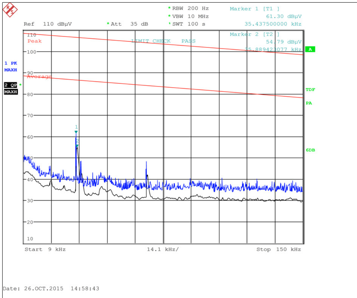
Plot 6-546: Radiated Emissions Transmit – 9 kHz – 150 kHz Horizontal Peak/Average
