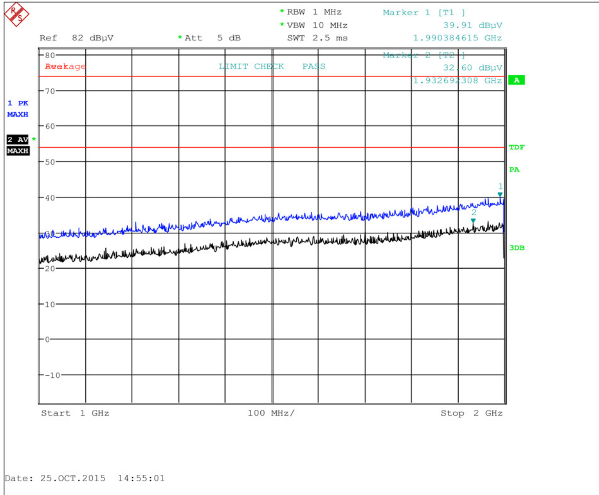
Plot 6-533: Radiated Emissions 1 GHz – 2 GHz Horizontal Peak/Average
