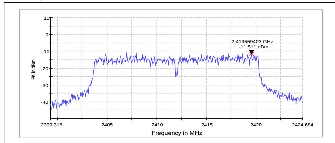
Channel 1 / 2412 MHz
