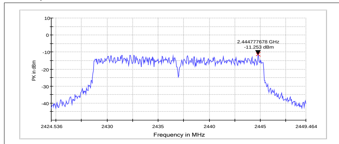
Channel 6 / 2437 MHz
