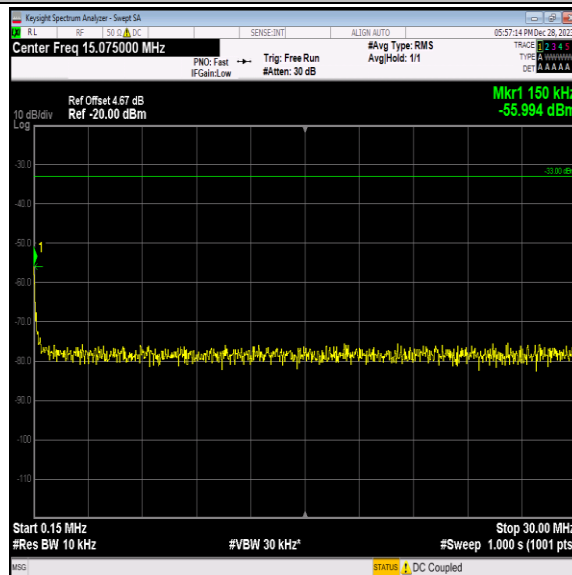
Band2-9538-2-0.15~30MHz-PASS
