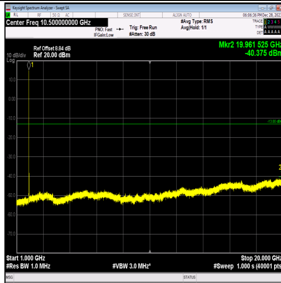
Band2-9400-5-1000~20000MHz-PASS
