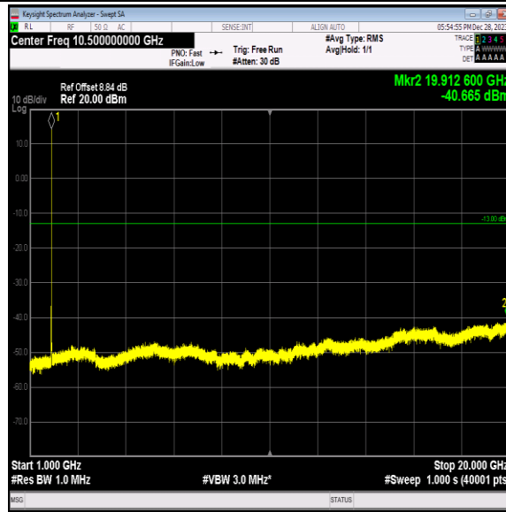
Band2-9262-2-1000~20000MHz-PASS
