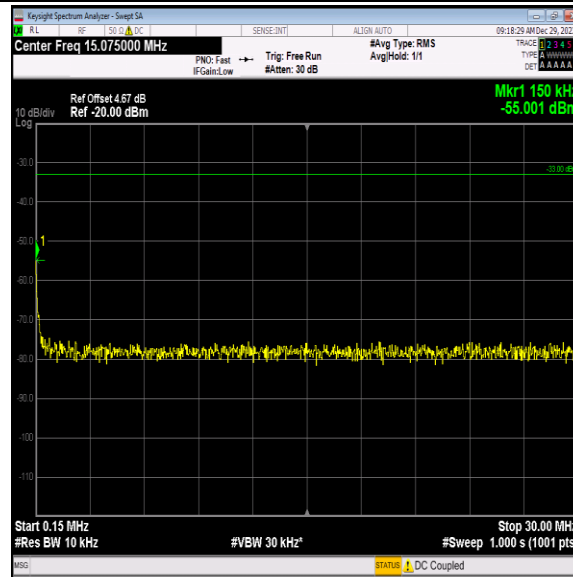
Band4-1312-3-0.15~30MHz-PASS
