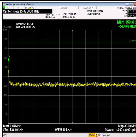
Band2-9538-1-0.15~30MHz-PASS
