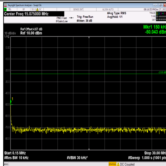
Band5-4233-3-0.15~30MHz-PASS
