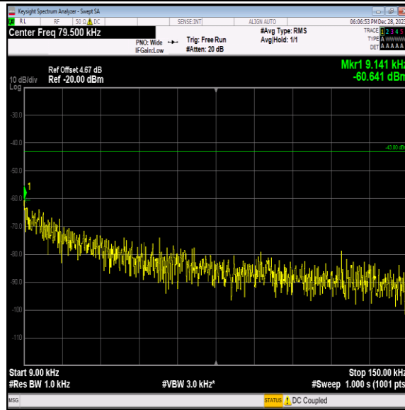
Band2-9538-5-0.009~0.15MHz-PASS
