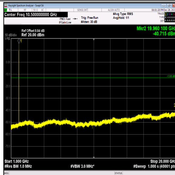
Band2-9538-3-1000~20000MHz-PASS
