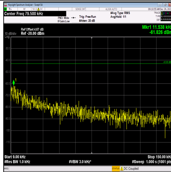
Band4-1312-1-0.009~0.15MHz-PASS
