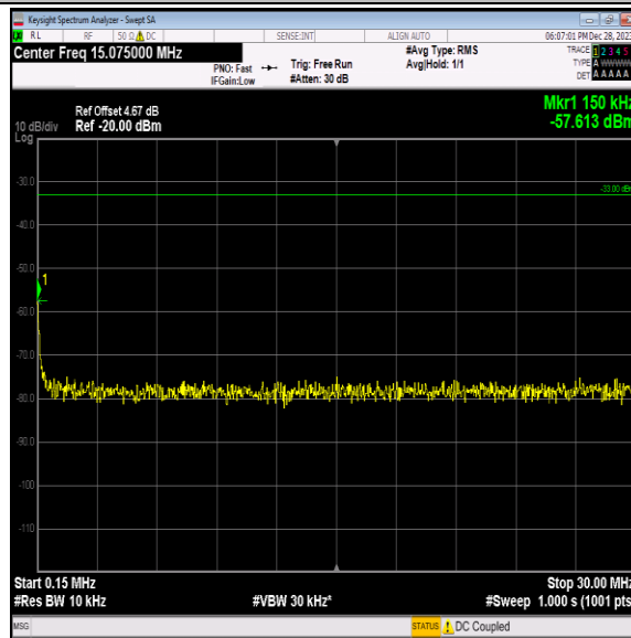
Band2-9538-5-0.15~30MHz-PASS
