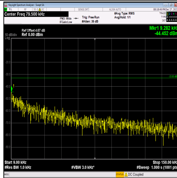
Band5-4233-4-0.009~0.15MHz-PASS
