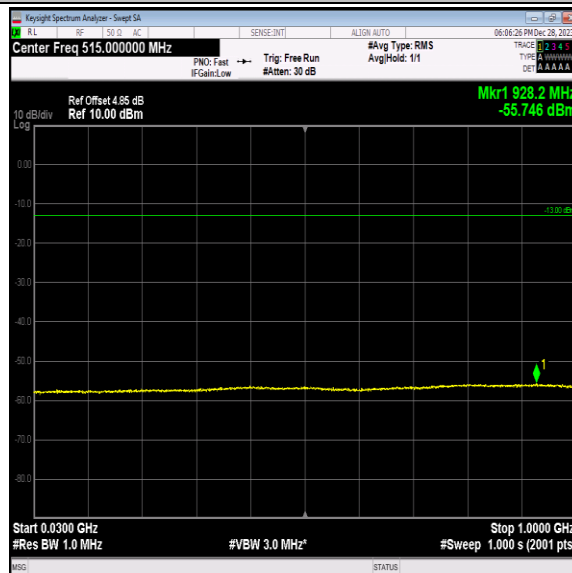
Band2-9400-5-30~1000MHz-PASS
