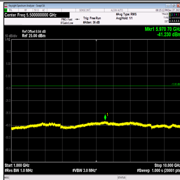
Band5-4233-2-1000~10000MHz-PASS
