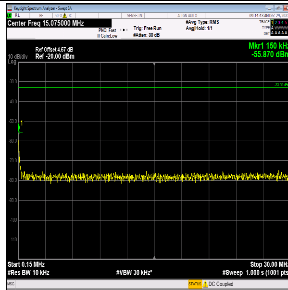
Band4-1312-2-0.15~30MHz-PASS
