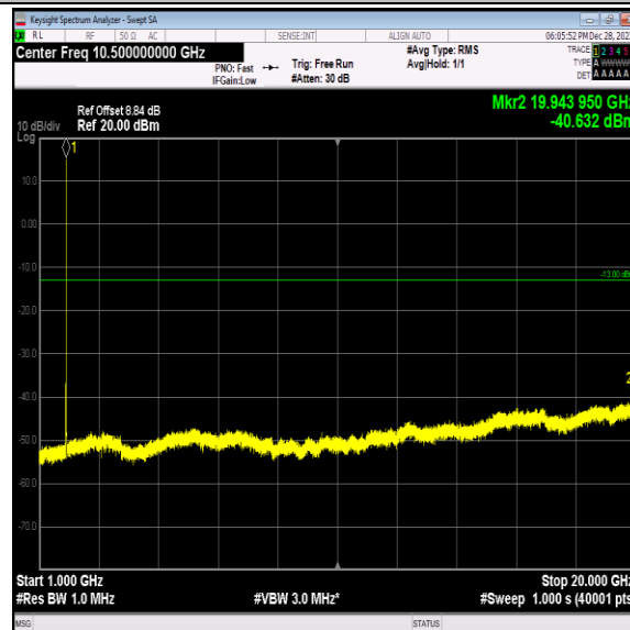
Band2-9262-5-1000~20000MHz-PASS
