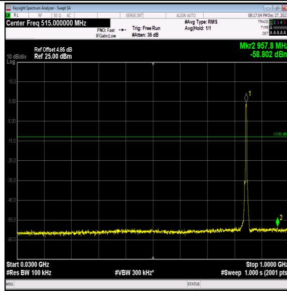
Band5-4233-3-30~1000MHz-PASS
