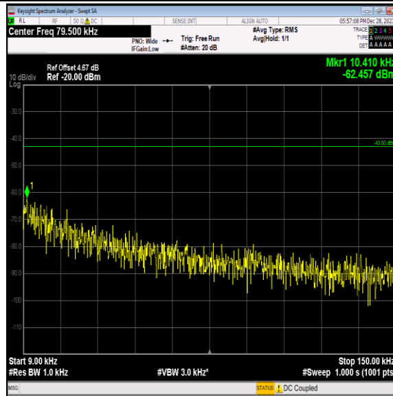
Band2-9538-2-0.009~0.15MHz-PASS
