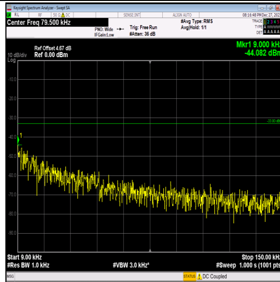
Band5-4233-3-0.009~0.15MHz-PASS
