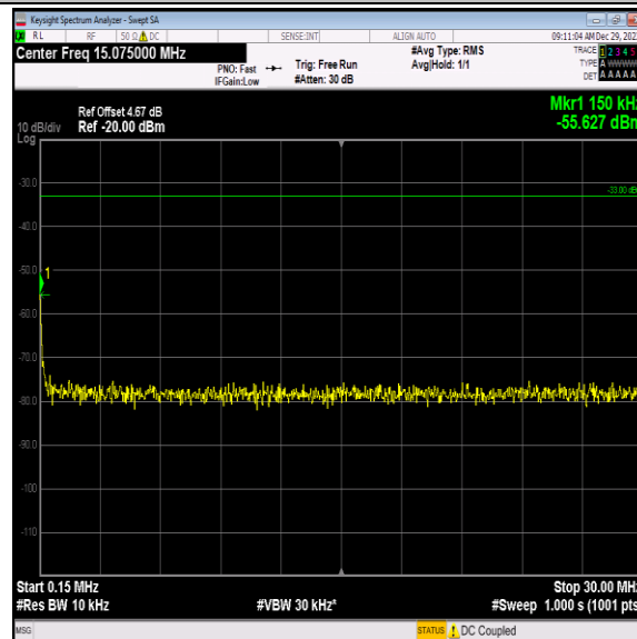
Band4-1312-1-0.15~30MHz-PASS
