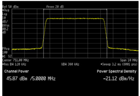
LTE5_ Middle Channel_256QAM_Average
