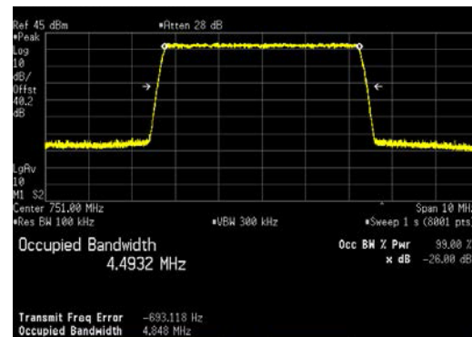
LTE5_256QAM
