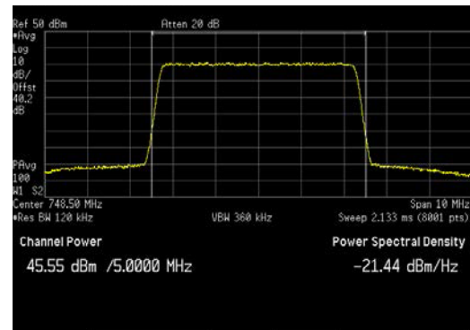
LTE5_Bottom Channel_Average
