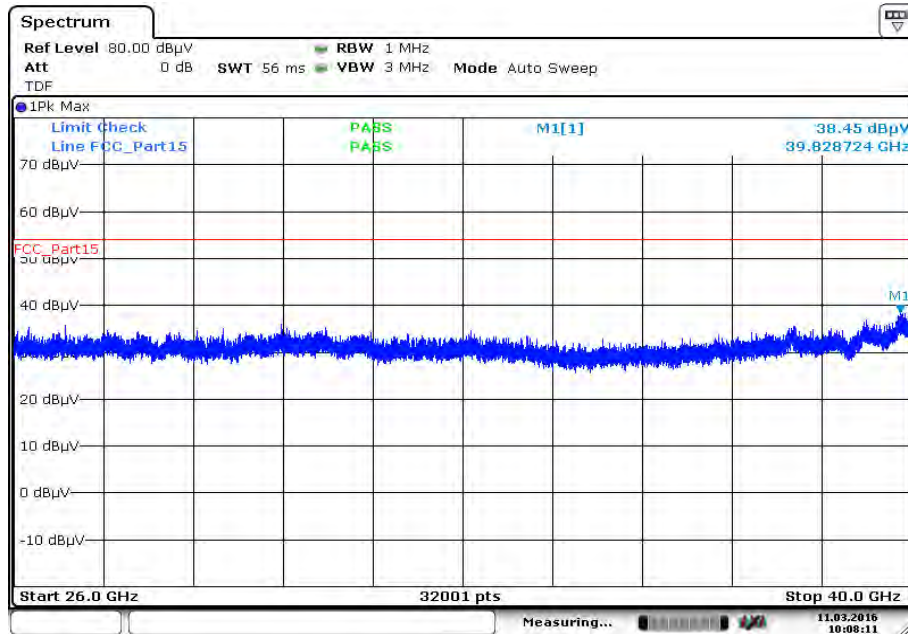
Plot 24: 26 GHz to 40 GHz, 5310 MHz, vertical & horizontal polarization
