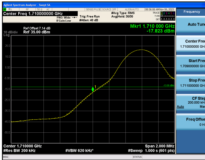
Band4-10MHz-16QAM-20000-1RB#49
