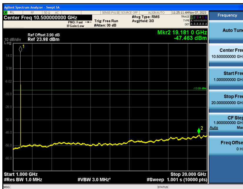
Band4-5MHz-QPSK-19975-1RB#0-Range1:30~1000MHz
