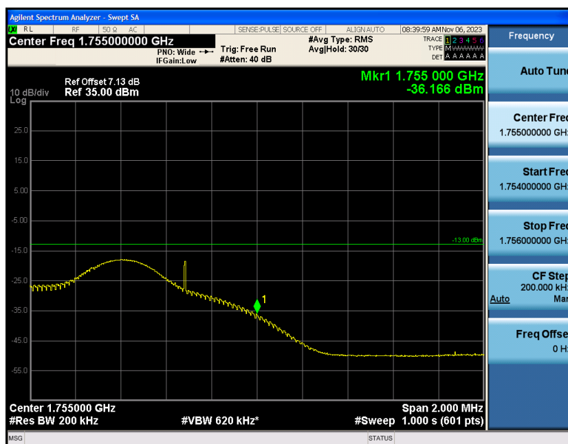
Band4-10MHz-16QAM-20350-1RB#49
