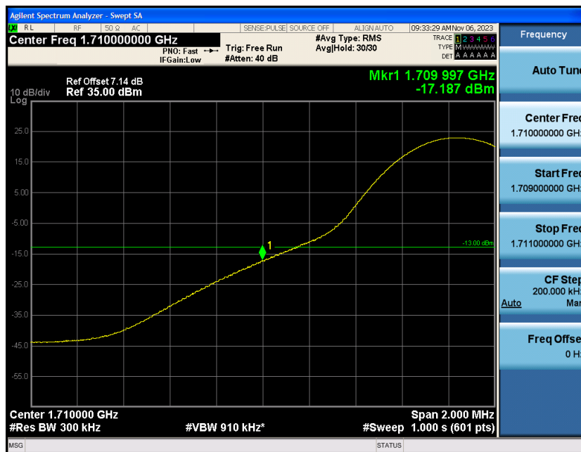
Band4-15MHz-QPSK-20025-1RB#74
