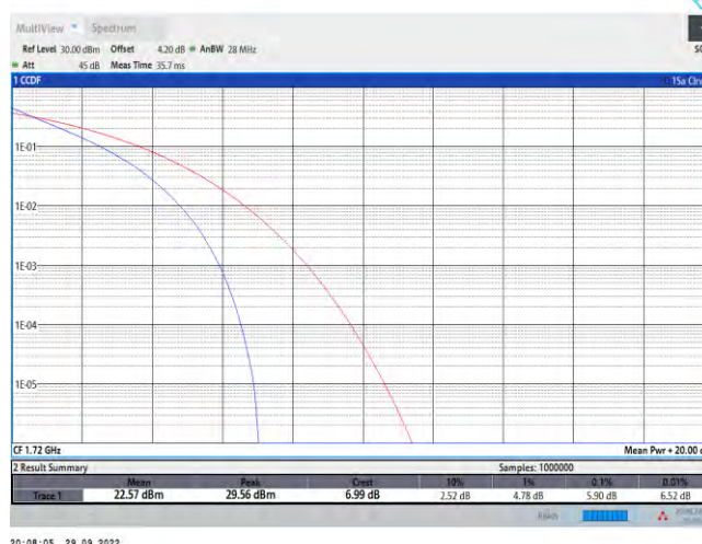
Band66-20MHz-QPSK-132322-100RB#0
