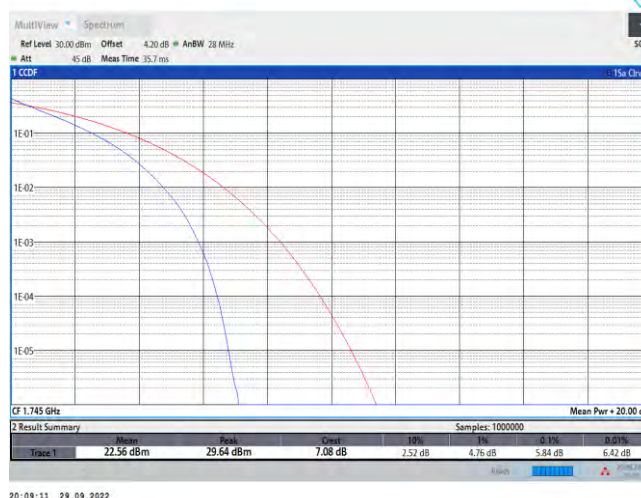
Band66-20MHz-QPSK-132322-100RB#0
