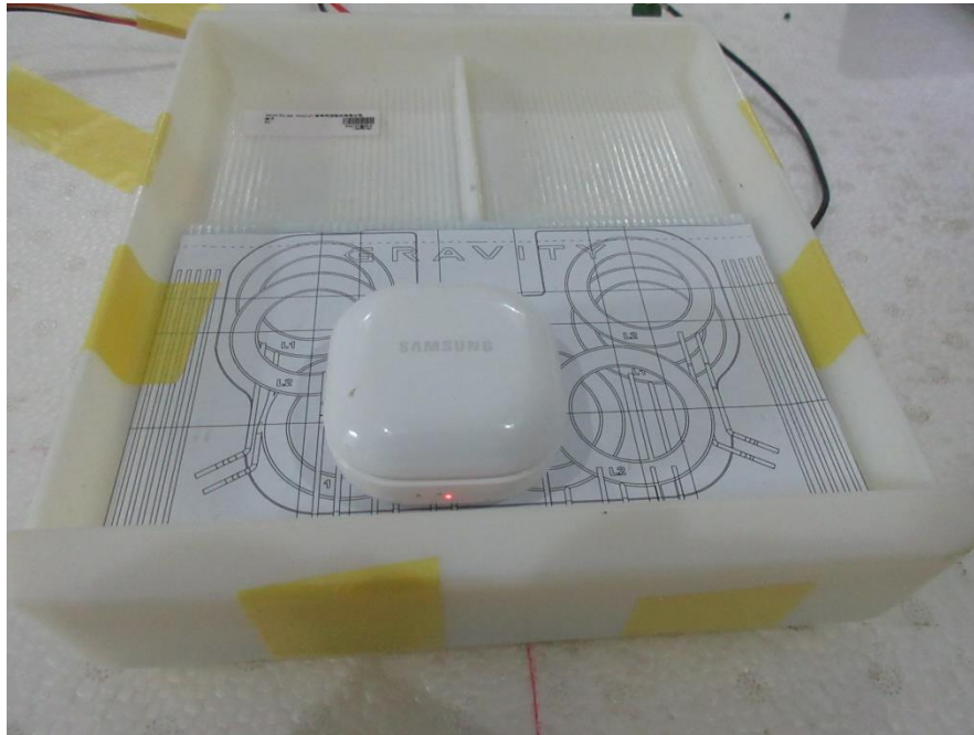
Operating Mode with charging case on Coil 5
