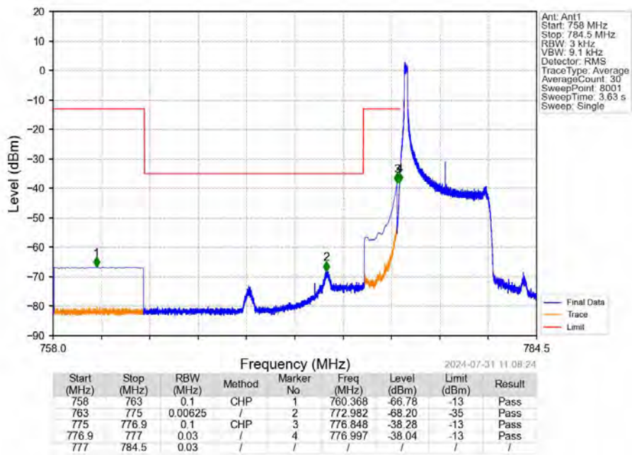
Band13_5MHz_16QAM_LCH_779.5MHz_RB_1_0_NTNV
