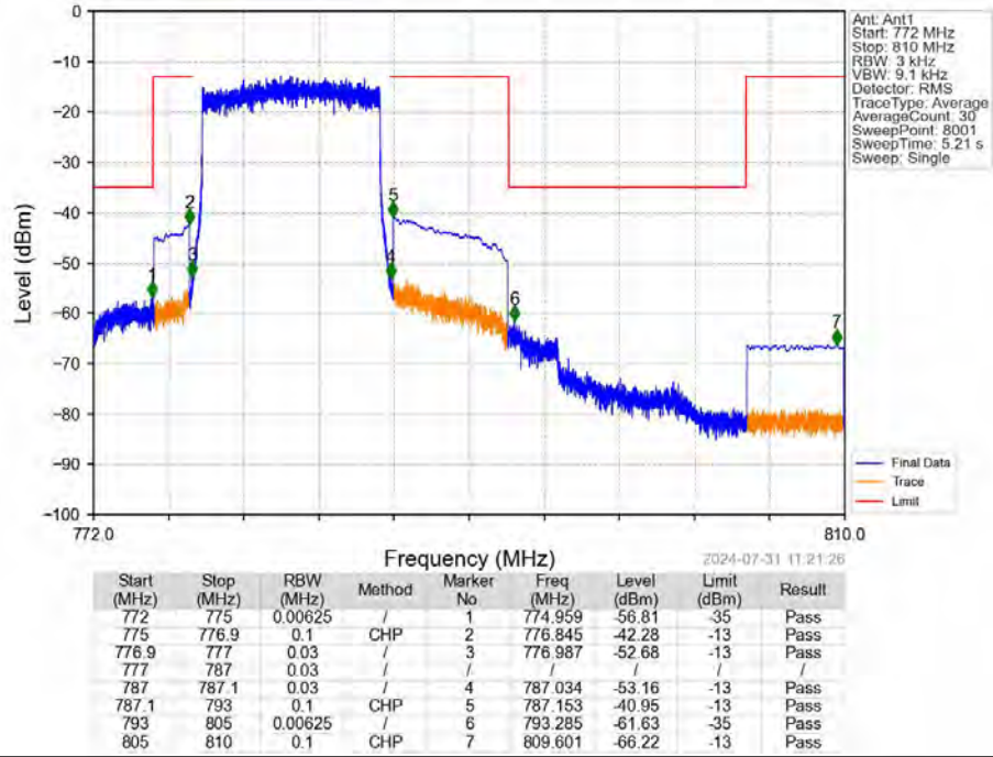
Band13_10MHz_16QAM_LCH_782MHz_RB_1_0_NTNV
