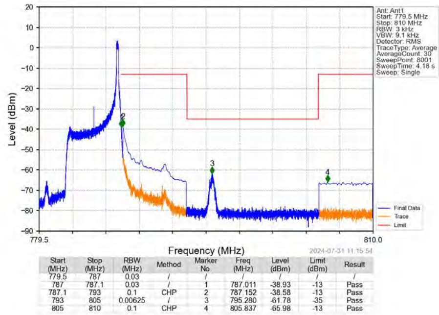
Band13_5MHz_16QAM_HCH_784.5MHz_RB_25_0_NTNV
