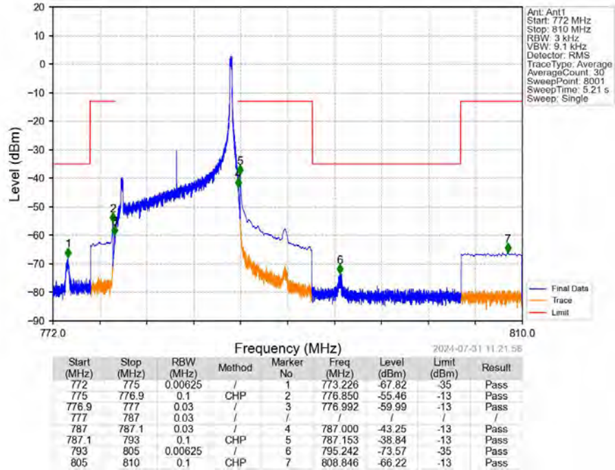
Band13_10MHz_16QAM_HCH_782MHz_RB_50_0_NTNV
