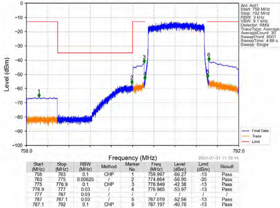
Band13_10MHz_QPSK_HCH_782MHz_RB_1_49_NTNV
