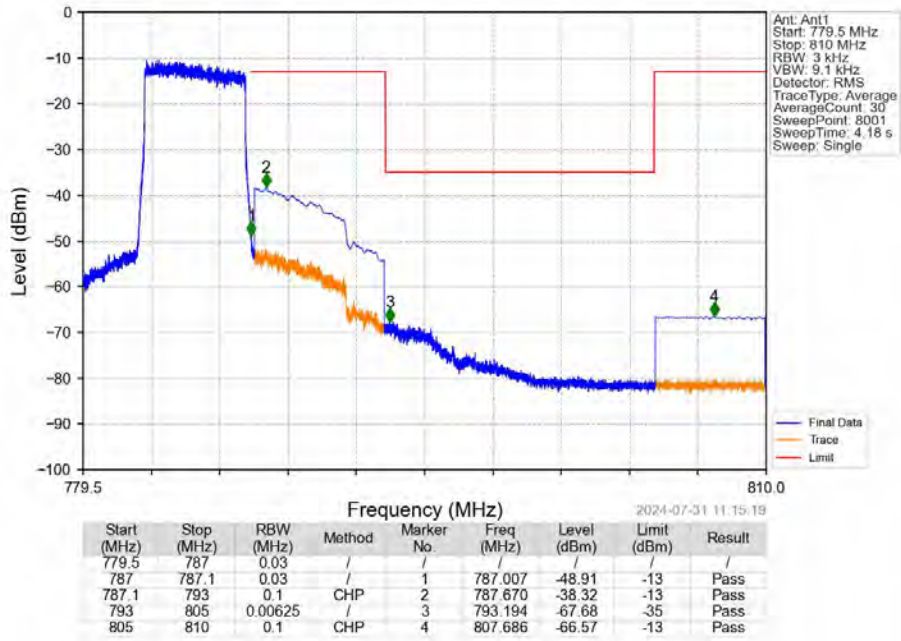
Band13_5MHz_16QAM_LCH_779.5MHz_RB_1_0_NTNV
