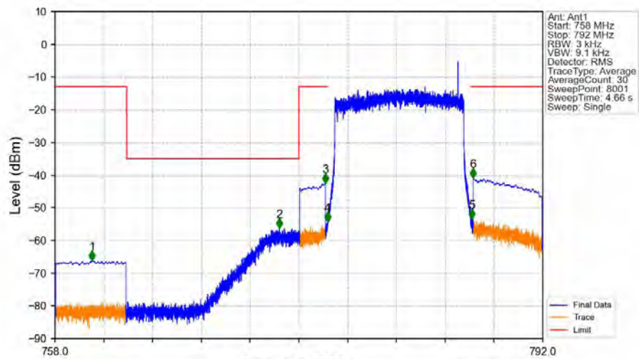
Band13_10MHz_16QAM_LCH_782MHz_RB_50_0_NTNV
