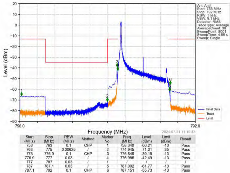
Band13_10MHz_16QAM_LCH_782MHz_RB_1_0_NTNV
