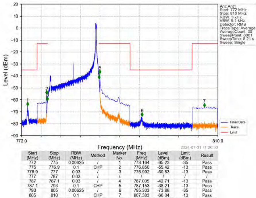
Band13_10MHz_QPSK_HCH_782MHz_RB_1_49_NTNV
