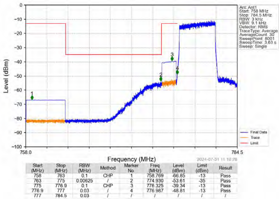
Band13_5MHz_16QAM_LCH_779.5MHz_RB_25_0_NTNV
