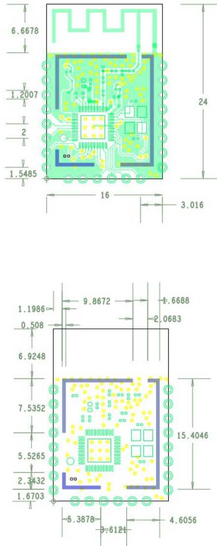
Figure 6-1WB3S-IPEX mechanical dimensions
