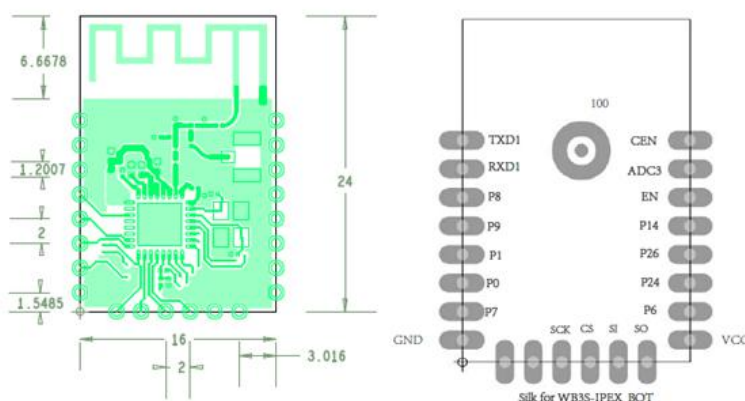
Figure 2-1 WB3S-IPEX front and rear views
