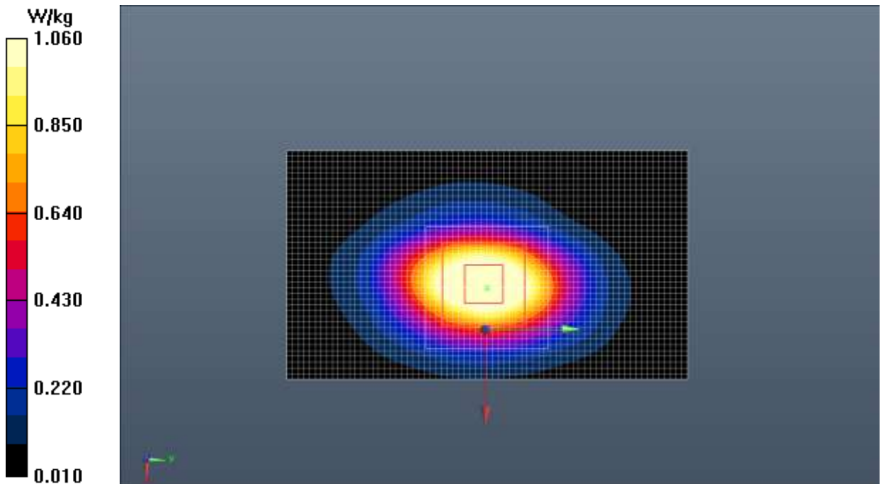
Fig.30 LTE Band 25
