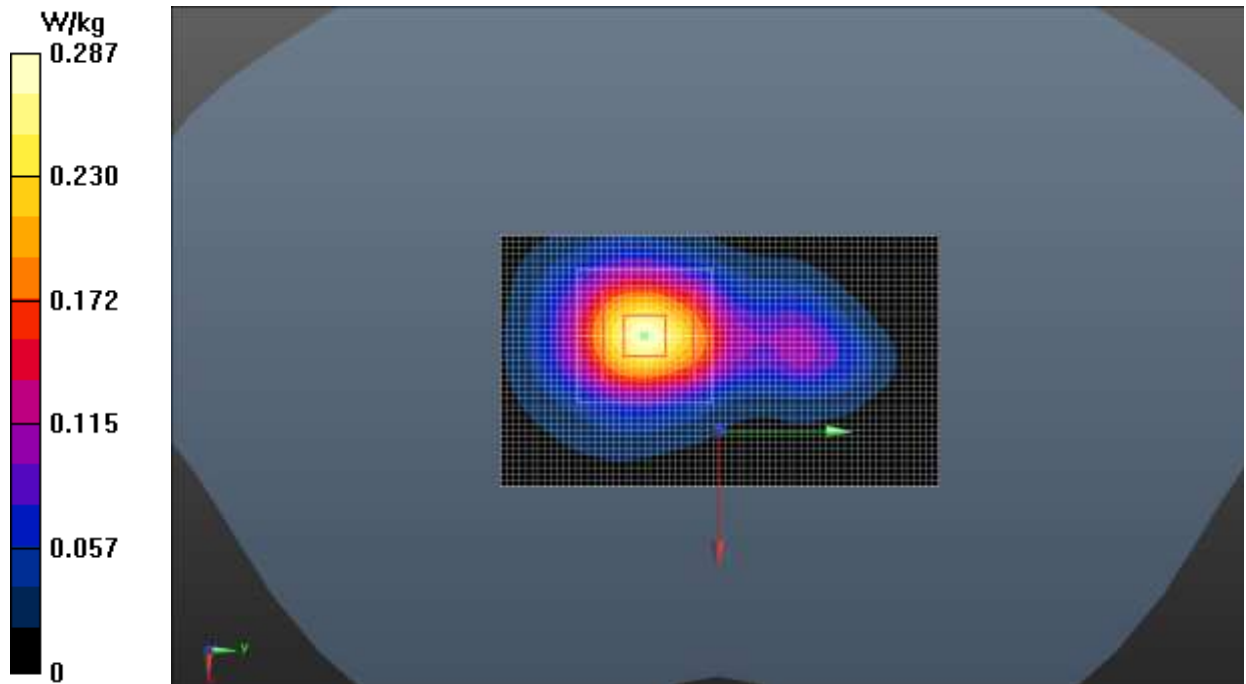
Fig.40 WLAN 2.4G
