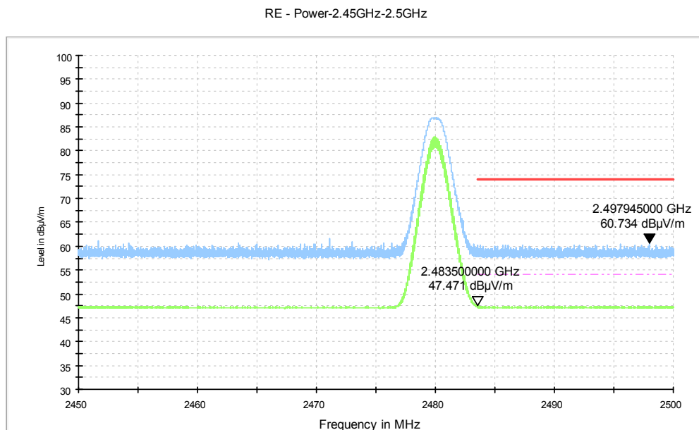
Fig.4. Frequency Band Edges: GFSK, Channel 39, 2.45GHz - 2.50GHz
