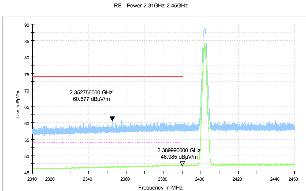
Fig.3. Frequency Band Edges: GFSK, Channel 0, 2.31GHz – 2.45GHz
