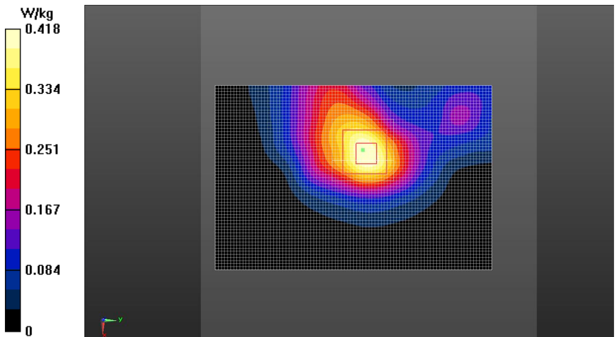
Fig.8 Wi-Fi 2.4G
