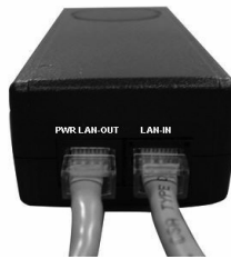
Figure 3-59 PoE Injector
