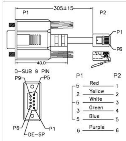
Figure 3-53 Serial Components
