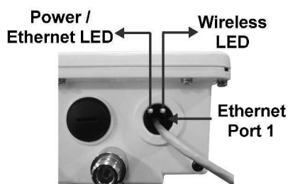
Figure 3-62 View LEDs
