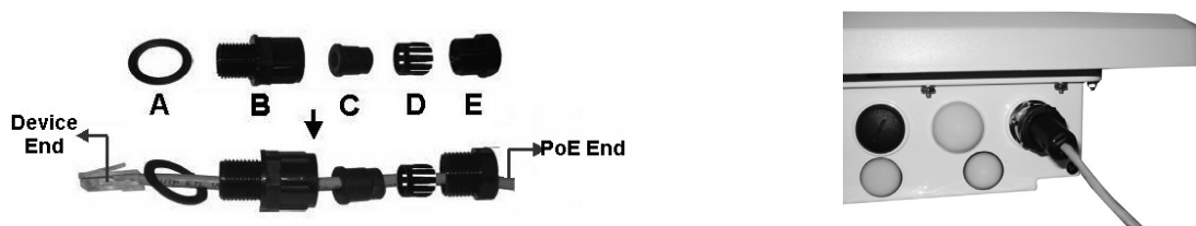
Figure 3-43 Weatherproofing RJ45 Connector
