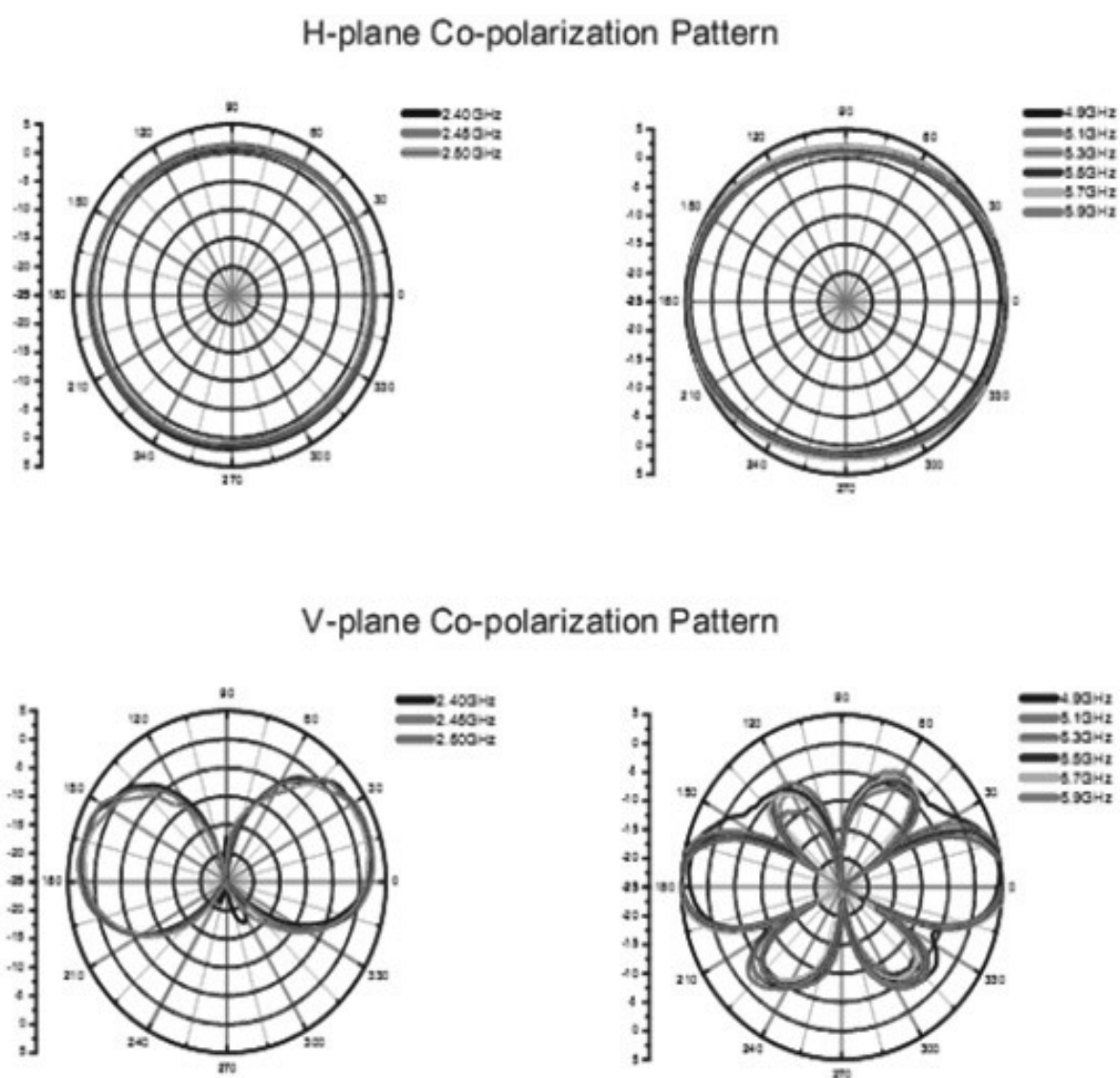
Figure 4-6 Radiation pattern for the Omni directional Antenna
