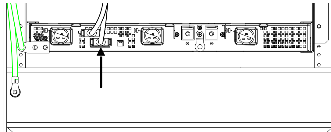
Figure 92: Alarm Cable
