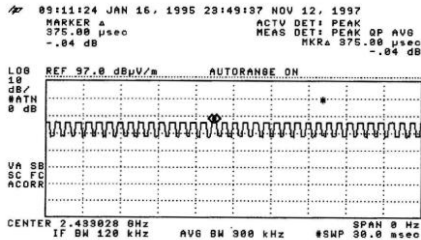
Figure C [Short Pulse]
