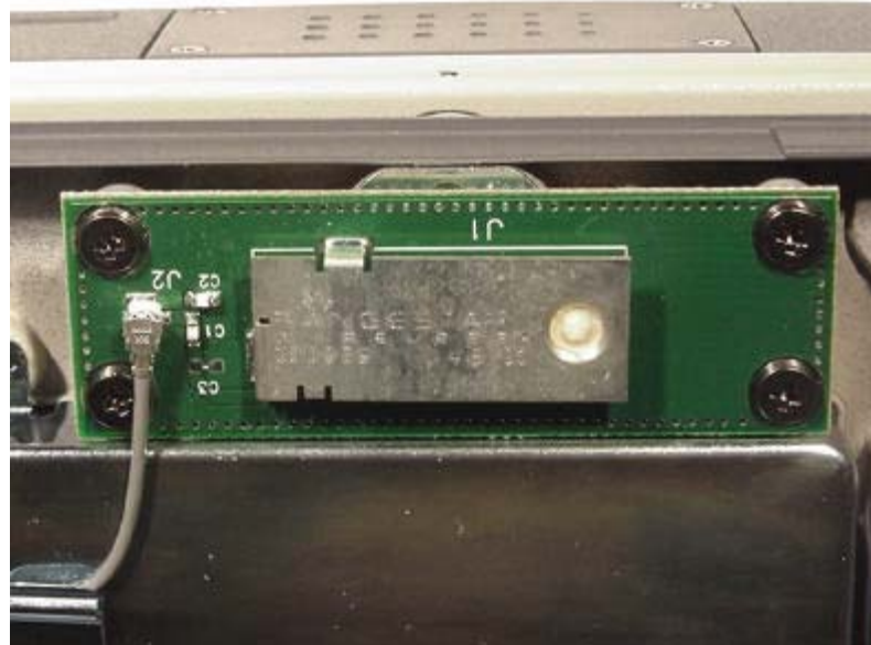
Back of LCD Display - Left-Side Antenna
