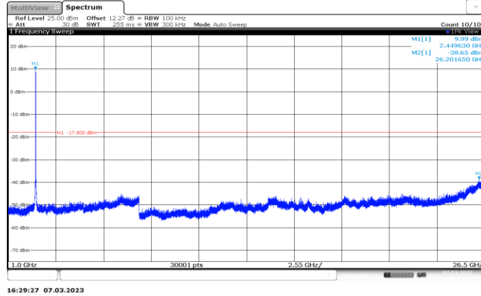
11G-CDD_Ant3_2457_1000~26500
