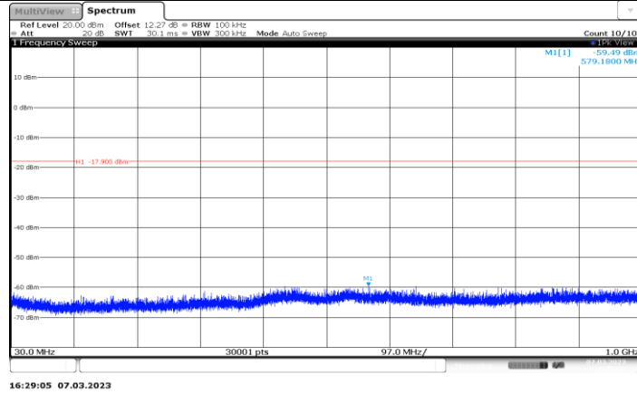
11G-CDD_Ant3_2457_30~1000
