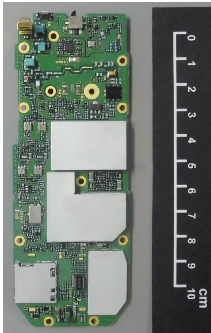
NX-5400-K2, K3, F2, F3 MAIN UNIT
