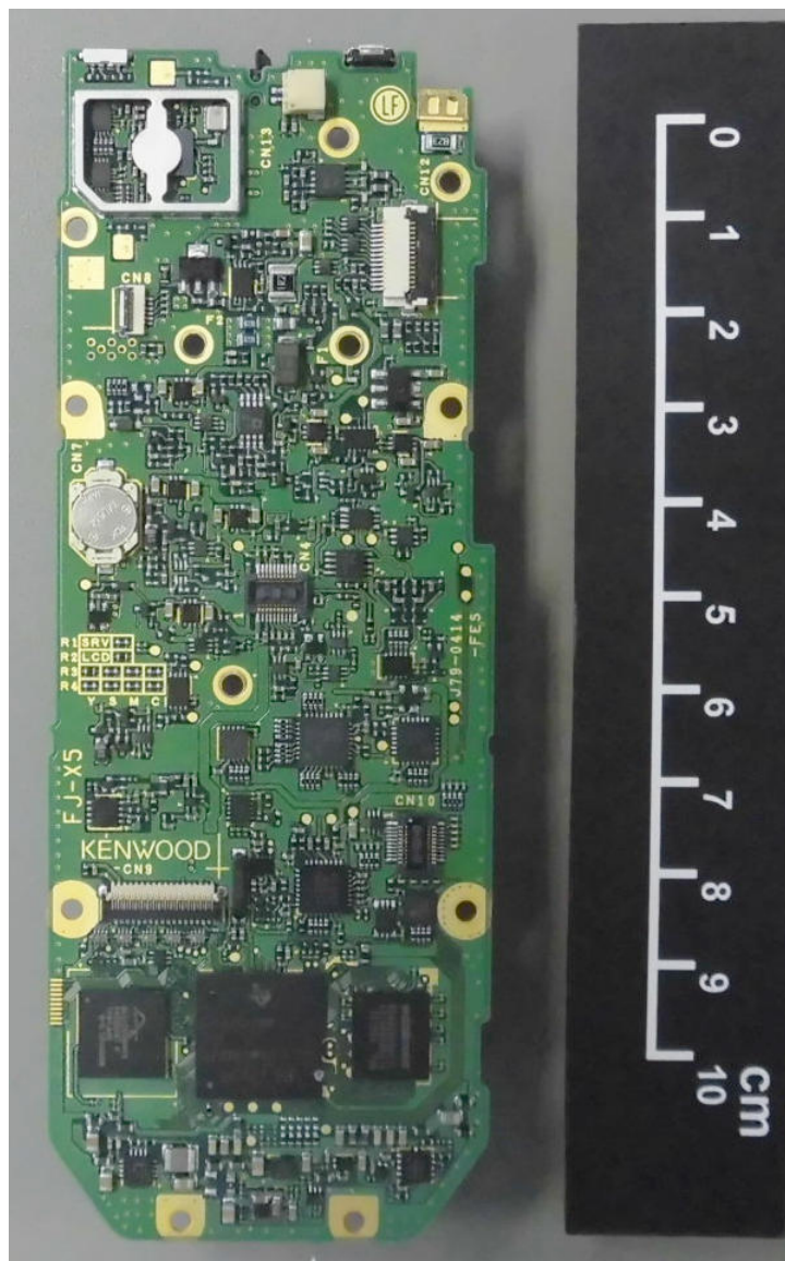
NX-5400-K2, K3, F2, F3 MAIN UNIT
