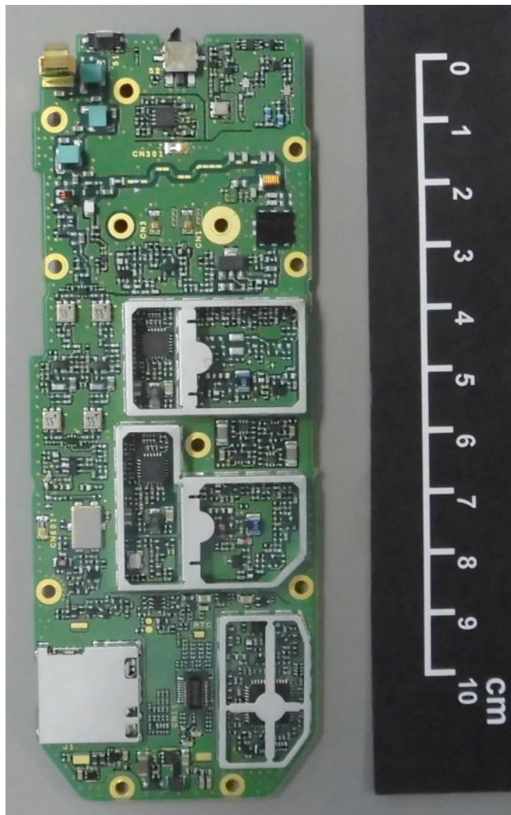
NX-5400-K2, K3, F2, F3 MAIN UNIT
