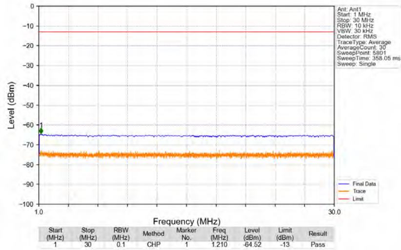
n5_15kHz_SISO_NTNV_5MHz_DFT-s-OFDM_PI/2_BPSK_846.5MHz_Edge_1RB_Right
