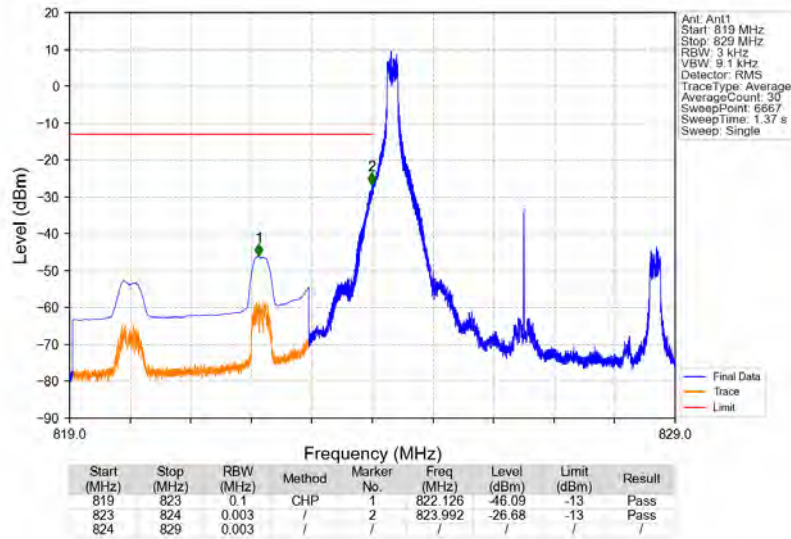
n5_15kHz_SISO_NTNV_5MHz_DFT-s-OFDM_QPSK_826.5MHz_Edge_1RB_Left
