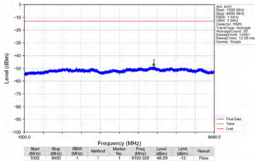
n5_15kHz_SISO_NTNV_5MHz_DFT-s-OFDM_QPSK_836.5MHz_Edge_1RB_Left
