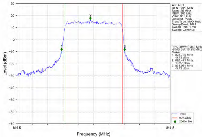
n5_15kHz_SISO_NTNV_10MHz_CP-OFDM_64 QAM_829MHz_Outer_Full
