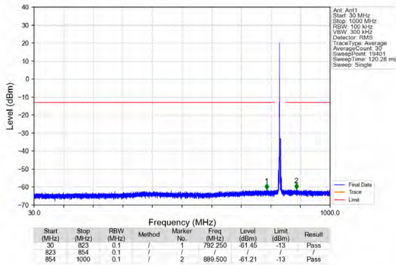
n5_15kHz_SISO_NTNV_5MHz_DFT-s-OFDM_PI/2_BPSK_836.5MHz_Edge_1RB_Left
