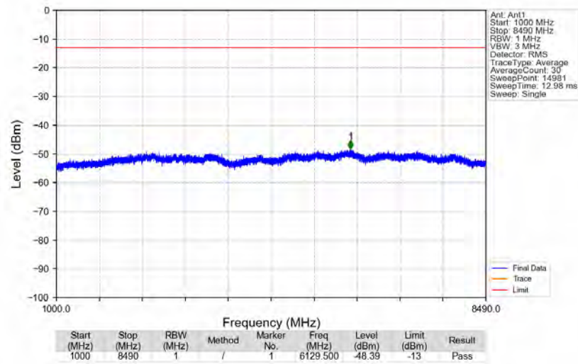
n5_15kHz_SISO_NTNV_5MHz_DFT-s-OFDM_PI/2_BPSK_846.5MHz_Edge_1RB_Right
