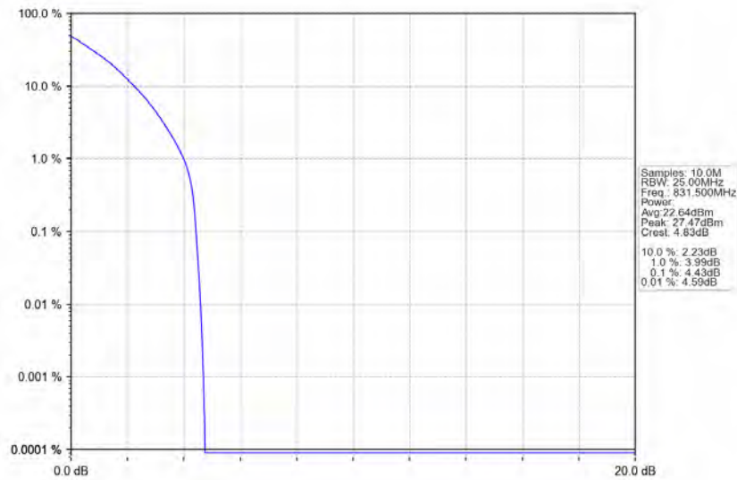
n5_15kHz_SISO_NTNV_15MHz_DFT-s-OFDM QPSK_831.5MHz_Outer_Full
