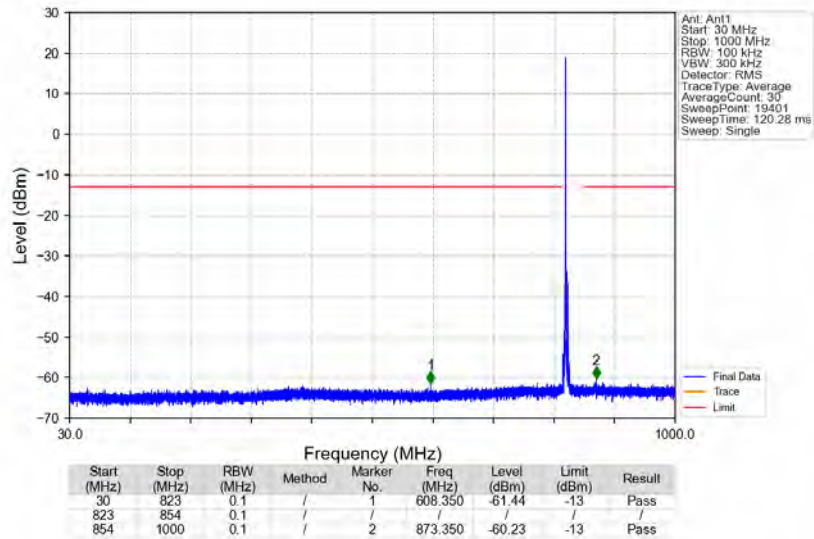
n5_15kHz_SISO_NTNV_5MHz_CP-OFDM_QPSK_826.5MHz_Edge_1RB_Left
