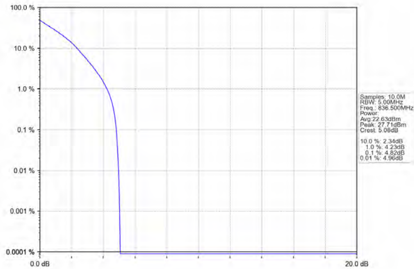
n5_15kHz_SISO_NTNV_5MHz_DFT-s-OFDM_QPSK_836.5MHz_Outer_Full
