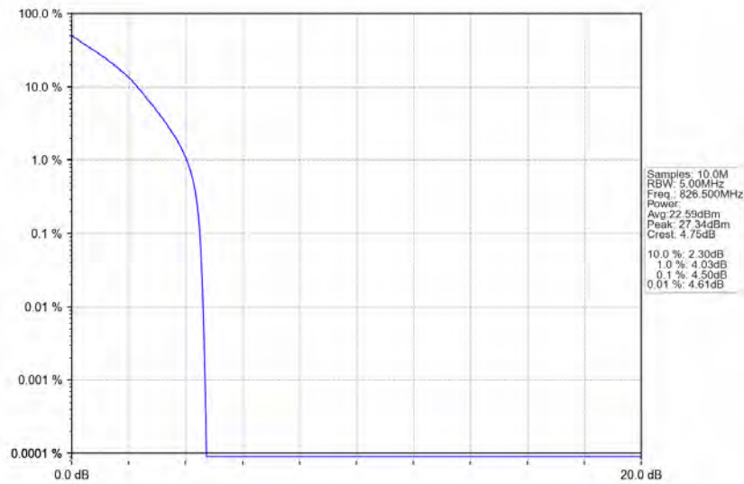
n5_15kHz_SISO_NTNV_5MHz_DFT-s-OFDM_QPSK_826.5MHz_Outer_Full
