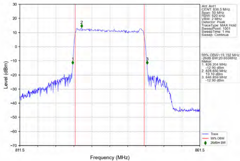
n5_15kHz_SISO_NTNV_20MHz_CP-OFDM_256_QAM_836.5MHz_Outer_Full
