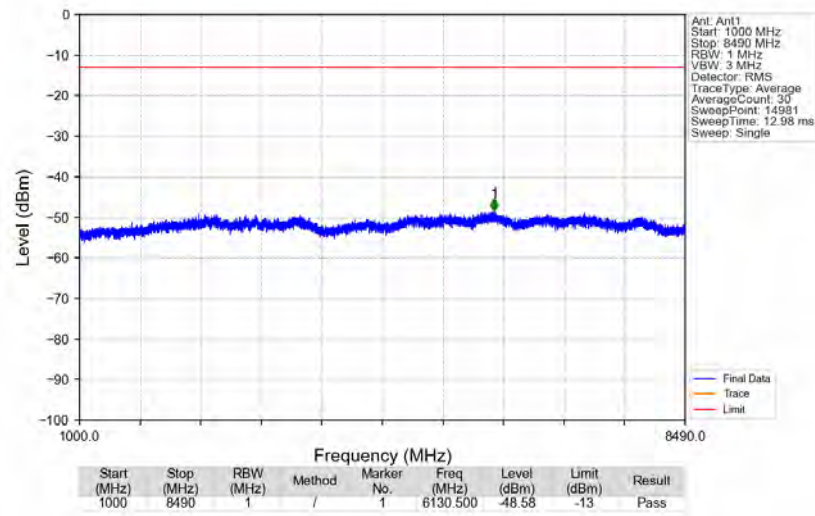
n5_15kHz_SISO_NTNV_5MHz_DFT-s-OFDM_QPSK_826.5MHz_Edge_1RB_Left
