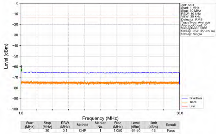
n5_15kHz_SISO_NTNV_5MHz_CP-OFDM_QPSK_826.5MHz_Edge_1RB_Left
