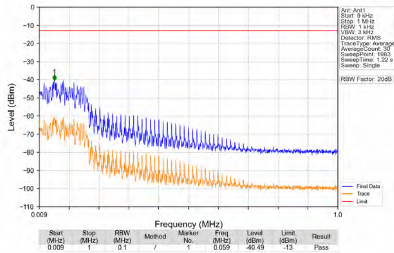
n5_15kHz_SISO_NTNV_5MHz_DFT-s-OFDM_QPSK_836.5MHz_Edge_1RB_Left
