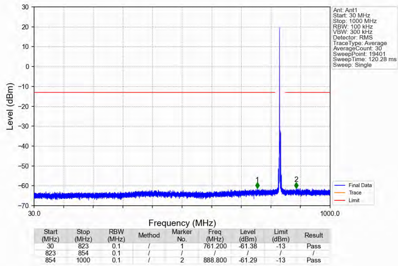
n5_15kHz_SISO_NTNV_5MHz_DFT-s-OFDM_QPSK_836.5MHz_Edge_1RB_Left
