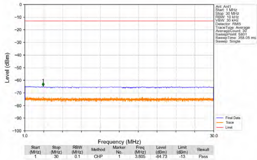
n5_15kHz_SISO_NTNV_5MHz_DFT-s-OFDM_QPSK_826.5MHz_Edge_1RB_Left
