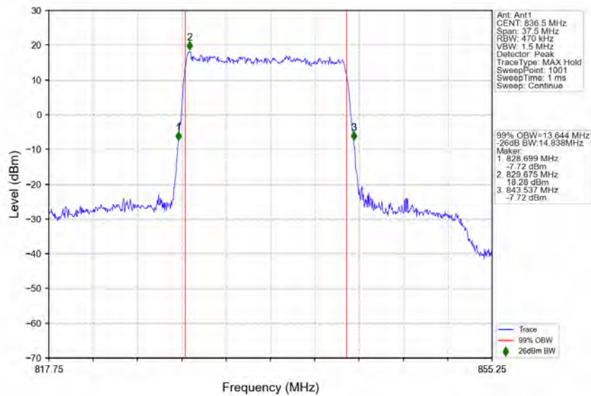
n5_15kHz_SISO_NTNV_15MHz_DFT-s-OFDM_16_QAM_836.5MHz_Outer_Full
