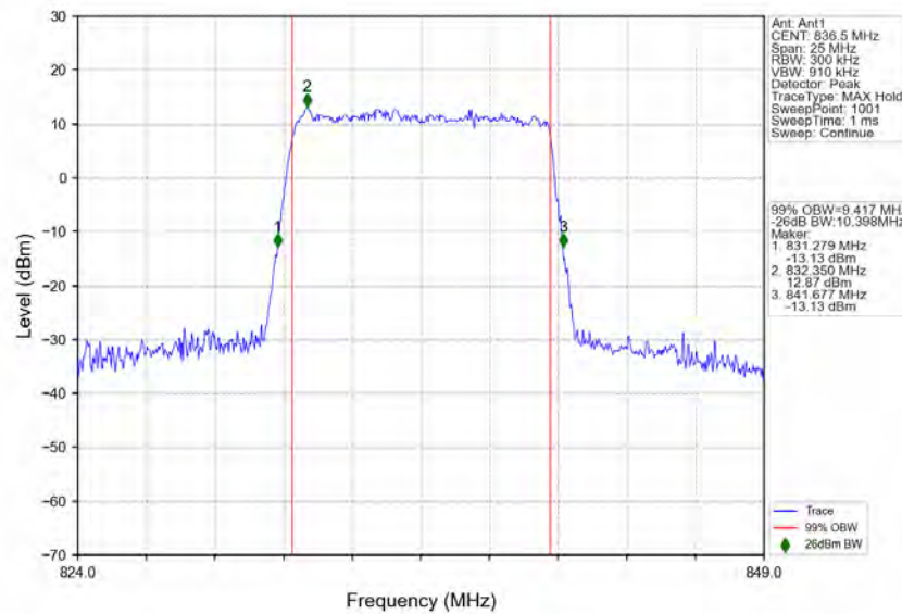
n5_15kHz_SISO_NTNV_10MHz_CP-OFDM_256_QAM_836.5MHz_Outer_Full
