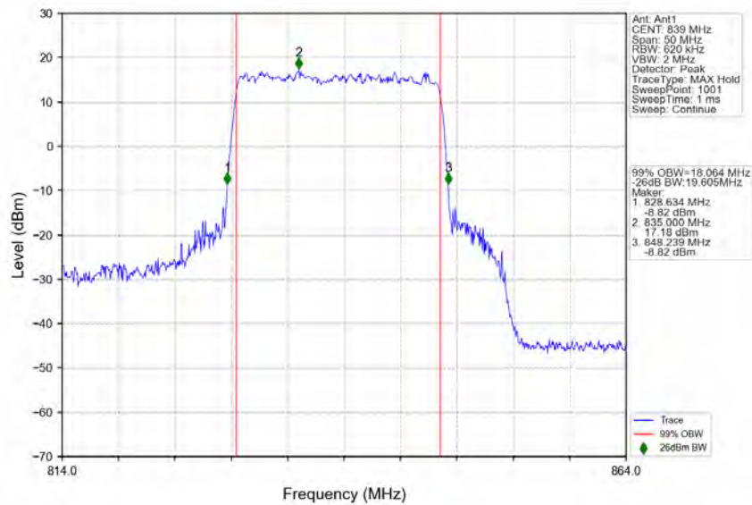
n5_15kHz_SISO_NTNV_20MHz_DFT-s-OFDM_64_QAM_839MHz_Outer_Full
