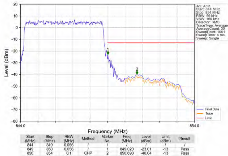
n5_15kHz_SISO_NTNV_5MHz_DFT-s-OFDM_PI/2_BPSK_846.5MHz_Outer_Full
