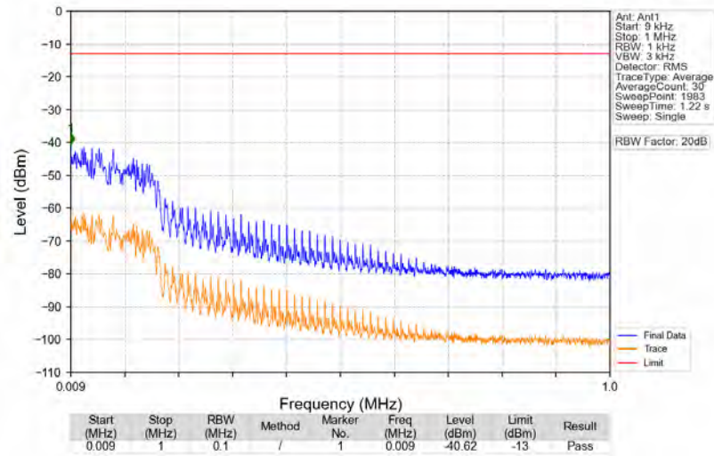
n5_15kHz_SISO_NTNV_5MHz_CP-OFDM_QPSK_836.5MHz_Edge_1RB_Left
