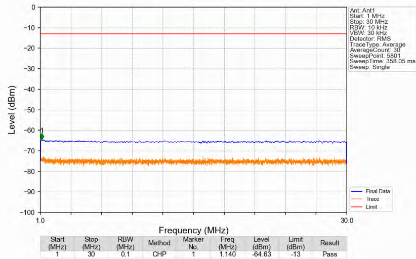
n5_15kHz_SISO_NTNV_5MHz_DFT-s-OFDM_PI/2_BPSK_836.5MHz_Edge_1RB_Left
