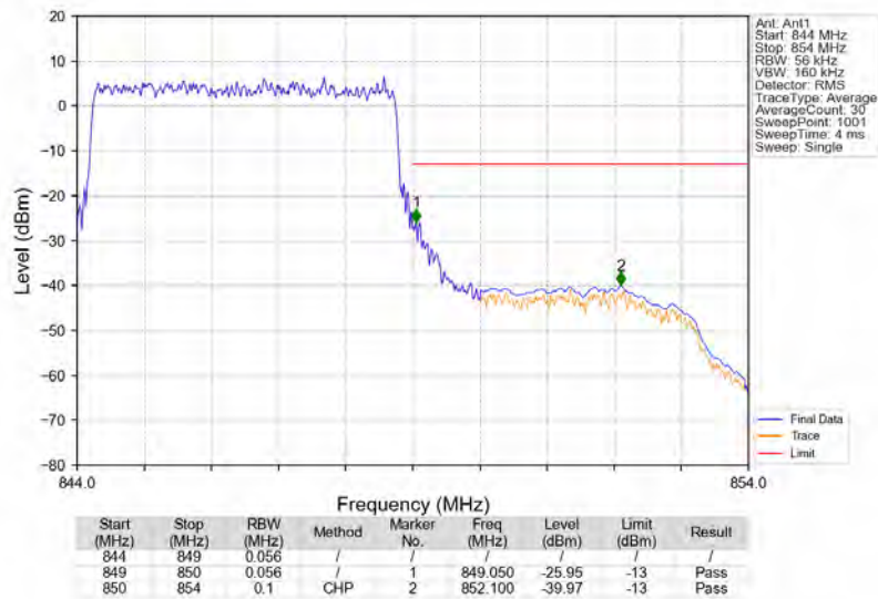
n5_15kHz_SISO_NTNV_5MHz_DFT-s-OFDM_QPSK_846.5MHz_Outer_Full
