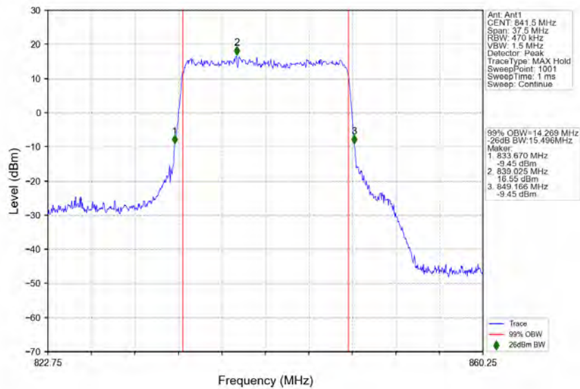
n5_15kHz_SISO_NTNV_15MHz_CP-OFDM_QPSK_841.5MHz_Outer_Full
