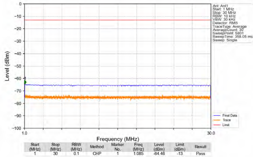
n5_15kHz_SISO_NTNV_5MHz_DFT-s-OFDM_QPSK_846.5MHz_Edge_1RB_Right
