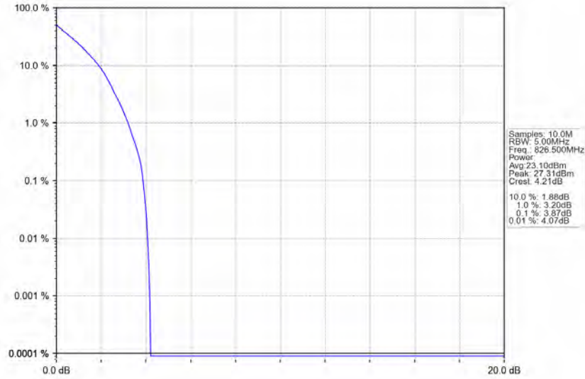
n5_15kHz_SISO_NTNV_5MHz_DFT-s-OFDM PI/2 BPSK_826.5MHz_Outer_Full
