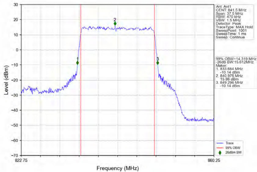
n5_15kHz_SISO_NTNV_15MHz_CP-OFDM_64_QAM_841.5MHz_Outer_Full
