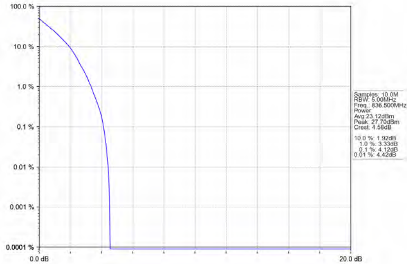
n5_15kHz_SISO_NTNV_5MHz_DFT-s-OFDM PI/2 BPSK_836.5MHz_Outer_Full
