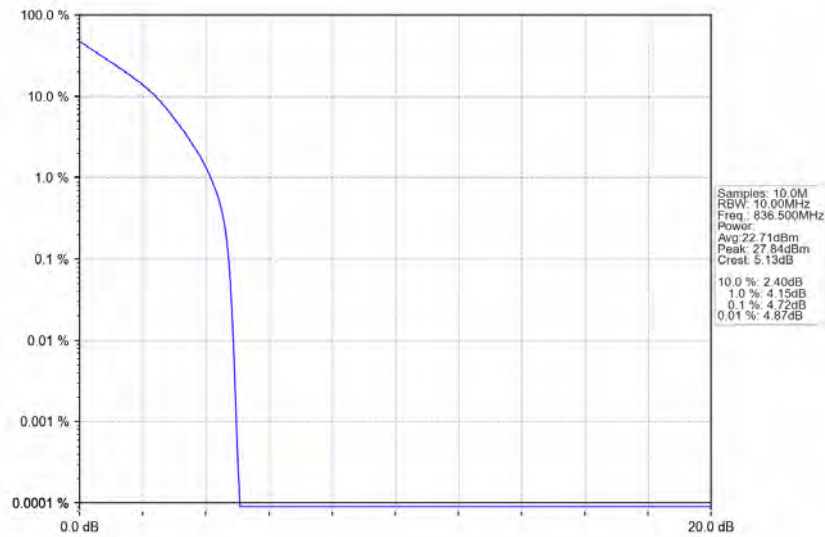
n5_15kHz_SISO_NTNV_10MHz_DFT-s-OFDM_QPSK_836.5MHz_Outer_Full
