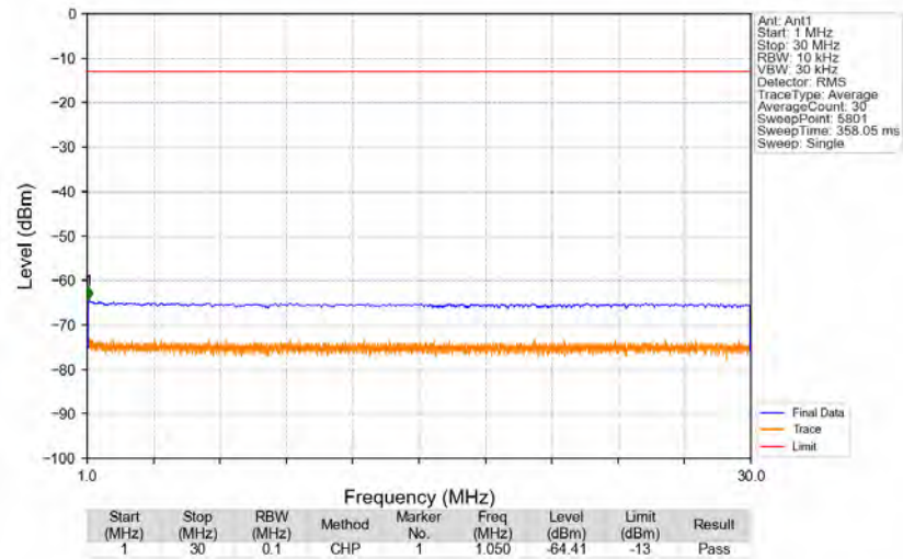
n5_15kHz_SISO_NTNV_5MHz_CP-OFDM_QPSK_836.5MHz_Edge_1RB_Left
