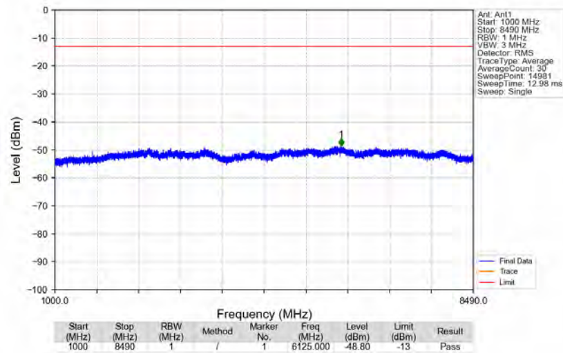
n5_15kHz_SISO_NTNV_5MHz_DFT-s-OFDM_PI/2_BPSK_836.5MHz_Edge_1RB_Left
