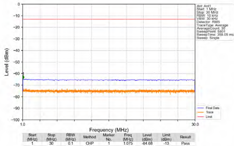
n5_15kHz_SISO_NTNV_5MHz_DFT-s-OFDM_QPSK_836.5MHz_Edge_1RB_Left
