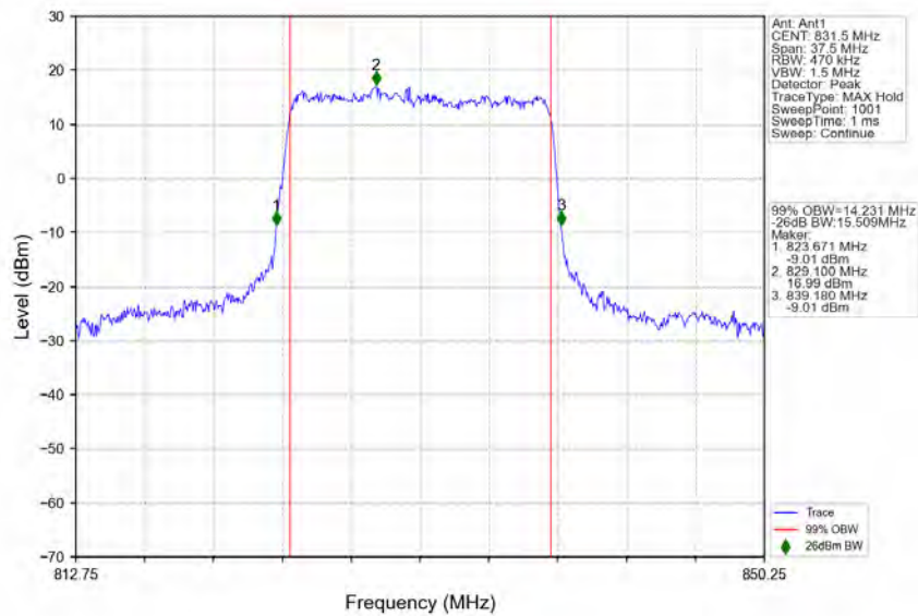
n5_15kHz_SISO_NTNV_15MHz_CP-OFDM_QPSK_831.5MHz_Outer_Full
