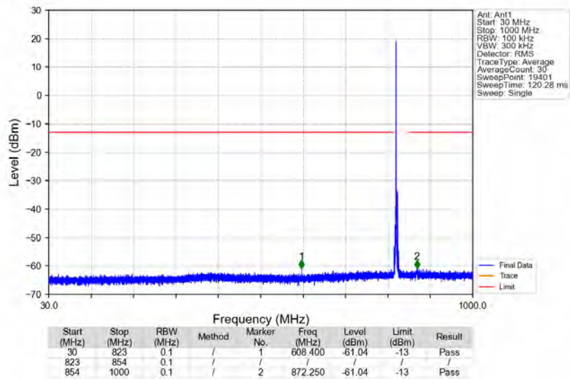
n5_15kHz_SISO_NTNV_5MHz_DFT-s-OFDM_QPSK_826.5MHz_Edge_1RB_Left
