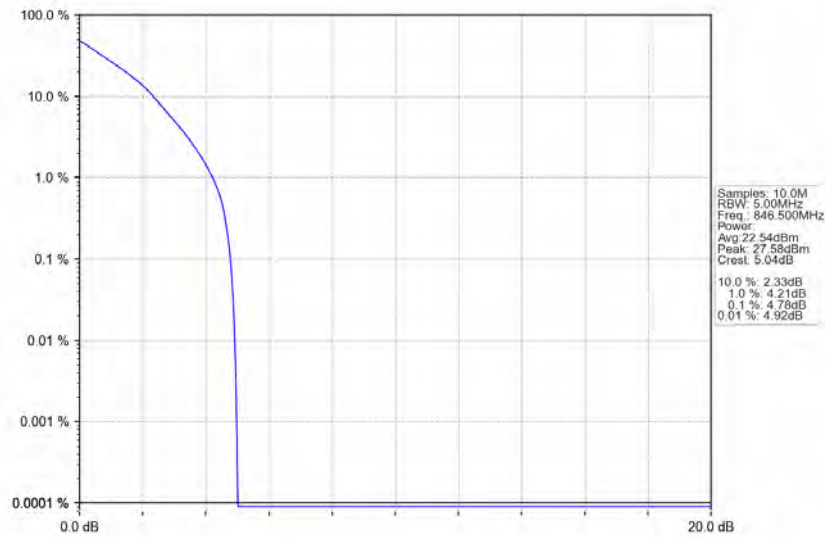
n5_15kHz_SISO_NTNV_5MHz_DFT-s-OFDM_QPSK_846.5MHz_Outer_Full
