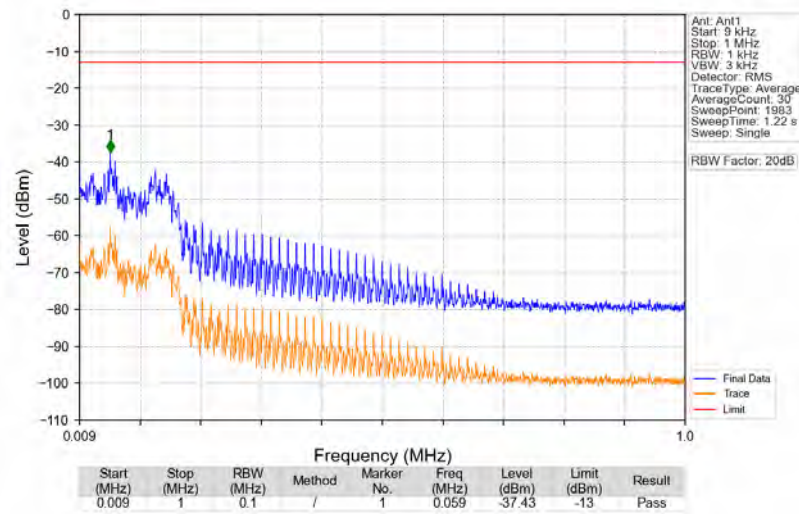
n5_15kHz_SISO_NTNV_5MHz_DFT-s-OFDM_PI/2_BPSK_836.5MHz_Edge_1RB_Left
