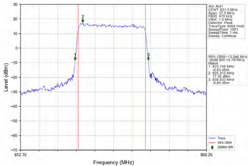
n5_15kHz_SISO_NTNV_15MHz_DFT-s-OFDM 64 QAM 831.5MHz_Outer_Full
