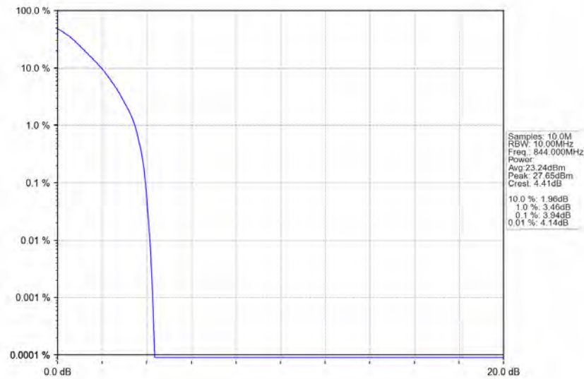
n5_15kHz_SISO_NTNV_10MHz_DFT-s-OFDM PI/2 BPSK_844MHz_Outer_Full
