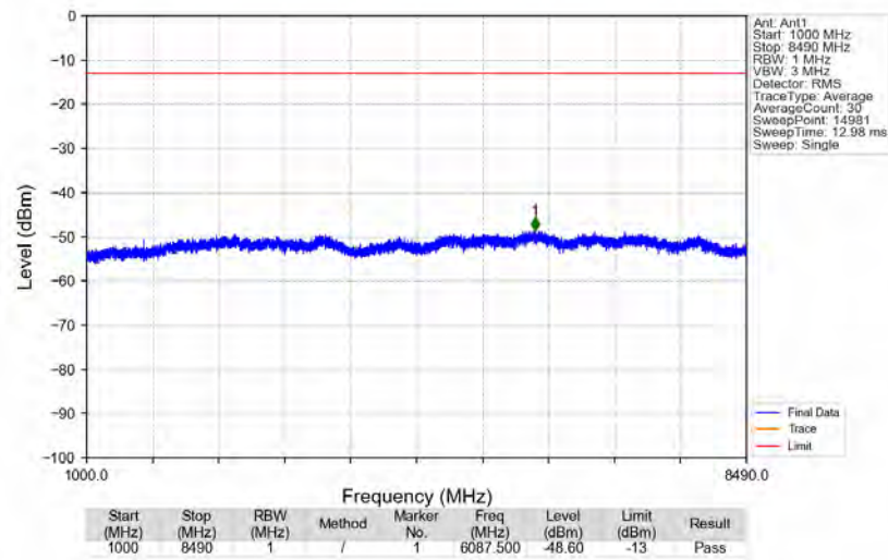
n5_15kHz_SISO_NTNV_5MHz_CP-OFDM_QPSK_826.5MHz_Edge_1RB_Left
