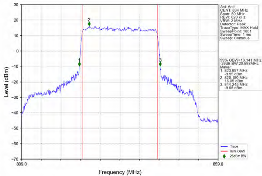
n5_15kHz_SISO_NTNV_20MHz_CP-OFDM_64_QAM_834MHz_Outer_Full
