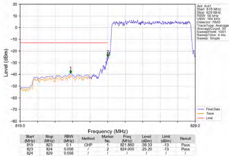
n5_15kHz_SISO_NTNV_5MHz_DFT-s-OFDM PI/2 BPSK_826.5MHz_Outer_Full
