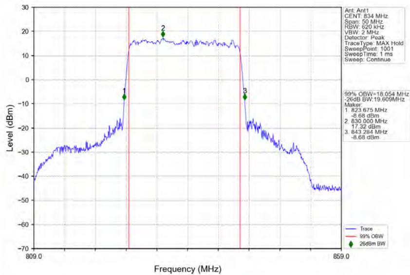
n5_15kHz_SISO_NTNV_20MHz_DFT-s-OFDM_64_QAM_834MHz_Outer_Full
