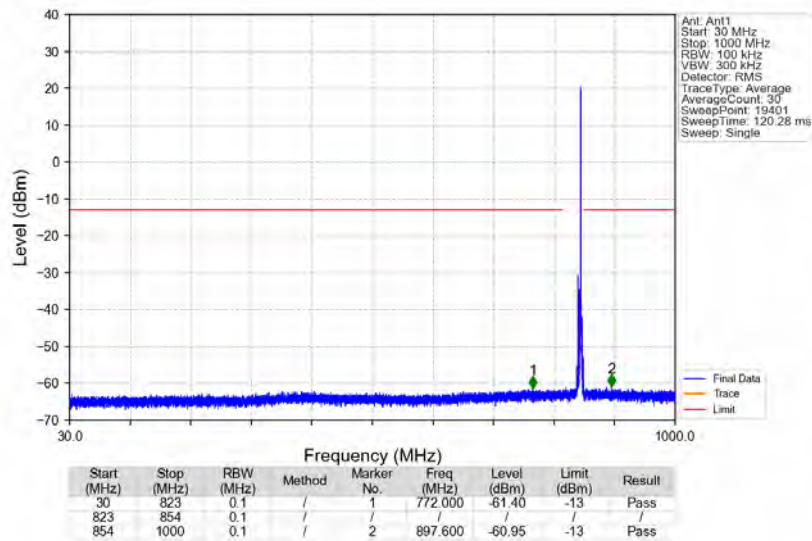
n5_15kHz_SISO_NTNV_5MHz_DFT-s-OFDM_PI/2_BPSK_846.5MHz_Edge_1RB_Right
