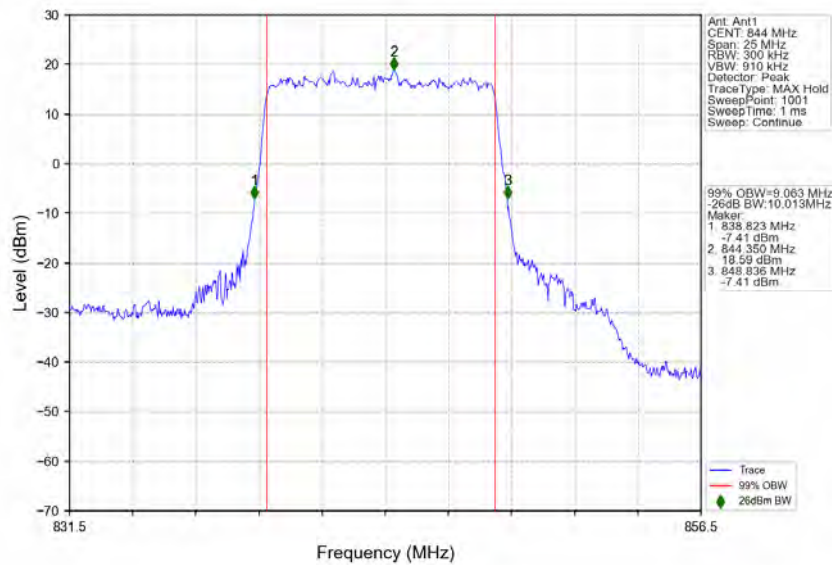
n5_15kHz_SISO_NTNV_10MHz_DFT-s-OFDM_QPSK_844MHz_Outer_Full
