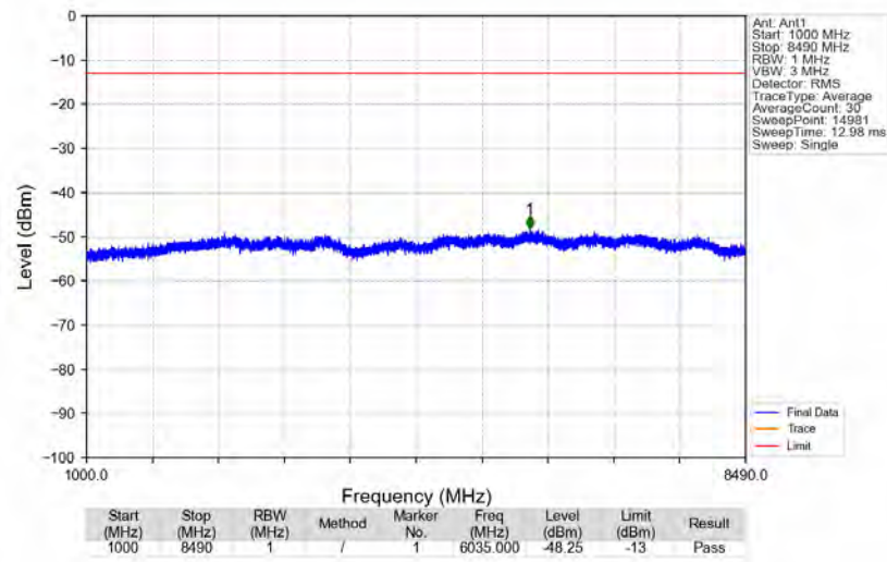
n5_15kHz_SISO_NTNV_5MHz_DFT-s-OFDM_QPSK_846.5MHz_Edge_1RB_Right
