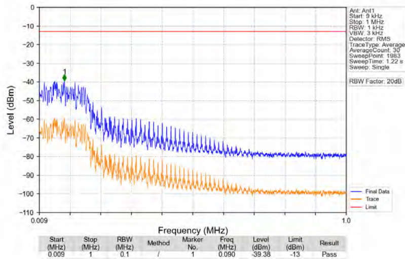
n5_15kHz_SISO_NTNV_5MHz_DFT-s-OFDM_QPSK_826.5MHz_Edge_1RB_Left
