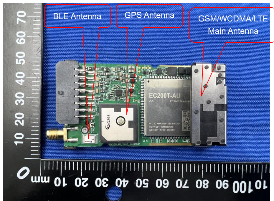
MAIN BOARD REAR VIEW (WITH SHIELDING)
