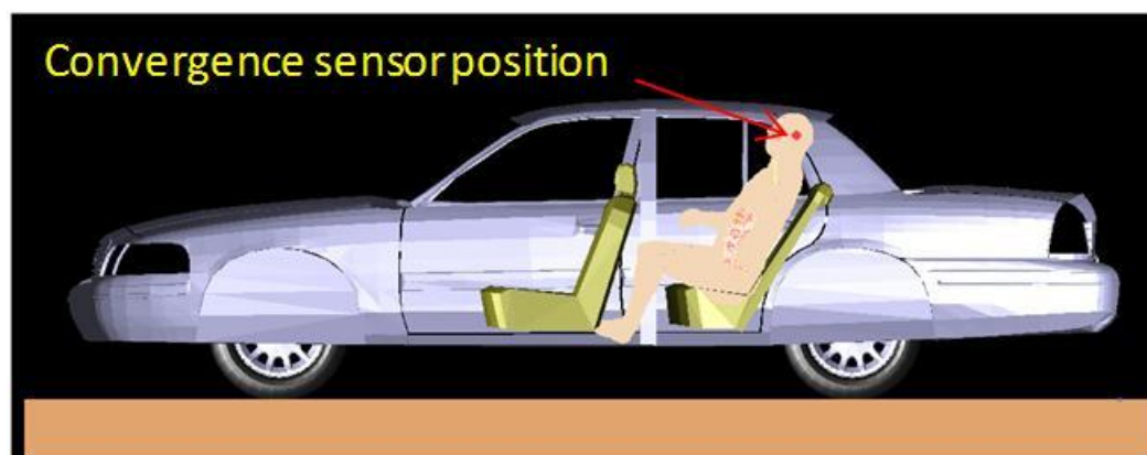
Locations for the E-field sensors placed in the passenger for the convergence analysis.
