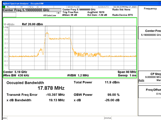
ANT L_802.11ax_HE40_26T_Low_UNII 1
