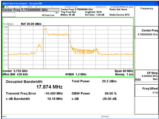
ANT L_802.11ax_HE40_26T_Low_UNII 3
