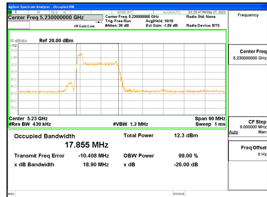
ANT R_802.11ax_HE40_26T_Low_UNII 1
