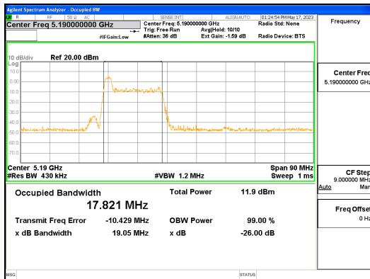
ANT R_802.11ax_HE40_26T_Low_UNII 1
