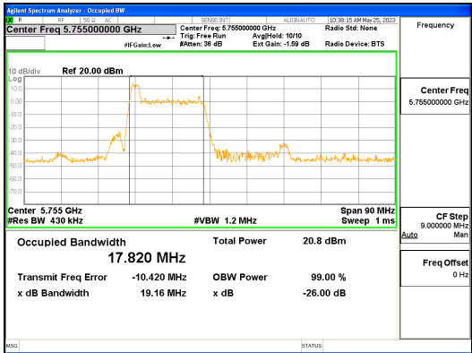
ANT R_802.11ax_HE40_26T_Low_UNII 3
