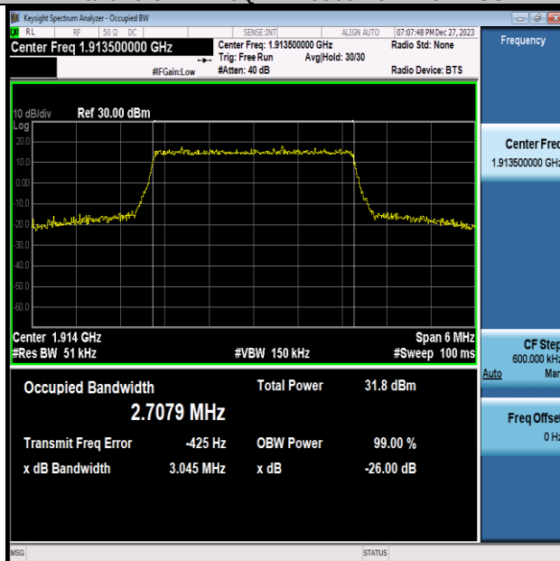
Band25-3MHz-16QAM-26675-15RB#0-PASS
