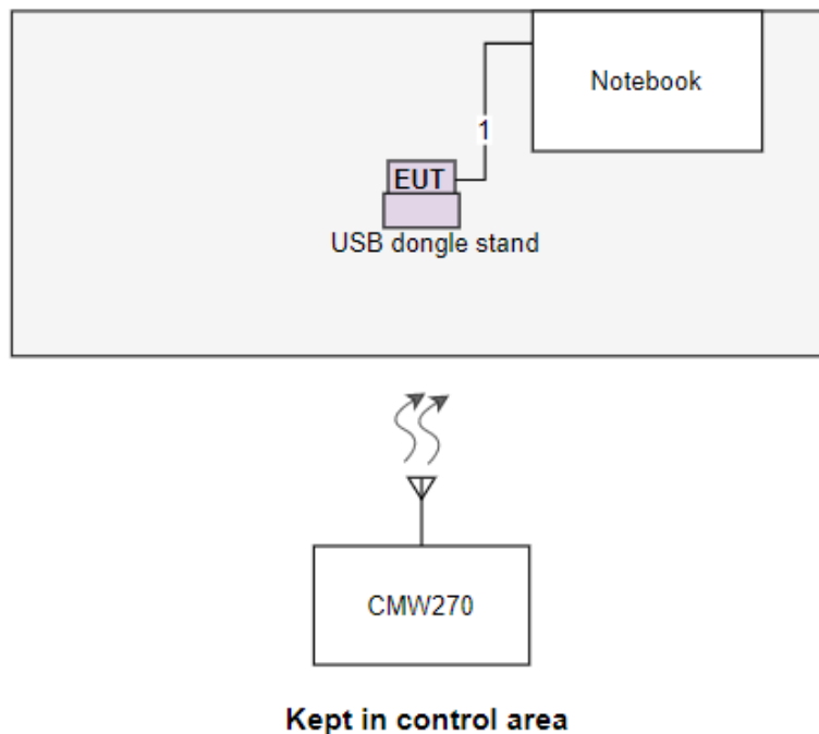
Test Setup Diagram (with USB dongle stand)
