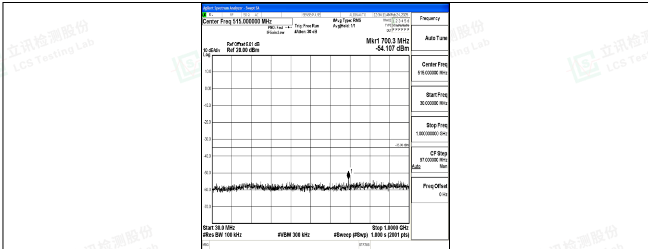
Band7_5MHz_QPSK_21100_1RB#0_30~1000_30~1000
