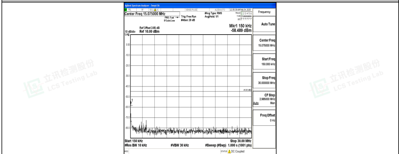
Band7_5MHz_16QAM_21425_1RB#0_0.15~30_0.15~30
