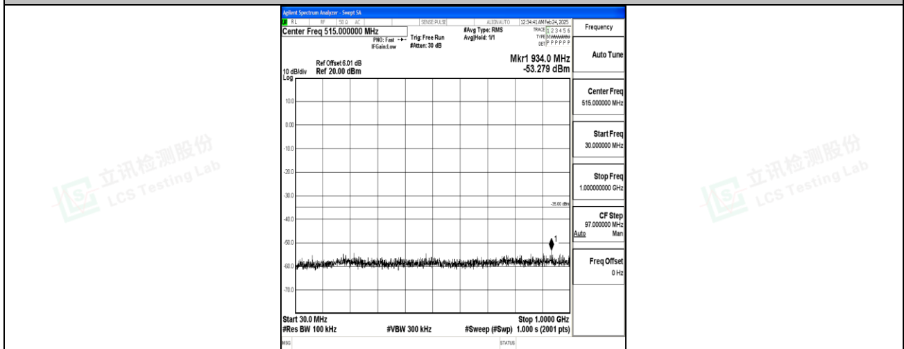
Band7_5MHz_16QAM_21100_1RB#0_30~1000_30~1000
