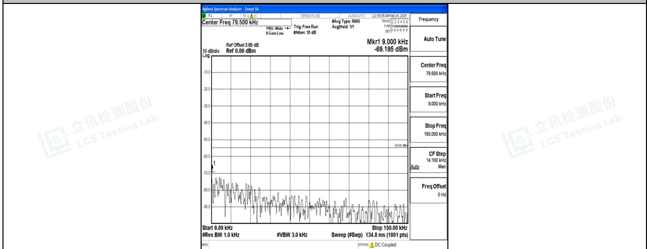
Band7_5MHz_QPSK_21425_1RB#0_0.009~0.15_0.009~0.15
