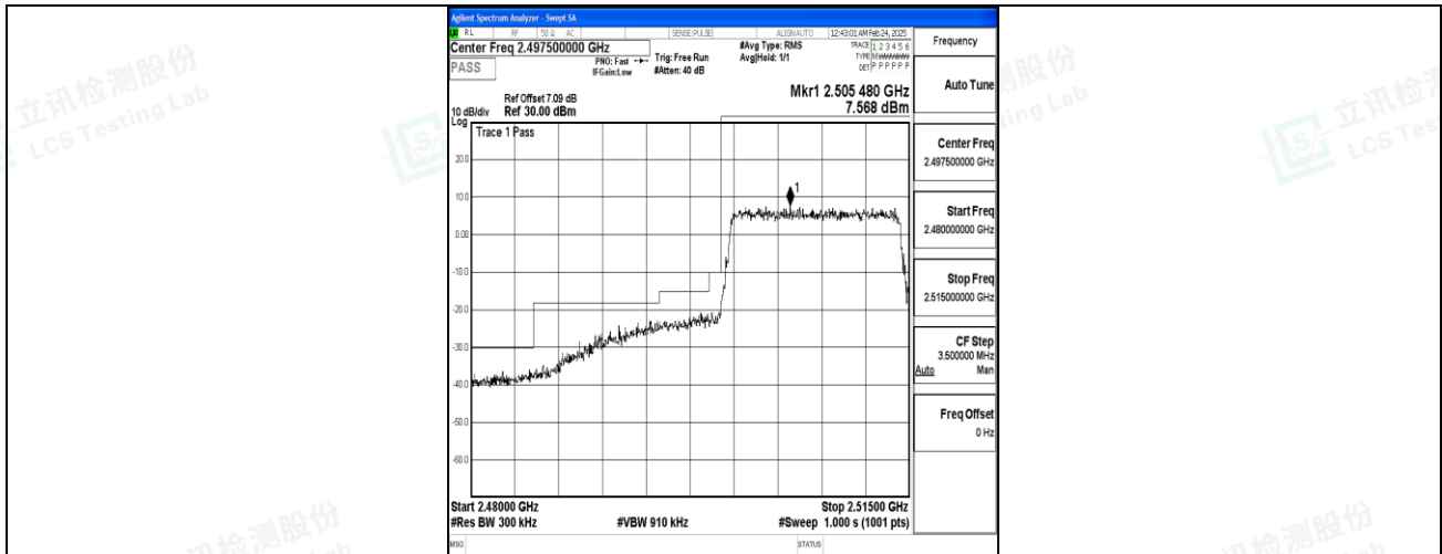
Band7_15MHz_QPSK_20825_75RB#0
