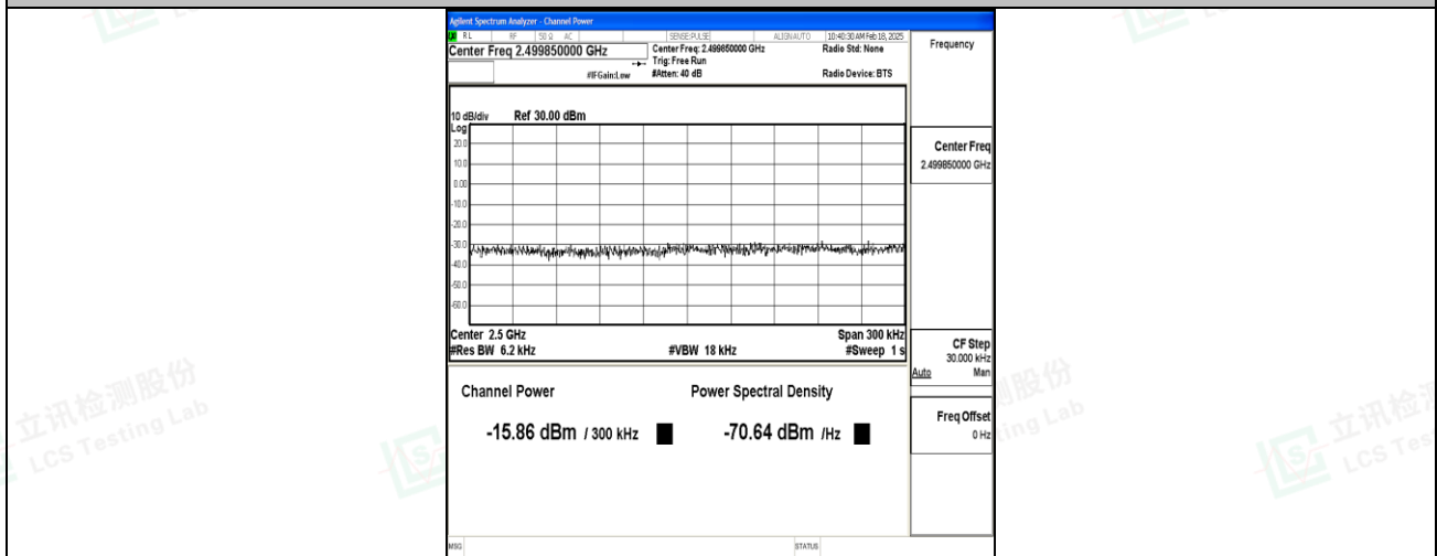
Band7_15MHz_QPSK_20825_75RB#0_Final4
