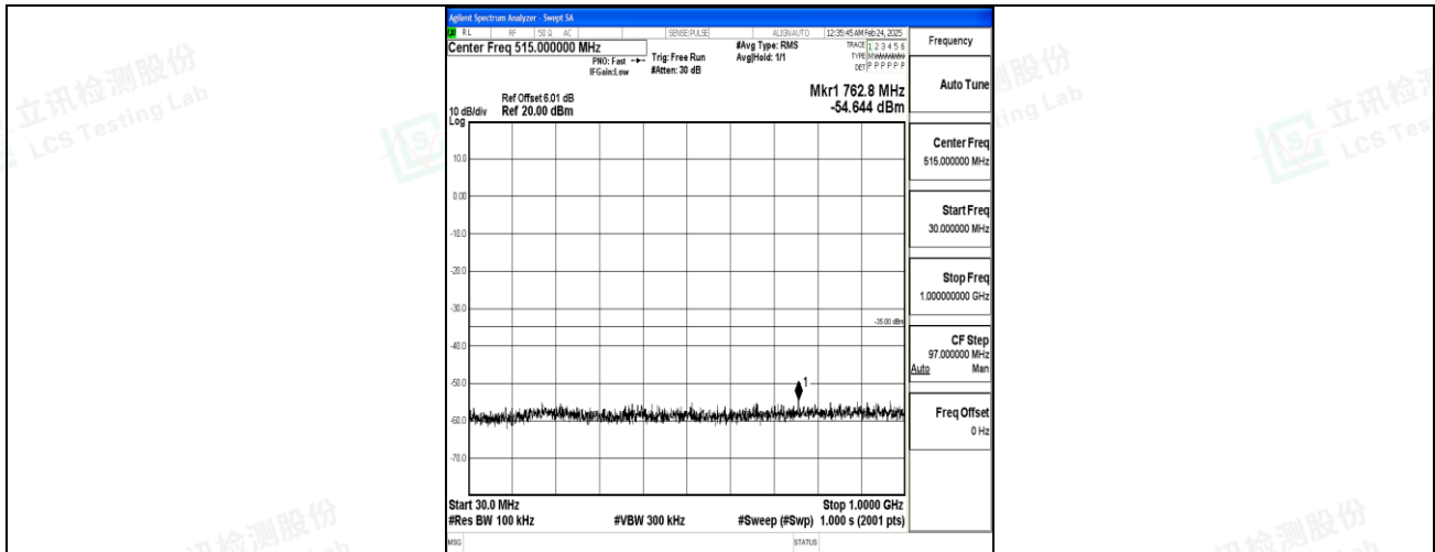
Band7_5MHz_16QAM_21425_1RB#0_30~1000_30~1000
