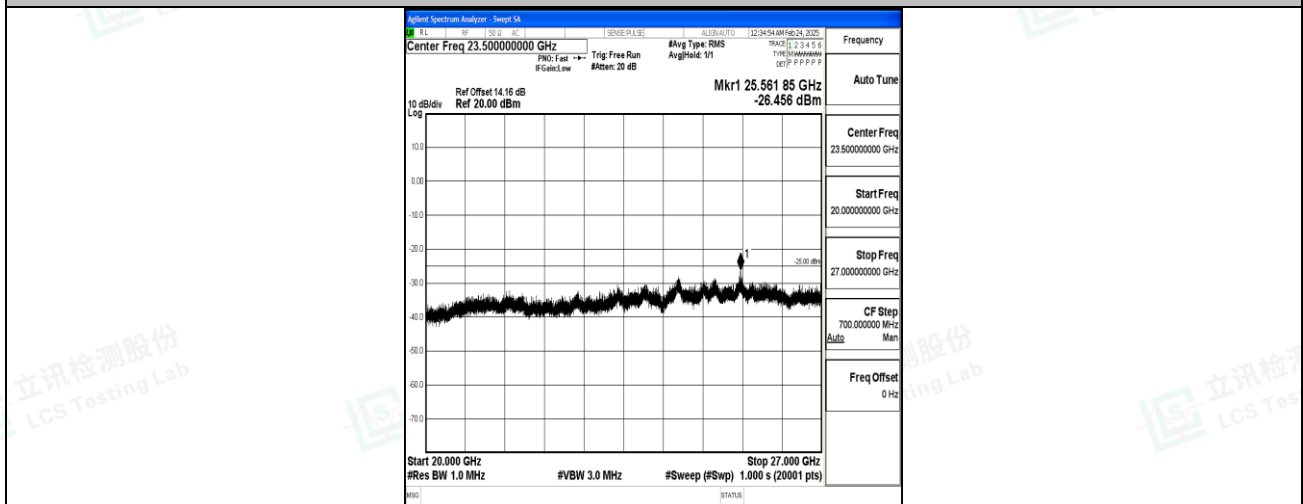
Band7_5MHz_16QAM_21100_1RB#0_20000~27000_20000~27000
