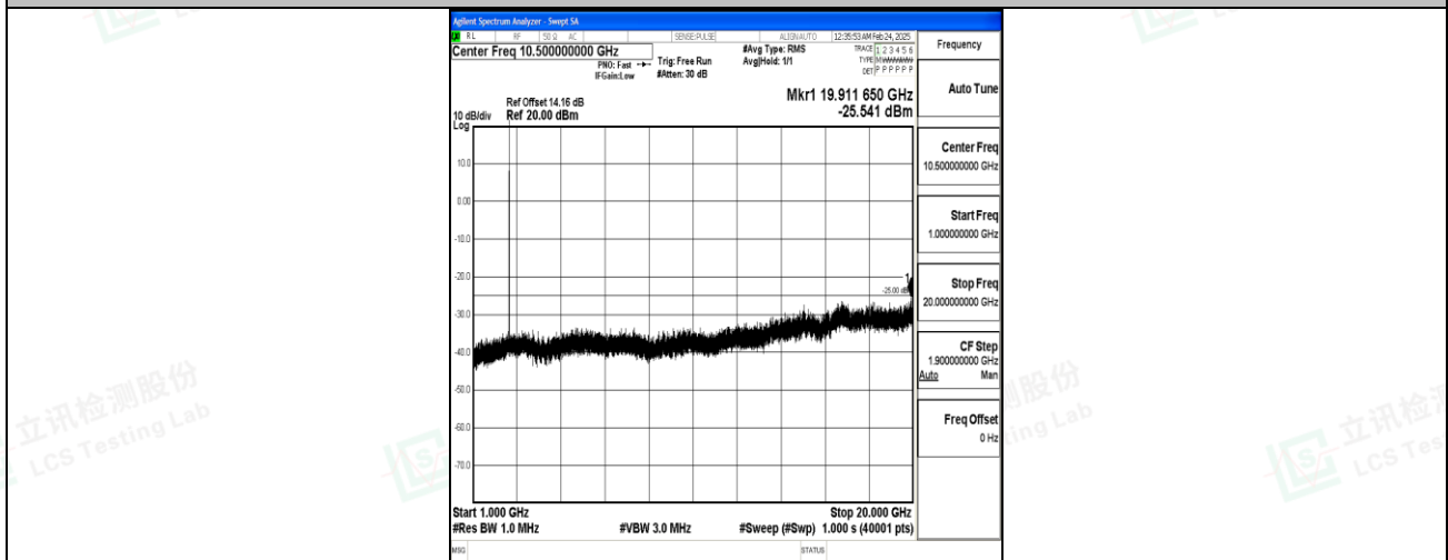
Band7_5MHz_16QAM_21425_1RB#0_1000~20000_1000~20000
