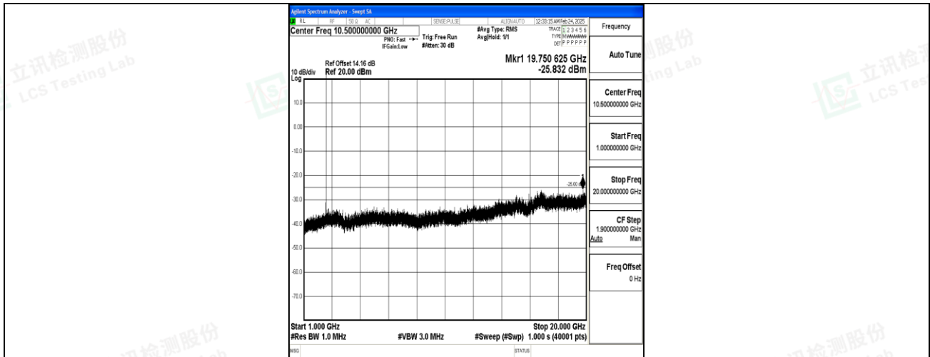
Band7_5MHz_QPSK_20775_1RB#0_1000~20000_1000~20000
