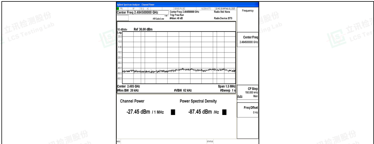
Band7_15MHz_QPSK_20825_75RB#0_Final1
