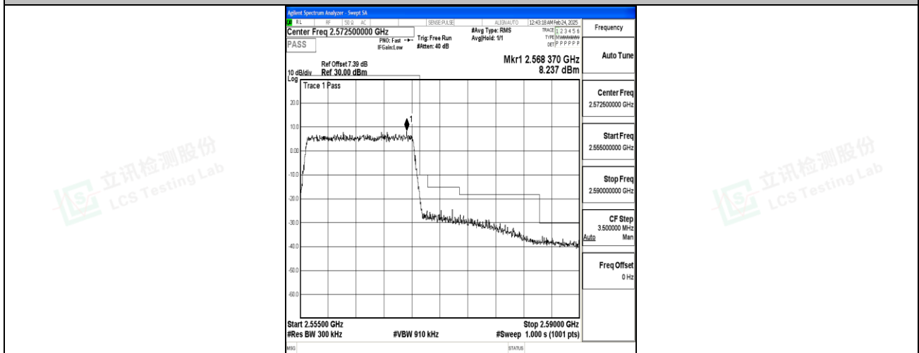
Band7_15MHz_QPSK_21375_75RB#0
