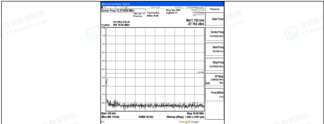
Band7_5MHz_16QAM_20775_1RB#0_0.15~30_0.15~30
