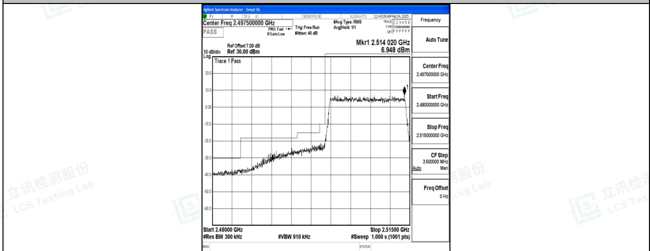
Band7_15MHz_16QAM_20825_75RB#0
