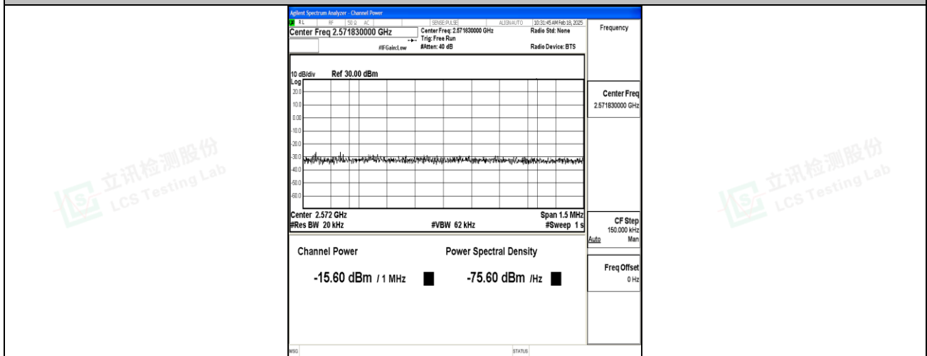
Band7_10MHz_QPSK_21400_50RB#0_Final1
