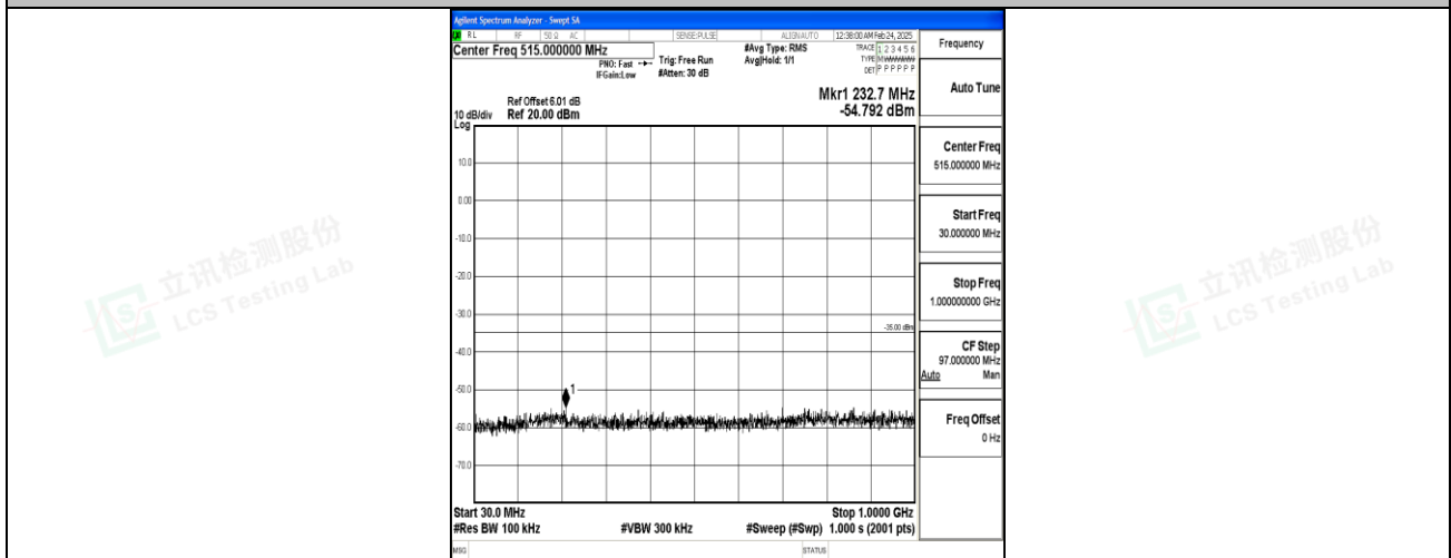
Band7_10MHz_QPSK_20800_1RB#0_30~1000_30~1000
