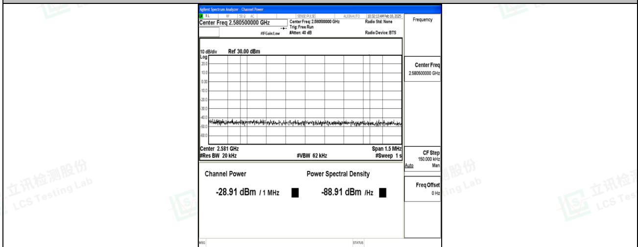
Band7_10MHz_16QAM_21400_50RB#0_Final3
