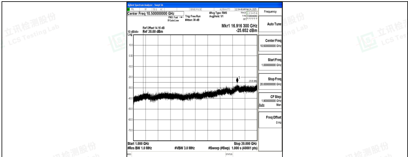
Band7_5MHz_16QAM_21100_1RB#0_1000~20000_1000~20000
