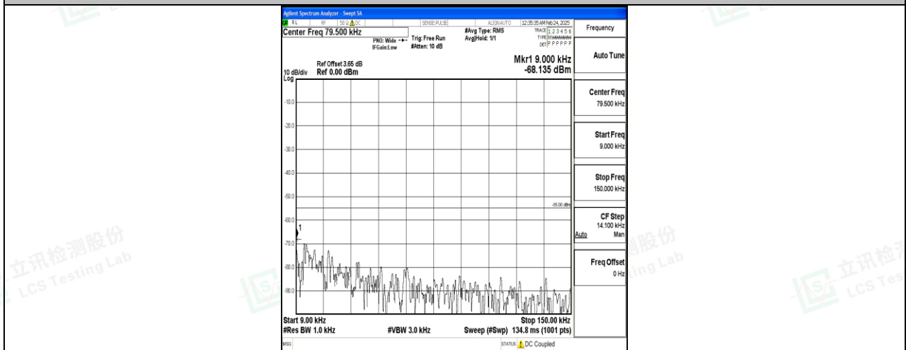
Band7_5MHz_16QAM_21425_1RB#0_0.009~0.15_0.009~0.15
