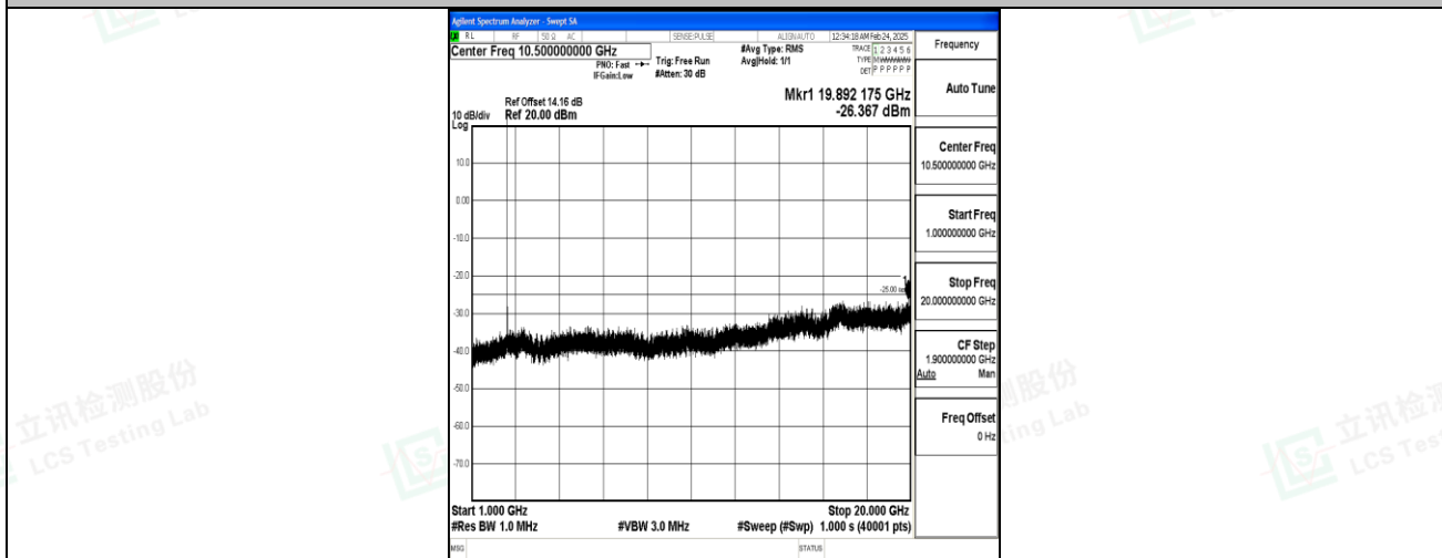
Band7_5MHz_QPSK_21100_1RB#0_1000~20000_1000~20000
