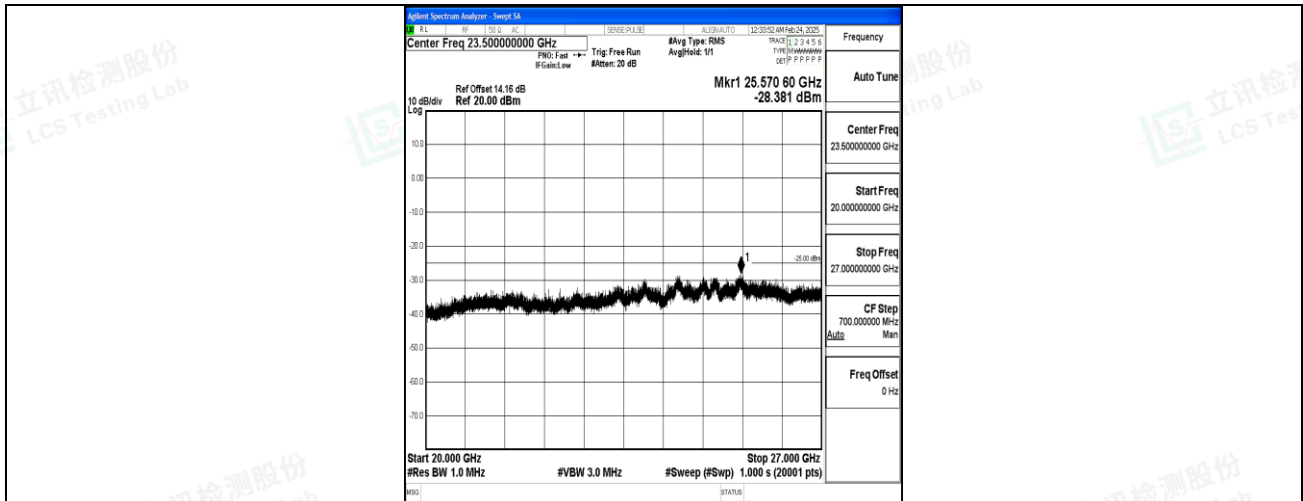
Band7_5MHz_16QAM_20775_1RB#0_20000~27000_20000~27000
