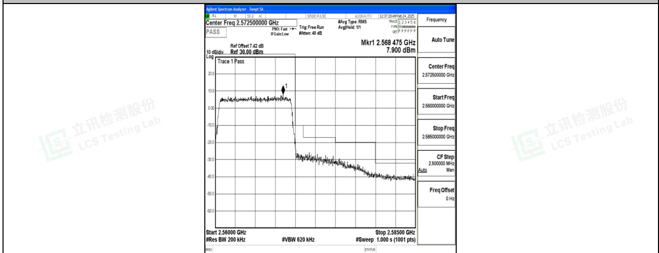
Band7_10MHz_QPSK_21400_50RB#0
