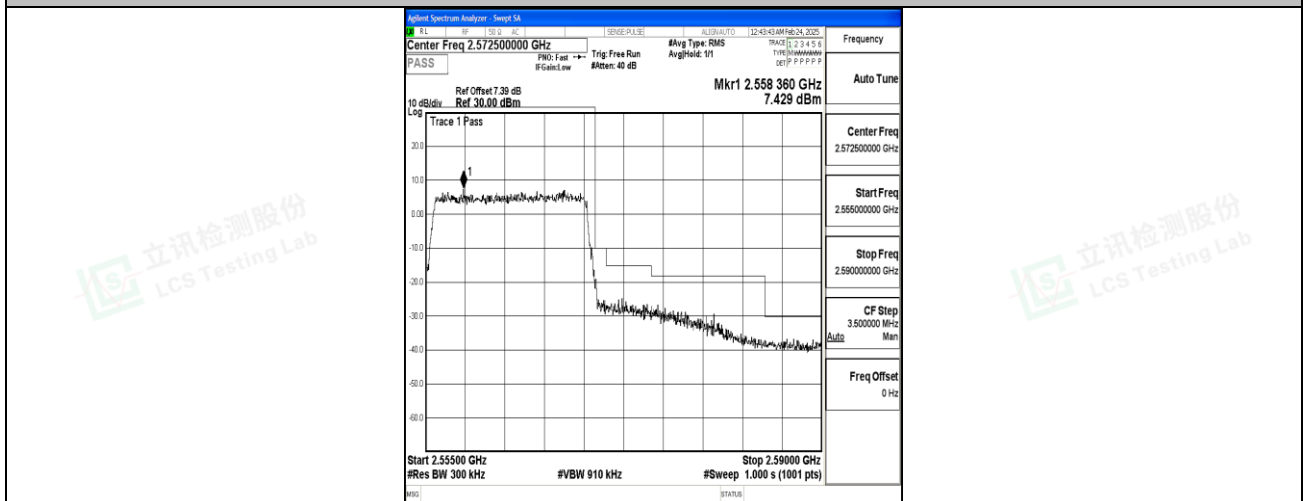
Band7_15MHz_16QAM_21375_75RB#0
