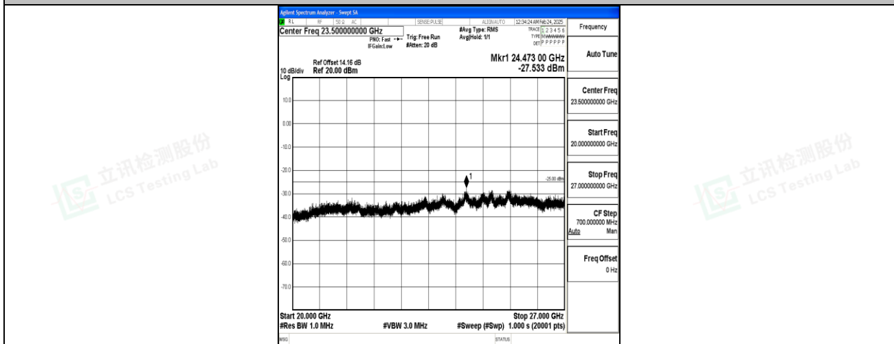
Band7_5MHz_QPSK_21100_1RB#0_20000~27000_20000~27000
