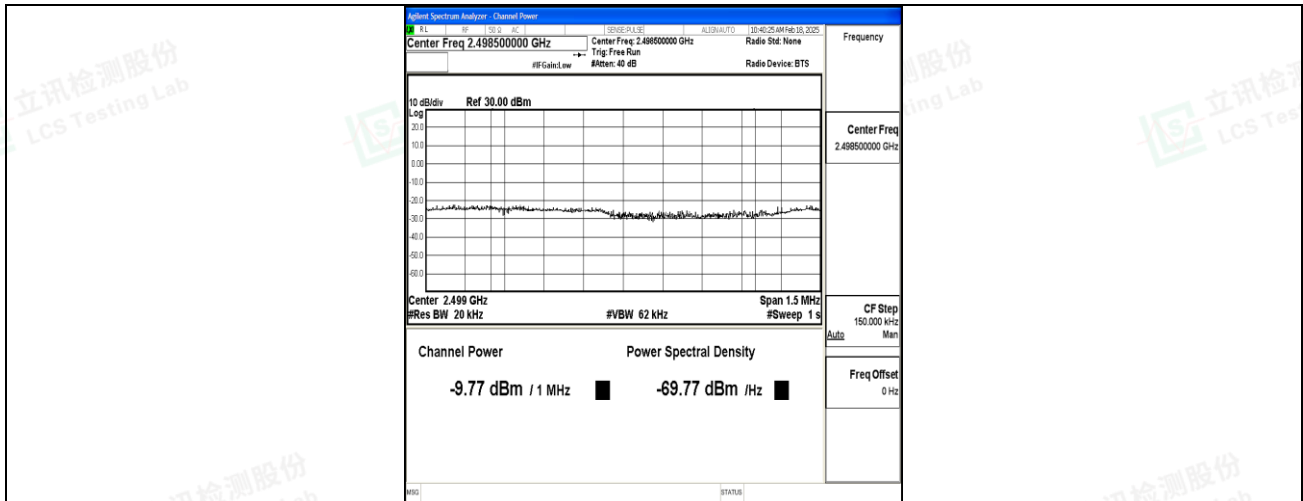
Band7_15MHz_QPSK_20825_75RB#0_Final3
