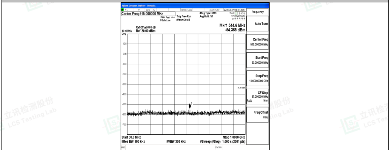
Band7_5MHz_QPSK_21425_1RB#0_30~1000_30~1000
