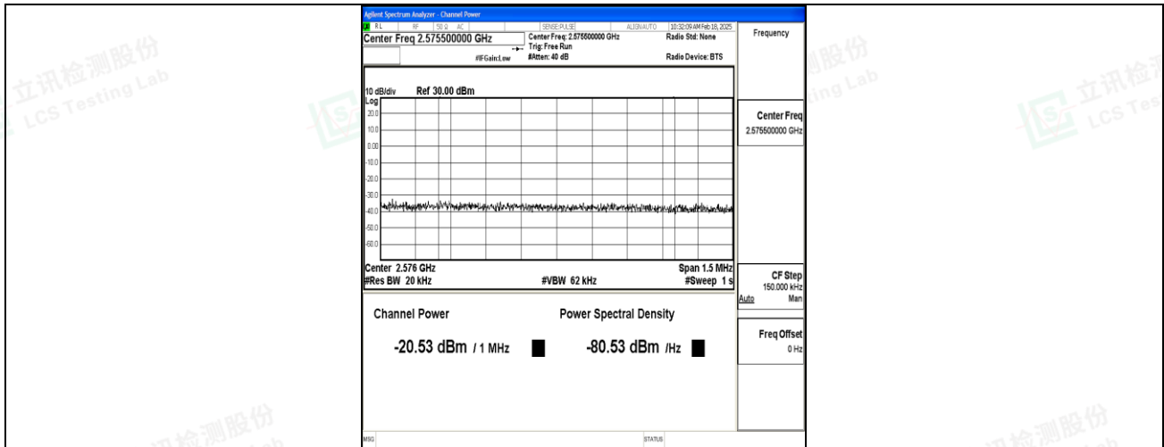
Band7_10MHz_16QAM_21400_50RB#0_Final2
