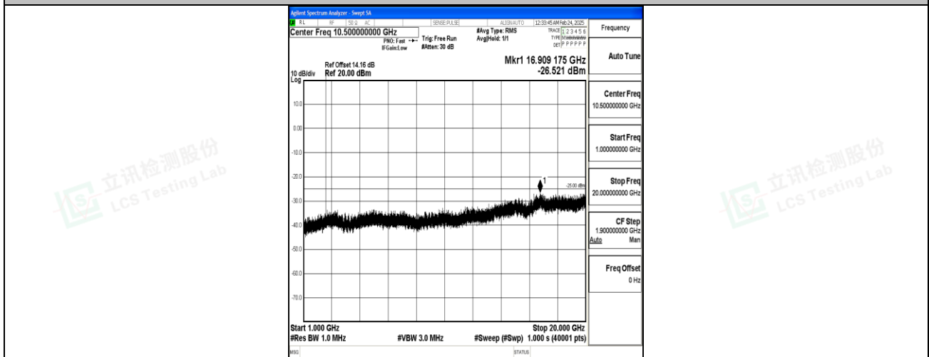
Band7_5MHz_16QAM_20775_1RB#0_1000~20000_1000~20000
