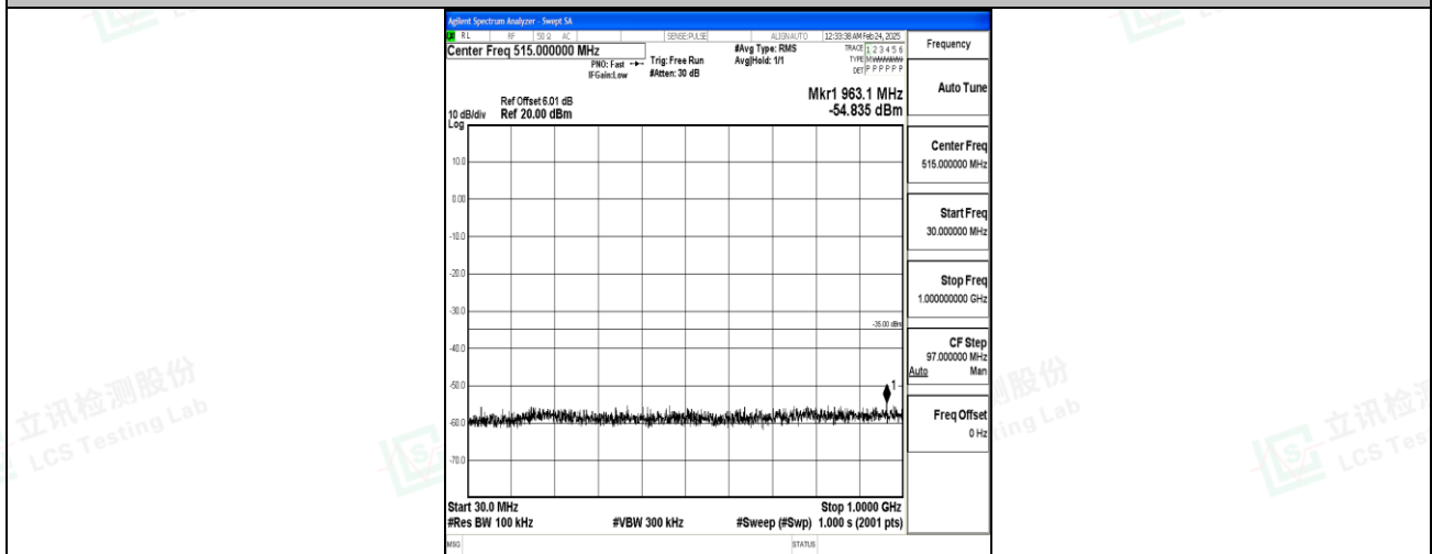
Band7_5MHz_16QAM_20775_1RB#0_30~1000_30~1000
