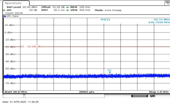
11AX20-CDD_Ant2_2412_30~1000
