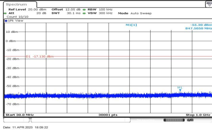
11AX20-CDD_Ant1_2417_30~1000
