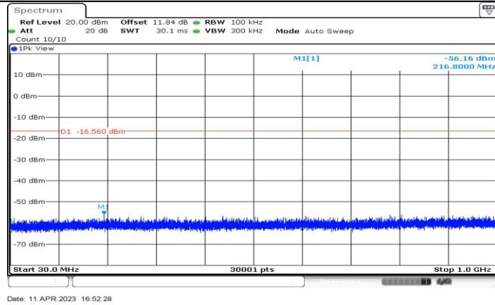
11G-CDD_Ant3_2457_30~1000
