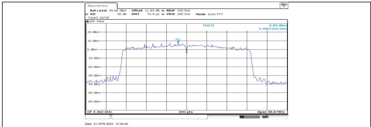
11AX20-CDD_Ant3_2462_0~Reference
