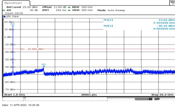
11AX20-CDD_Ant4_2437_1000~26500
