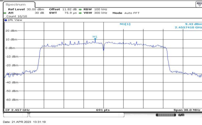
11AX20-CDD_Ant4_2457_0~Reference
