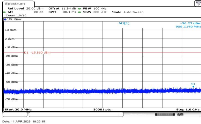
11AX20-CDD_Ant4_2437_30~1000
