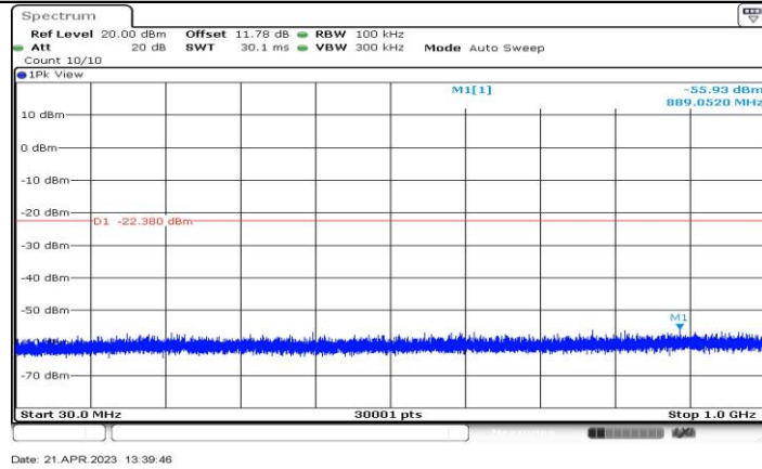
11AX40-CDD_Ant3_2422_30~1000
