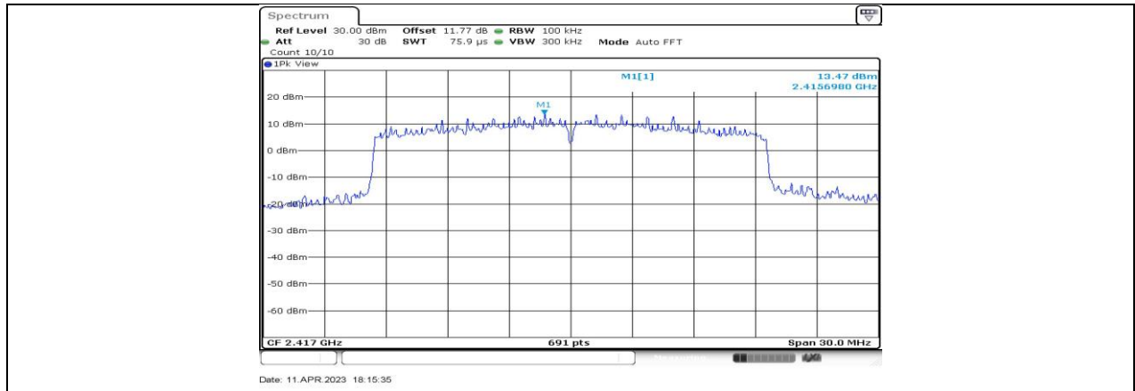
11AX20-CDD_Ant4_2417_0~Reference
