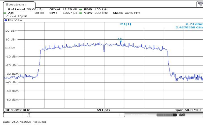
11AX40-CDD_Ant2_2422_0~Reference
