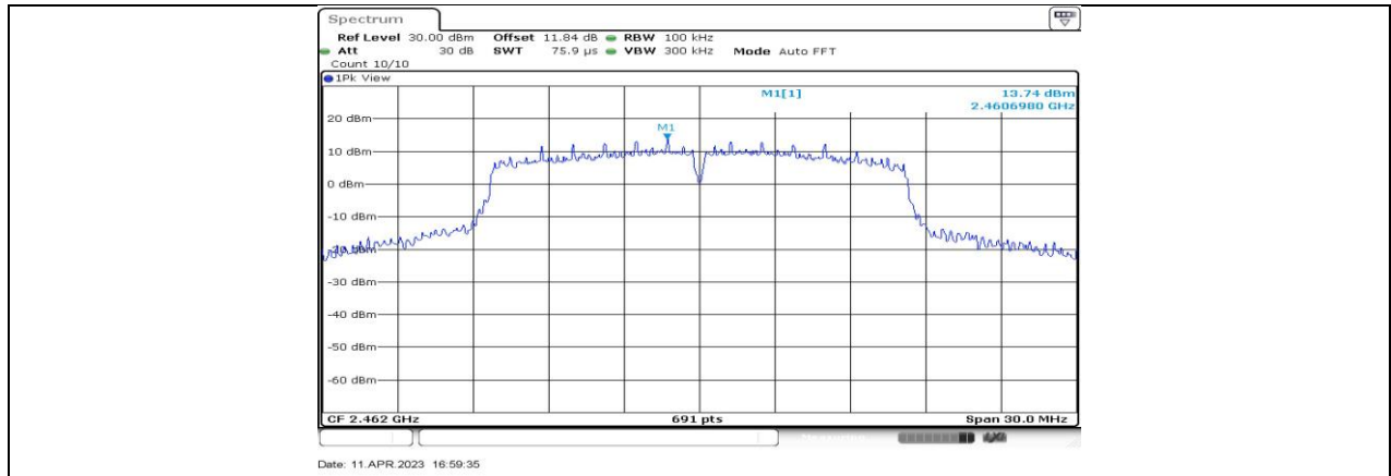
11G-CDD_Ant3_2462_0~Reference
