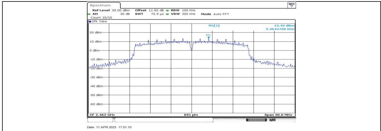
11G-CDD_Ant4_2462_0~Reference
