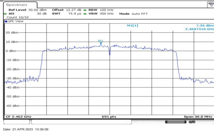
11AX20-CDD_Ant2_2462_0~Reference
