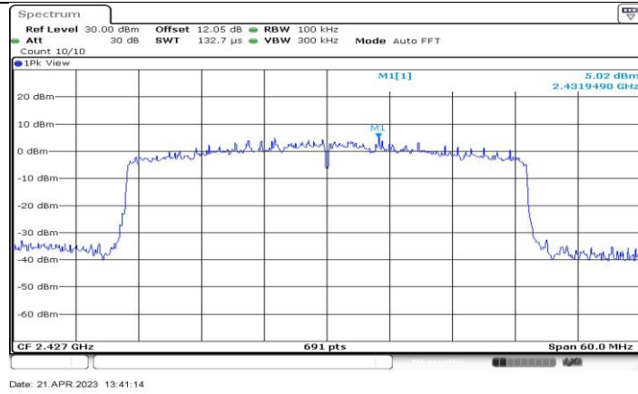
11AX40-CDD_Ant1_2427_0~Reference
