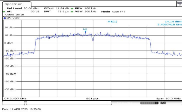
11AX20-CDD_Ant4_2437_0~Reference
