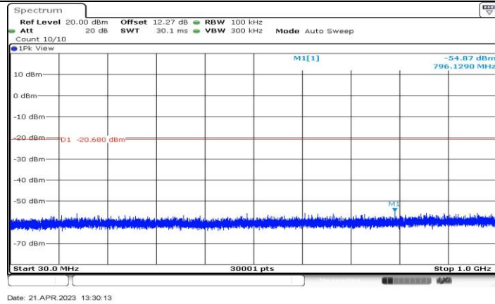
11AX20-CDD_Ant2_2457_30~1000
