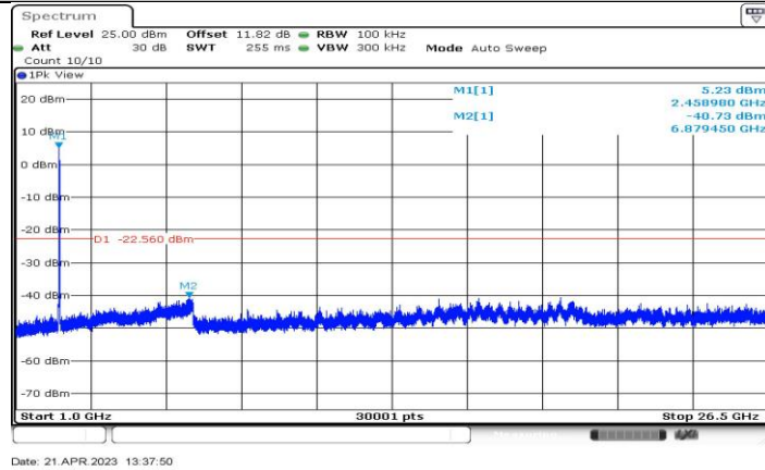
11AX20-CDD_Ant4_2462_1000~26500
