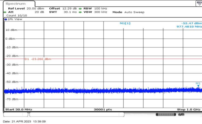
11AX40-CDD_Ant2_2422_30~1000
