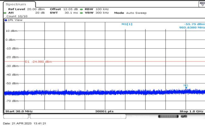
11AX40-CDD_Ant1_2427_30~1000
