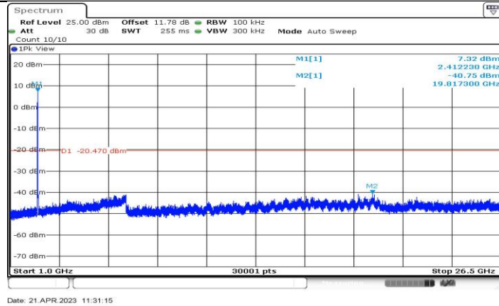
11AX20-CDD_Ant3_2412_1000~26500
