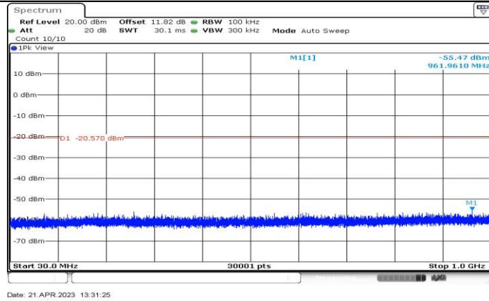
11AX20-CDD_Ant4_2457_30~1000
