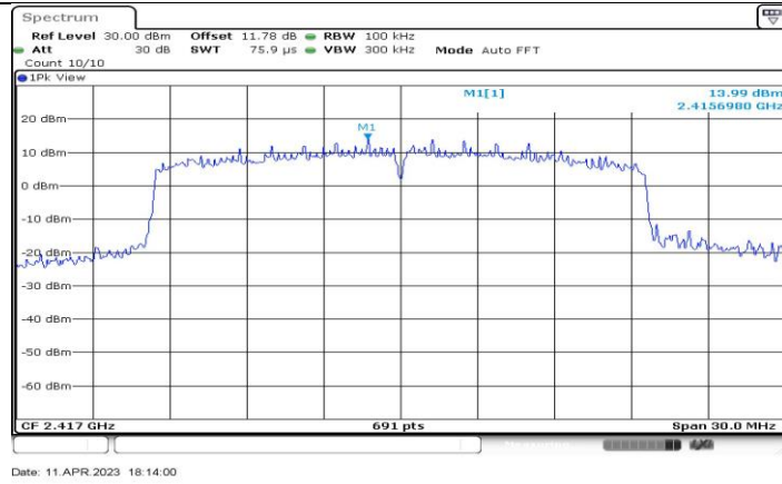
11AX20-CDD_Ant3_2417_0~Reference
