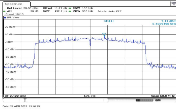
11AX40-CDD_Ant4_2422_0~Reference
