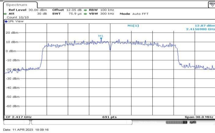
11AX20-CDD_Ant1_2417_0~Reference
