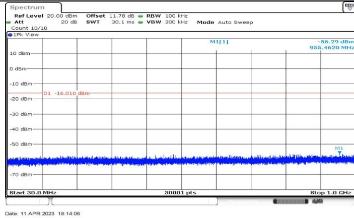
11AX20-CDD_Ant3_2417_30~1000
