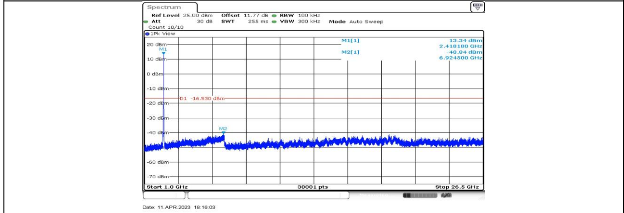
11AX20-CDD_Ant4_2417_1000~26500
