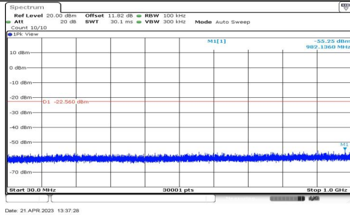
11AX20-CDD_Ant4_2462_30~1000
