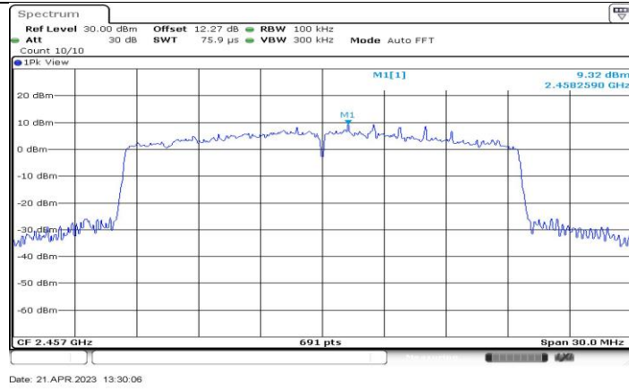
11AX20-CDD_Ant2_2457_0~Reference
