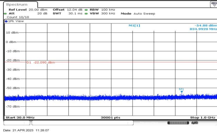
11AX20-CDD_Ant1_2412_30~1000
