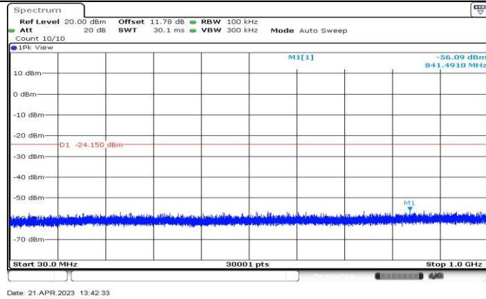
11AX40-CDD_Ant3_2427_30~1000
