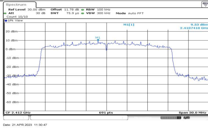
11AX20-CDD_Ant3_2412_0~Reference
