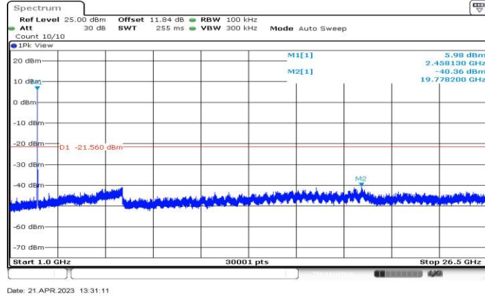
11AX20-CDD_Ant3_2457_1000~26500
