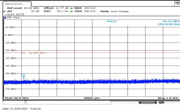
11AX40-CDD_Ant4_2422_30~1000
