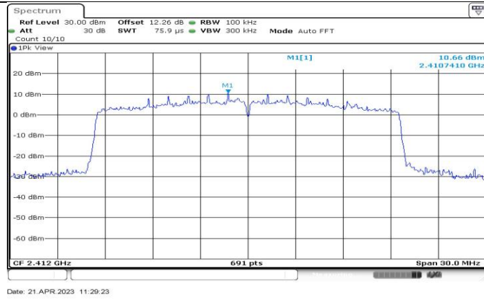
11AX20-CDD_Ant2_2412_0~Reference
