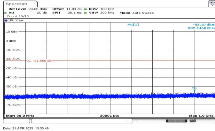
11AX20-CDD_Ant3_2457_30~1000
