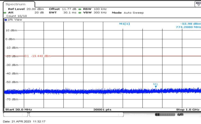
11AX20-CDD_Ant4_2412_30~1000
