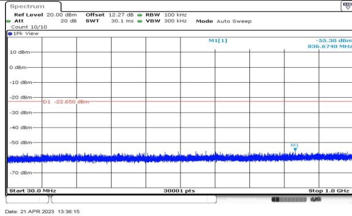
11AX20-CDD_Ant2_2462_30~1000
