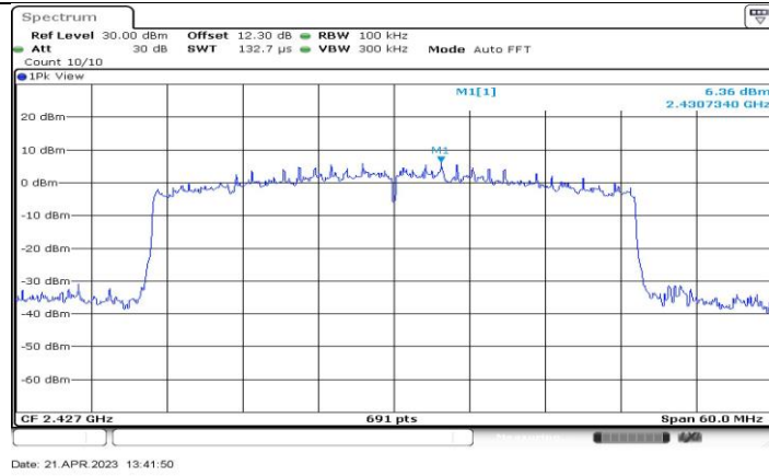
11AX40-CDD_Ant2_2427_0~Reference
