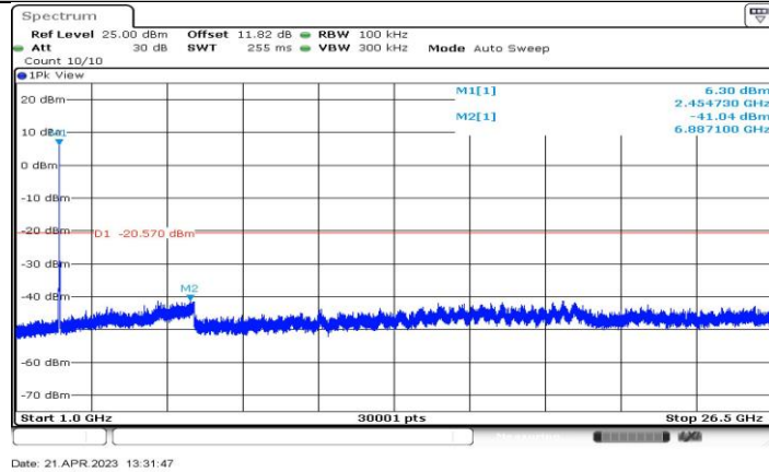
11AX20-CDD_Ant4_2457_1000~26500
