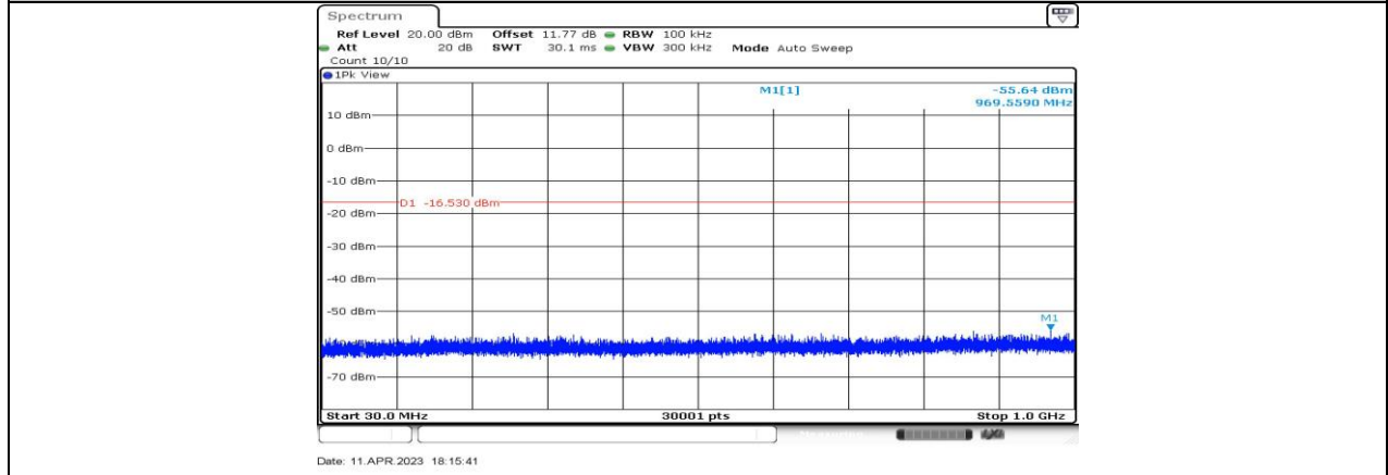
11AX20-CDD_Ant4_2417_30~1000
