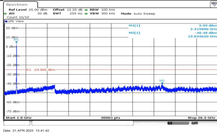
11AX40-CDD_Ant1_2427_1000~26500
