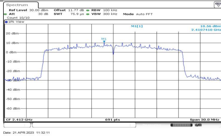
11AX20-CDD_Ant4_2412_0~Reference
