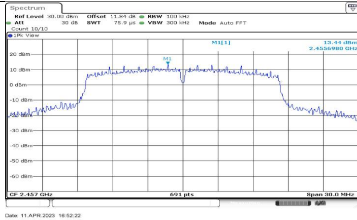
11G-CDD_Ant3_2457_0~Reference
