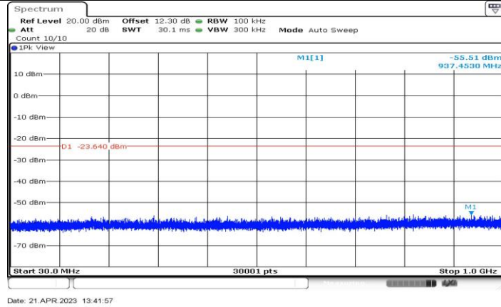
11AX40-CDD_Ant2_2427_30~1000
