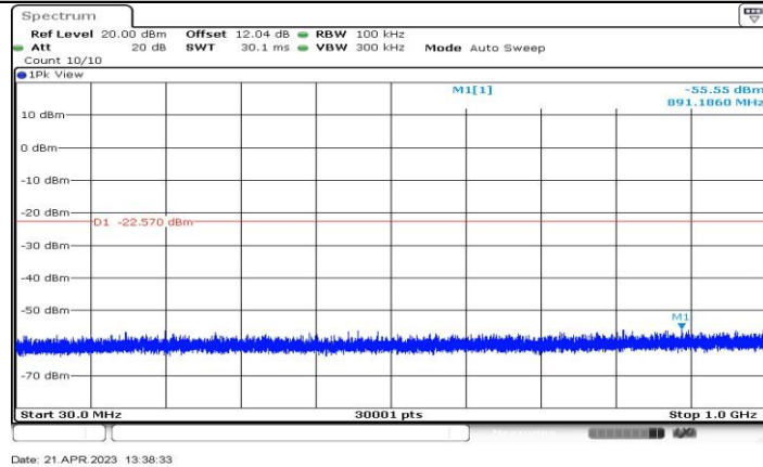
11AX40-CDD_Ant1_2422_30~1000
