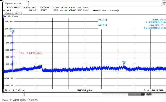
11AX40-CDD_Ant3_2427_1000~26500
