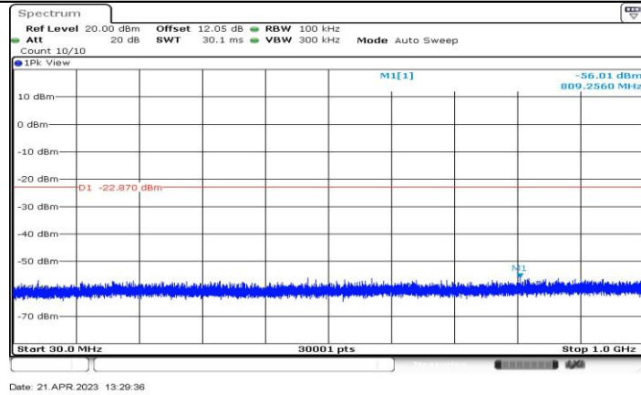
11AX20-CDD_Ant1_2457_30~1000
