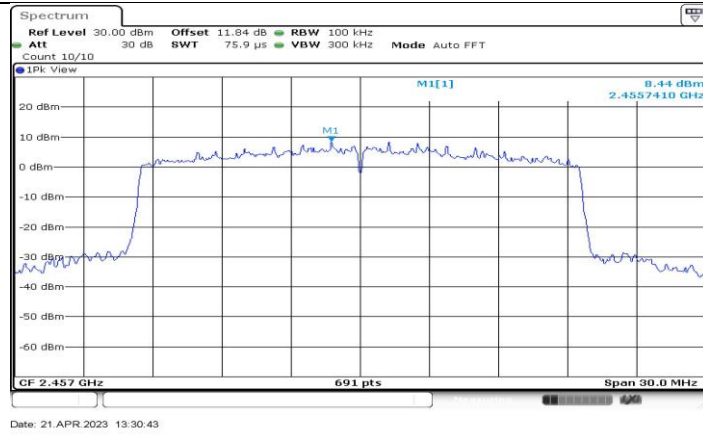
11AX20-CDD_Ant3_2457_0~Reference
