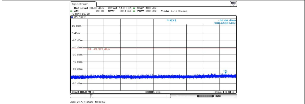
11AX20-CDD_Ant3_2462_30~1000
