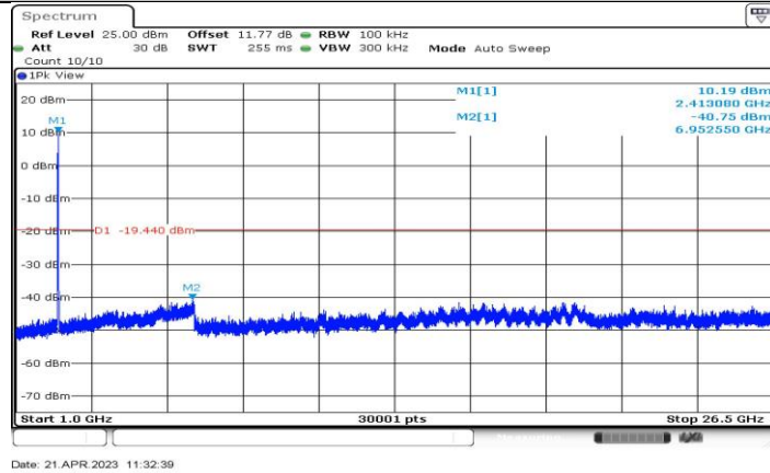
11AX20-CDD_Ant4_2412_1000~26500
