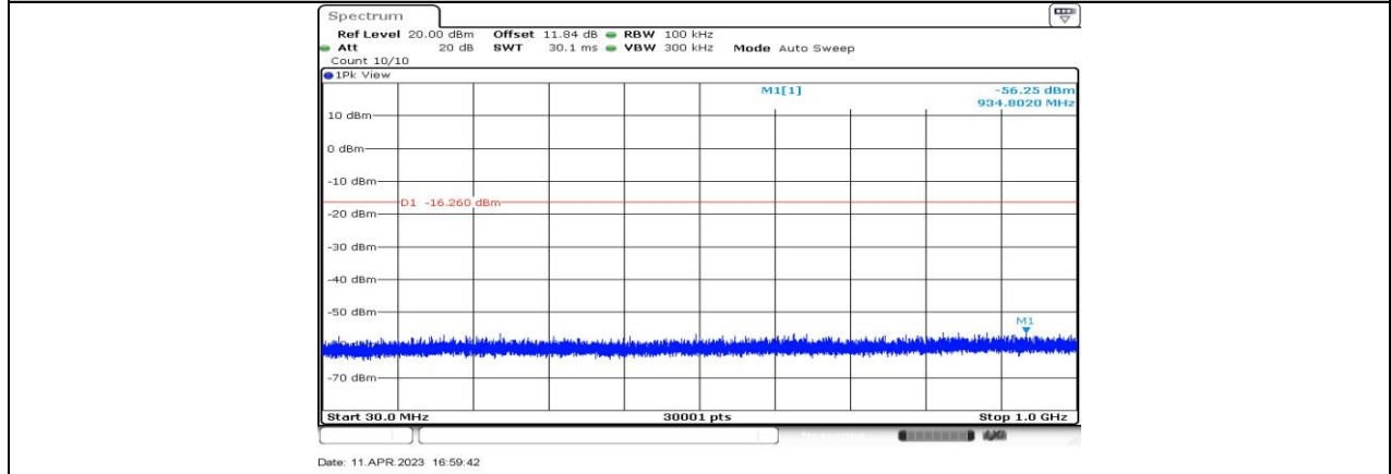
11G-CDD_Ant3_2462_30~1000
