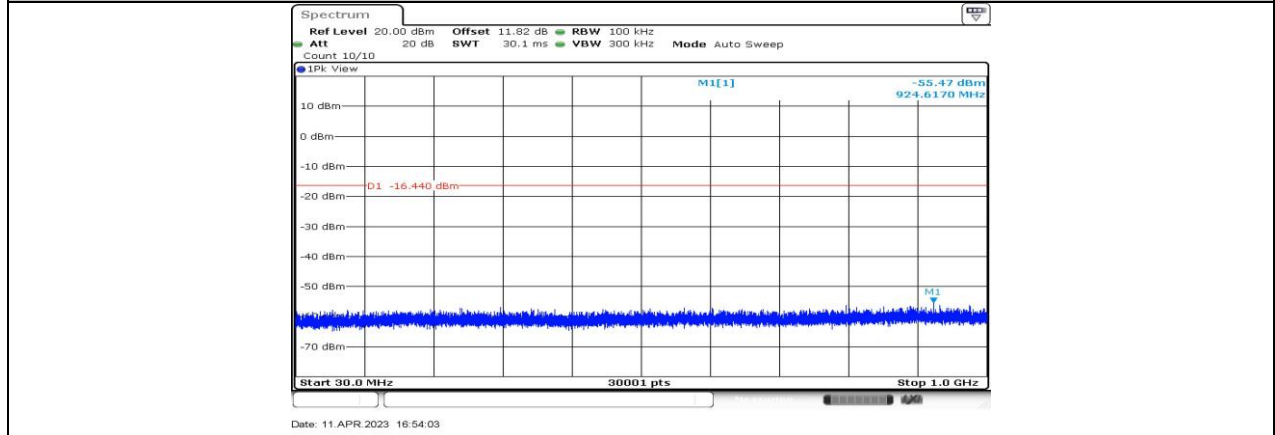
11G-CDD_Ant4_2457_30~1000
