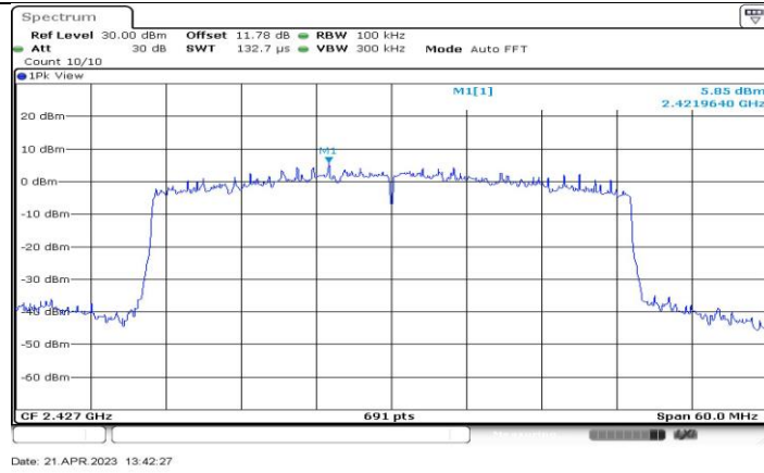
11AX40-CDD_Ant3_2427_0~Reference
