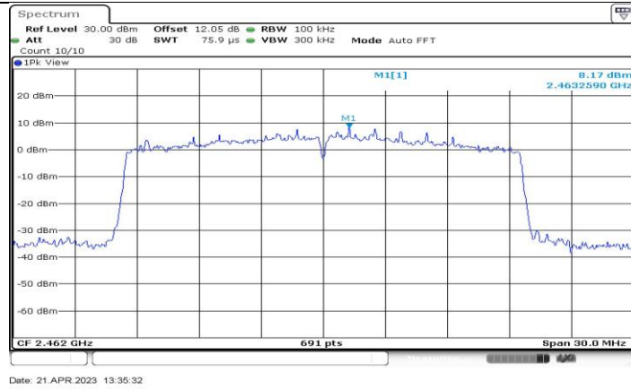
11AX20-CDD_Ant1_2462_0~Reference
