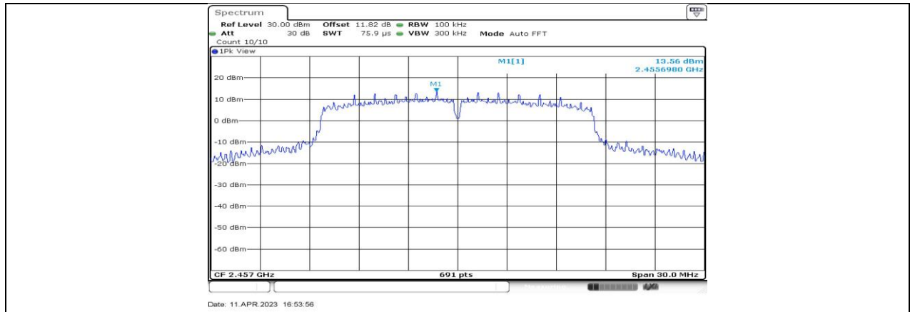
11G-CDD_Ant4_2457_0~Reference
