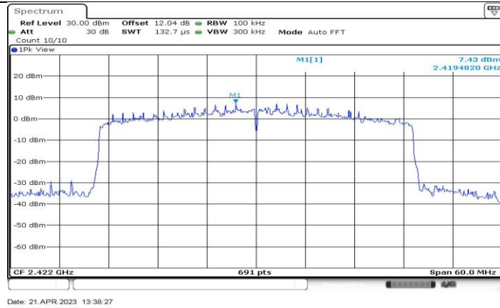
11AX40-CDD_Ant1_2422_0~Reference
