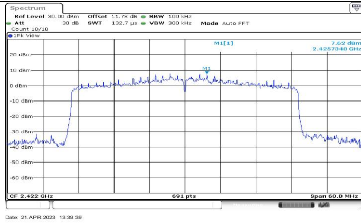
11AX40-CDD_Ant3_2422_0~Reference
