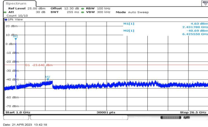
11AX40-CDD_Ant2_2427_1000~26500
