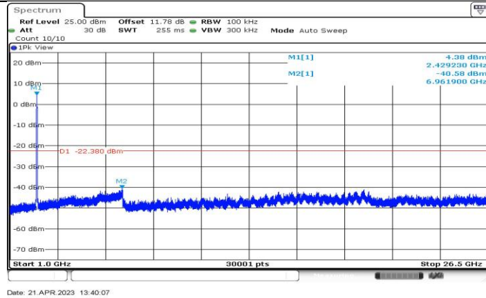
11AX40-CDD_Ant3_2422_1000~26500
