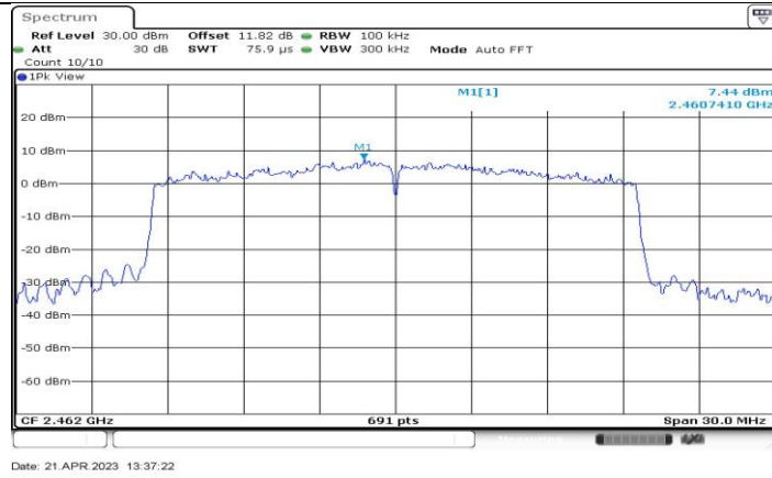
11AX20-CDD_Ant4_2462_0~Reference
