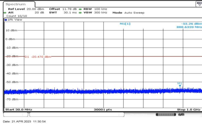
11AX20-CDD_Ant3_2412_30~1000
