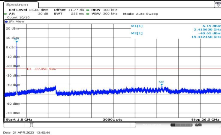
11AX40-CDD_Ant4_2422_1000~26500
