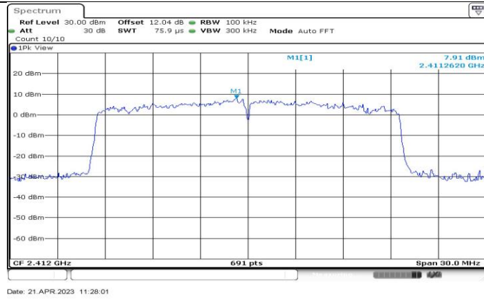
11AX20-CDD_Ant1_2412_0~Reference
