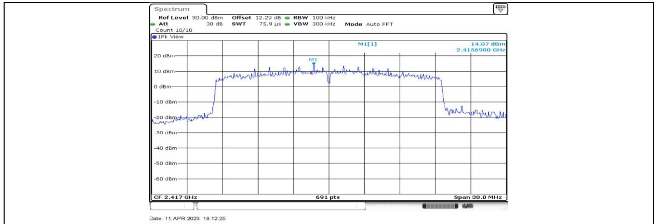
11AX20-CDD_Ant2_2417_0~Reference
