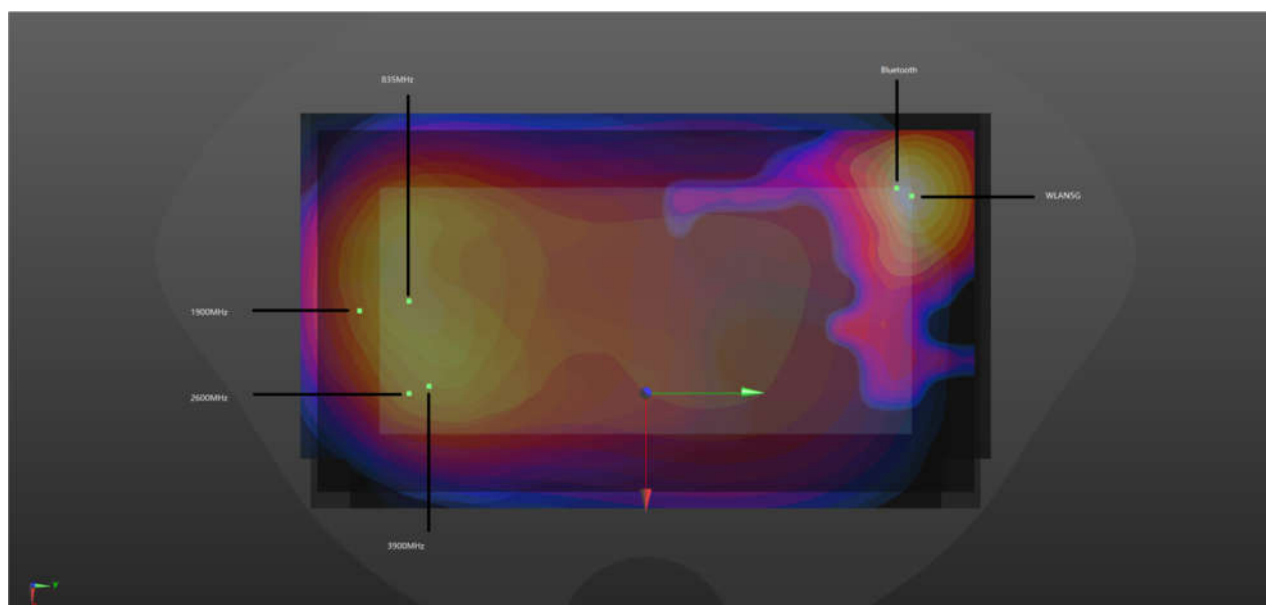
WWAN+5GHz+Bluetooth (5mm)_Body-worn
