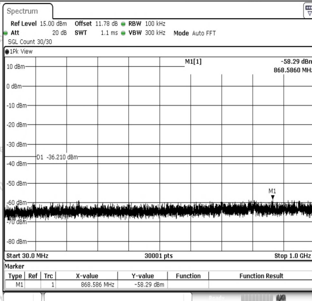
11N20SISO-Ant1-2412-30~1000-PASS
