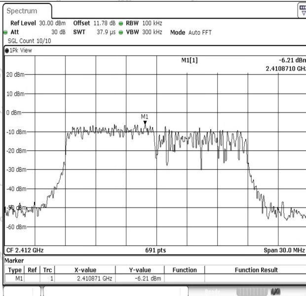
11N20SISO-Ant1-2412-0~Reference-PASS
