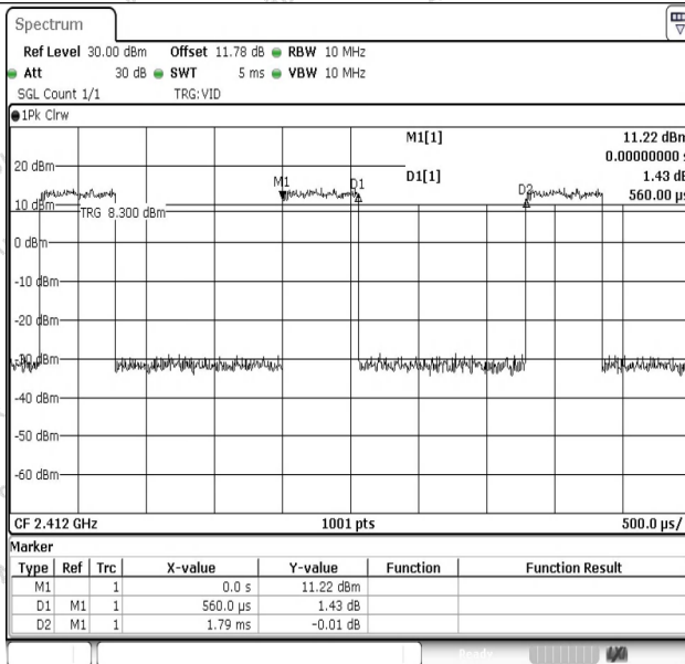
NTNV-11N20SISO-Ant1-2412
