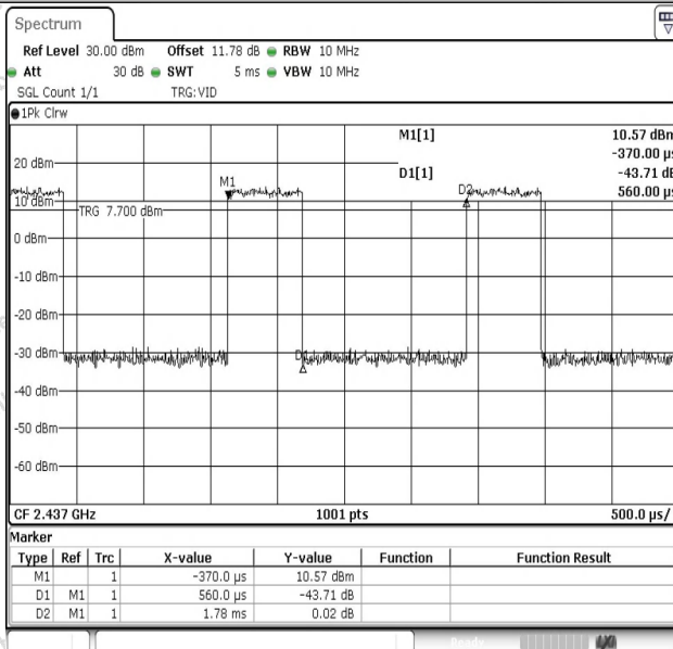
NTNV-11N20SISO-Ant1-2437
