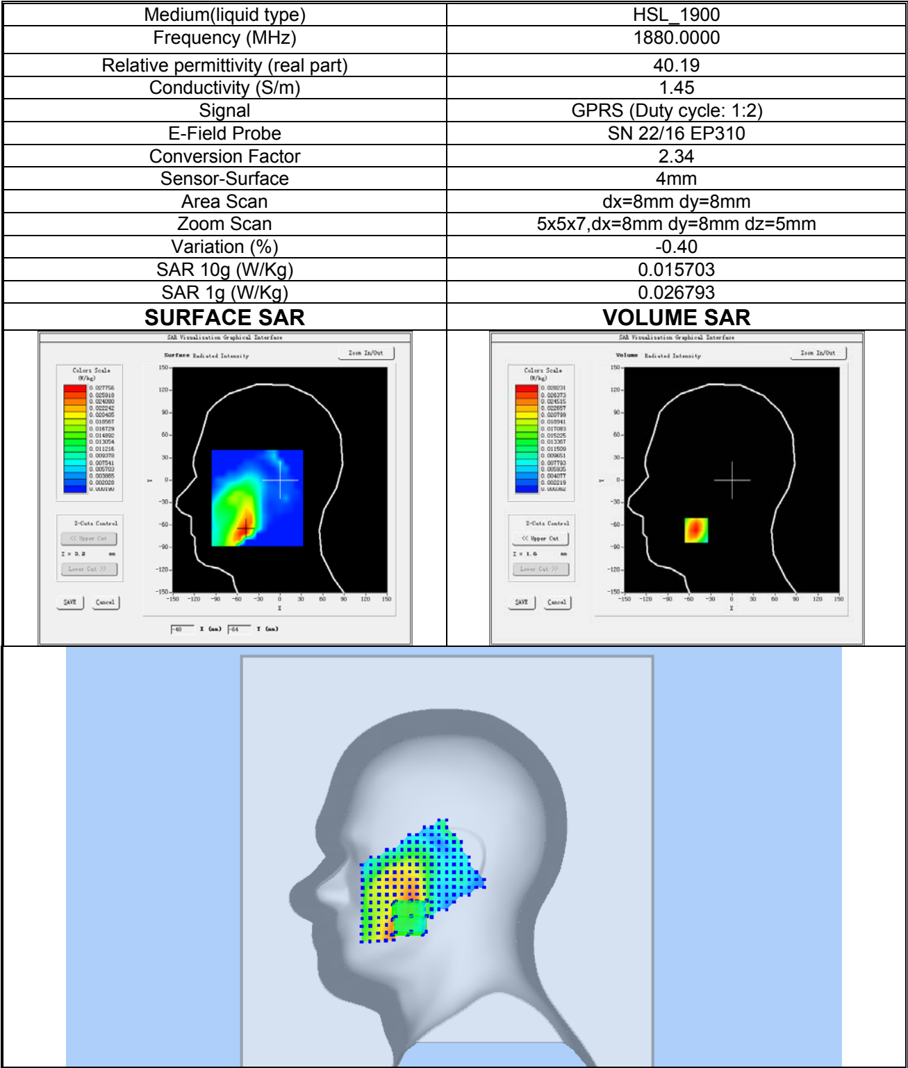
Plot 3: GPRS1900, Mid channel (Right Head Cheek) Product Description: Smartphone Test Date: 2022-05-15
