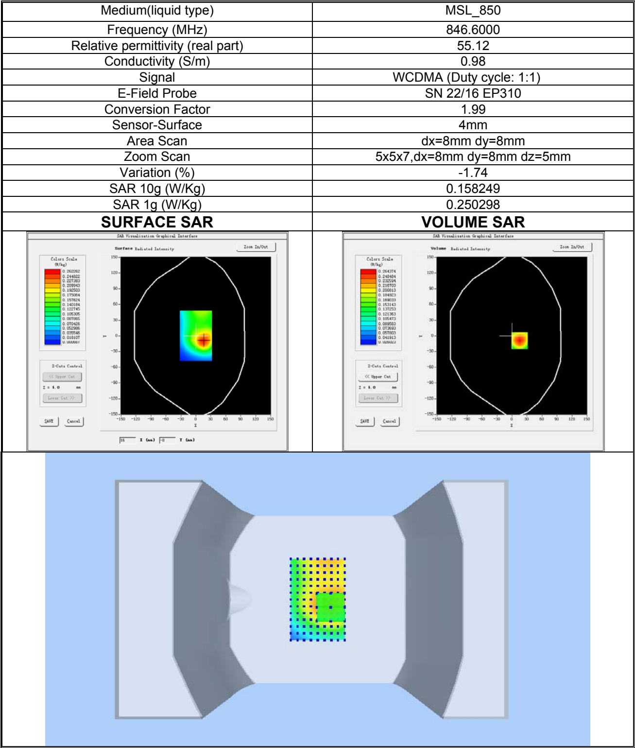
Plot 6: WCDMA BAND V, High channel (Body-worn /Hotspot, Back side) Product Description: Smartphone Test Date: 2022-04-30
