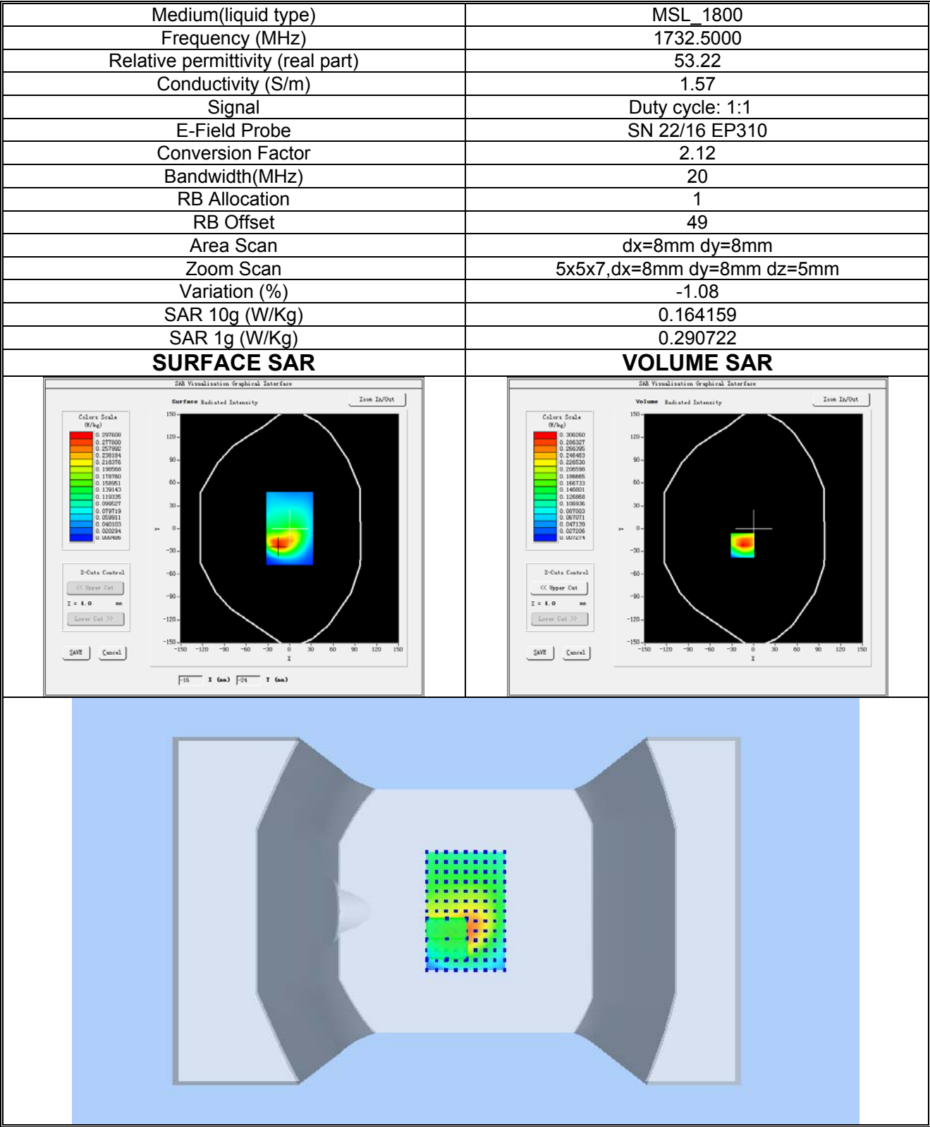
Plot 10:LTE BAND 4, Middle channel (Body-worn /Hotspot, Back side) Product Description:Smartphone Test Date: 2022-05-10
