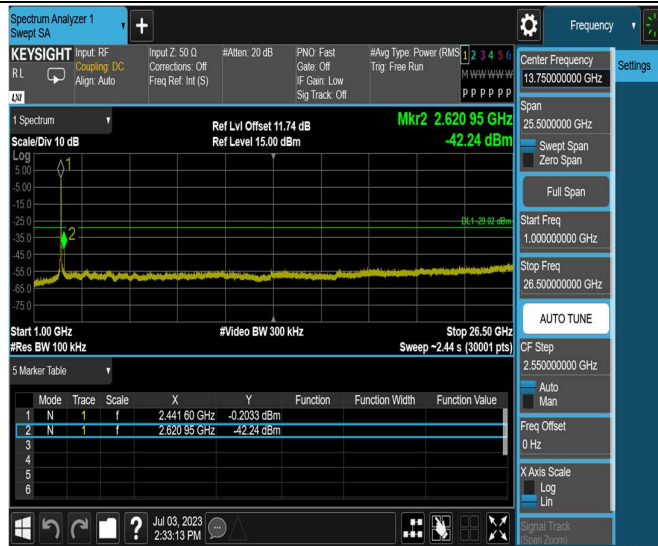
11N40SISO_Ant1_2452_0~Reference
