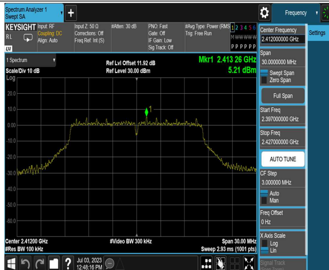
11G_Ant1_2412_0~Reference
