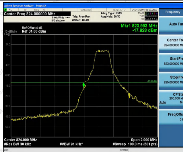
Band26-1.4MHz-QPSK-26797-1RB#5
