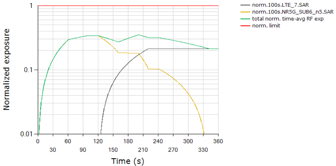
Total Normalized Time-averaged RF Exposure Tech: LTE, Band 7 / Tech: NR5G SUB6, Band n5
