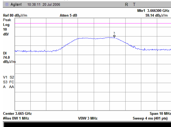
Plot 7.3.16 Radiated emission measurements at the forth harmonic
