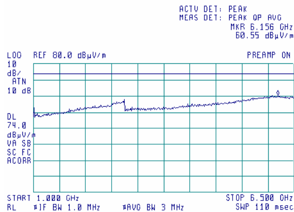
Plot 7.3.6 Radiated emission measurements from 1000 to 6500 MHz
