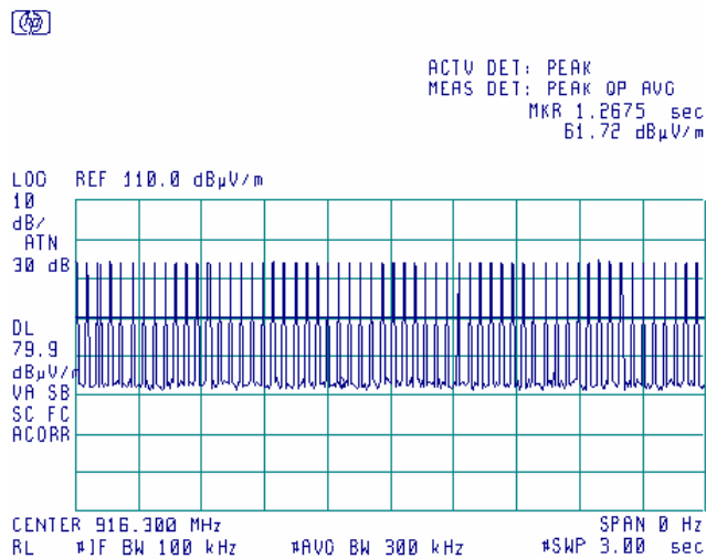
Plot 7.3.28 Transmission burst duration FSK modulation
