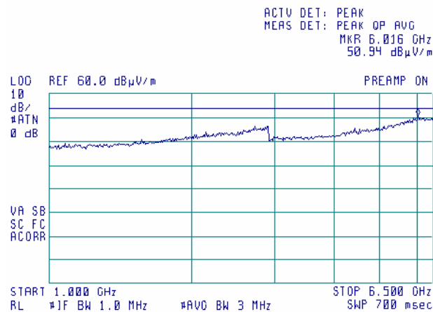
Plot 8.1.4 Radiated emission measurements above 1000 MHz, horizontal antenna polarization
