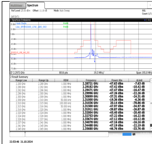
Band40(2305-2315)-5MHz-16QAM-38775-1RB#24-PASS
