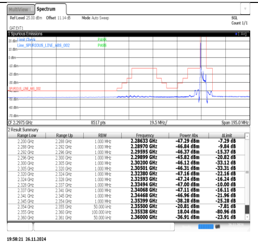
Band40(2350-2360)-5MHz-QPSK-39225-1RB#24-PASS
