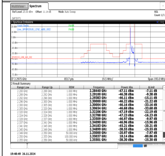
Band40(2350-2360)-5MHz-16QAM-39175-1RB#24-PASS
