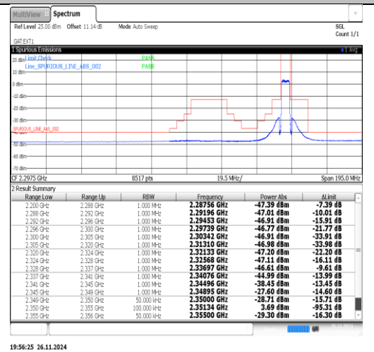
Band40(2350-2360)-5MHz-16QAM-39225-1RB#0-PASS
