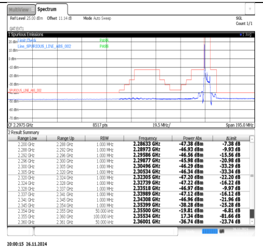
Band40(2350-2360)-5MHz-16QAM-39225-1RB#24-PASS
