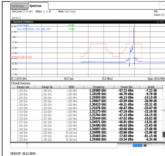
Band40(2350-2360)-5MHz-16QAM-39225-25RB#0-PASS
