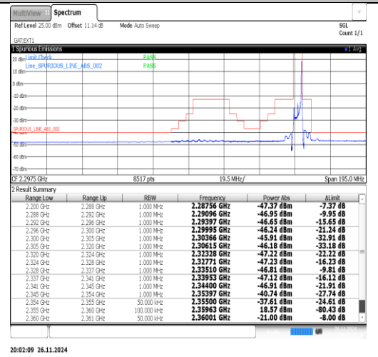
Band40(2350-2360)-5MHz-16QAM-39175-25RB#0-PASS
