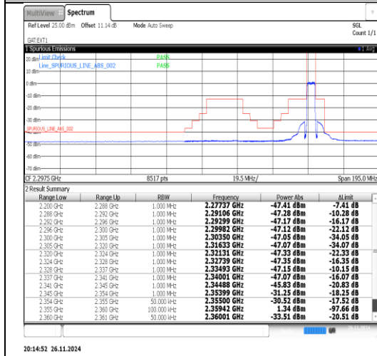
Band40(2350-2360)-5MHz-16QAM-39175-1RB#0-PASS
