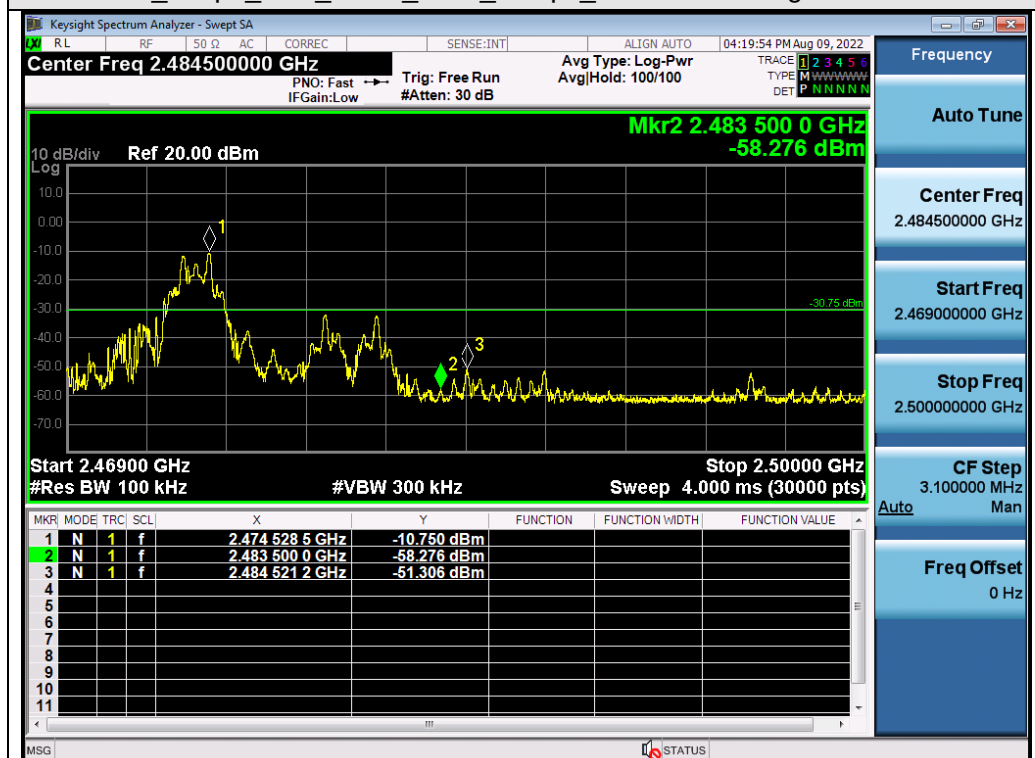
Test_Graph_FSK_ANT1_2474_2Mbps_Higher Band Edge Emissions
