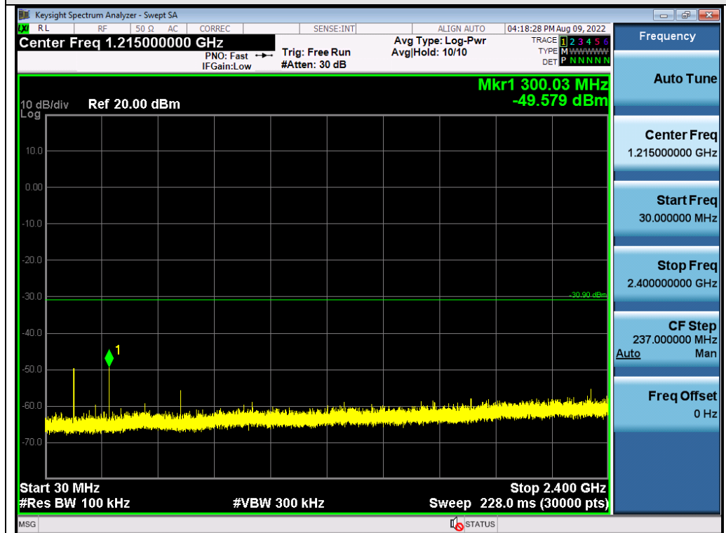
Test_Graph_FSK_ANT1_2474_2Mbps_Lower Band Emissions
