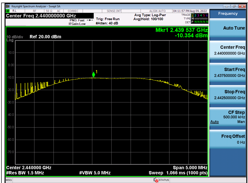
Test_Graph_FSK_ANT1_2440_2Mbps_Peak Power
