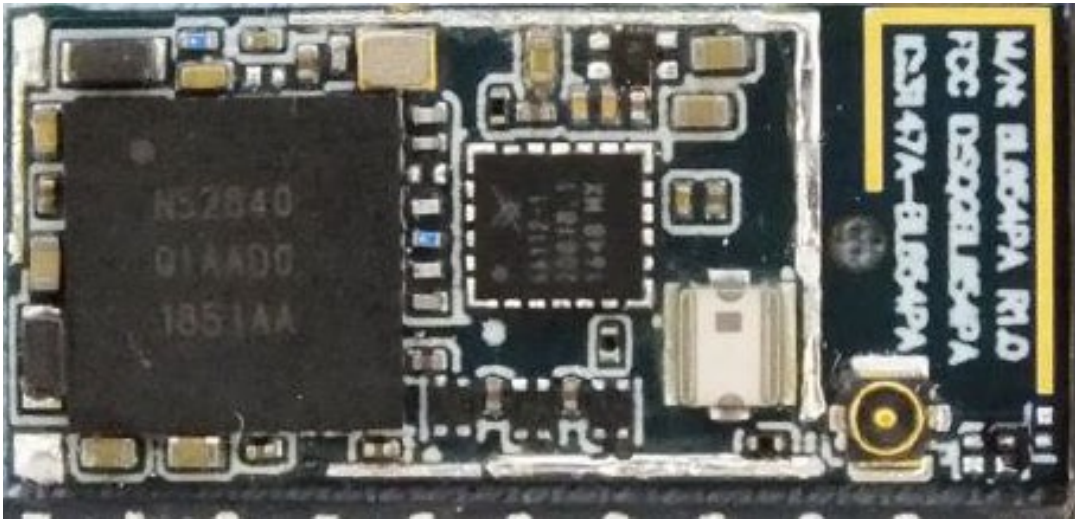
External Antenna
