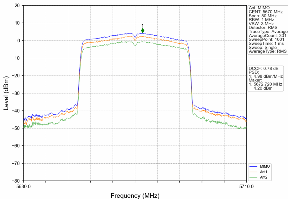
802.11ax(HEW40)_HCH_5670MHz_RU484_Left_MIMO_NTNV
