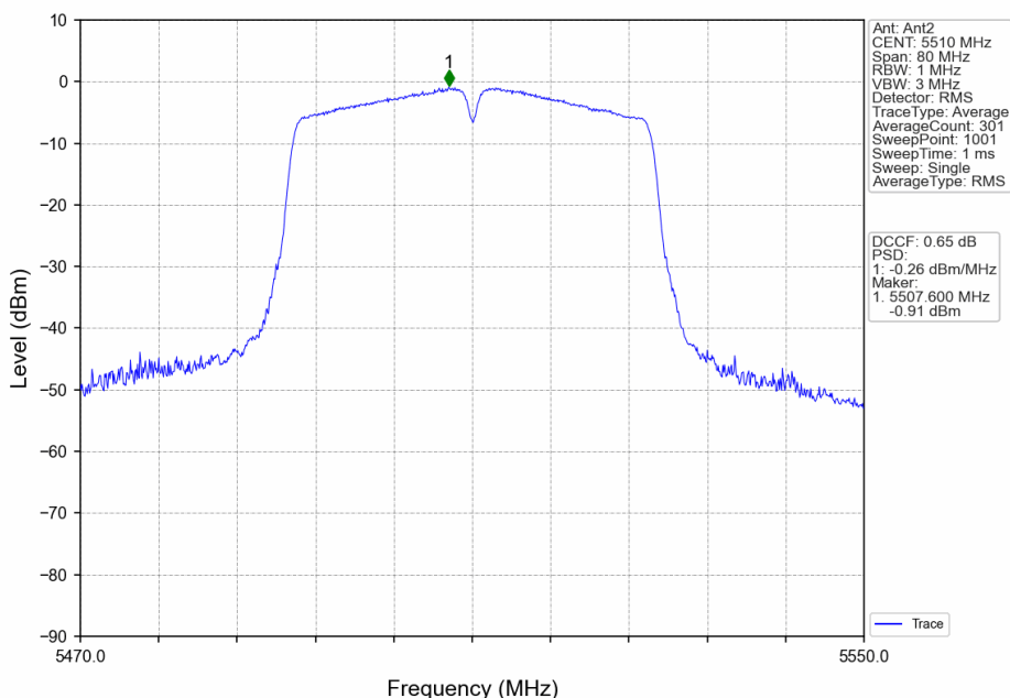
802.11ac(VHT40)_LCH_5510MHz_MIMO_NTNV
