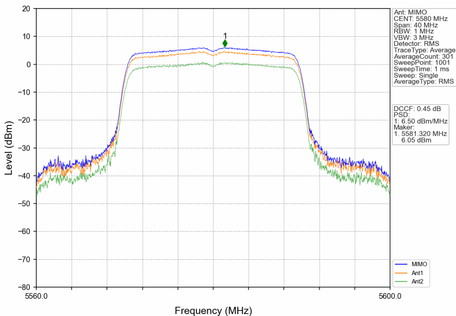
802.11ax(HEW20)_MCH_5580MHz_RU242_Left_MIMO_NTNV
