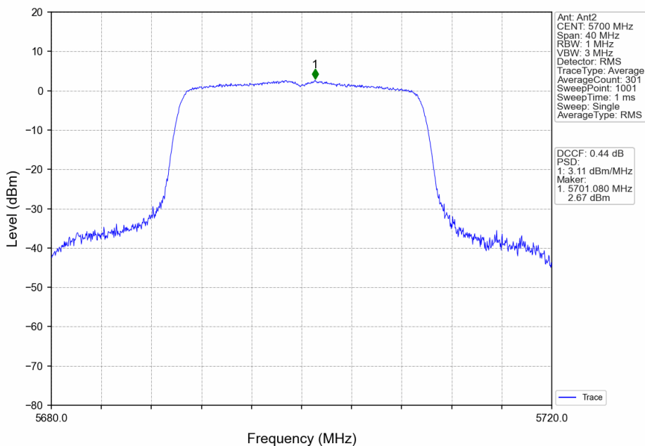
802.11ax(HEW20)_HCH_5700MHz_RU242_Left_Ant2_NTNV
