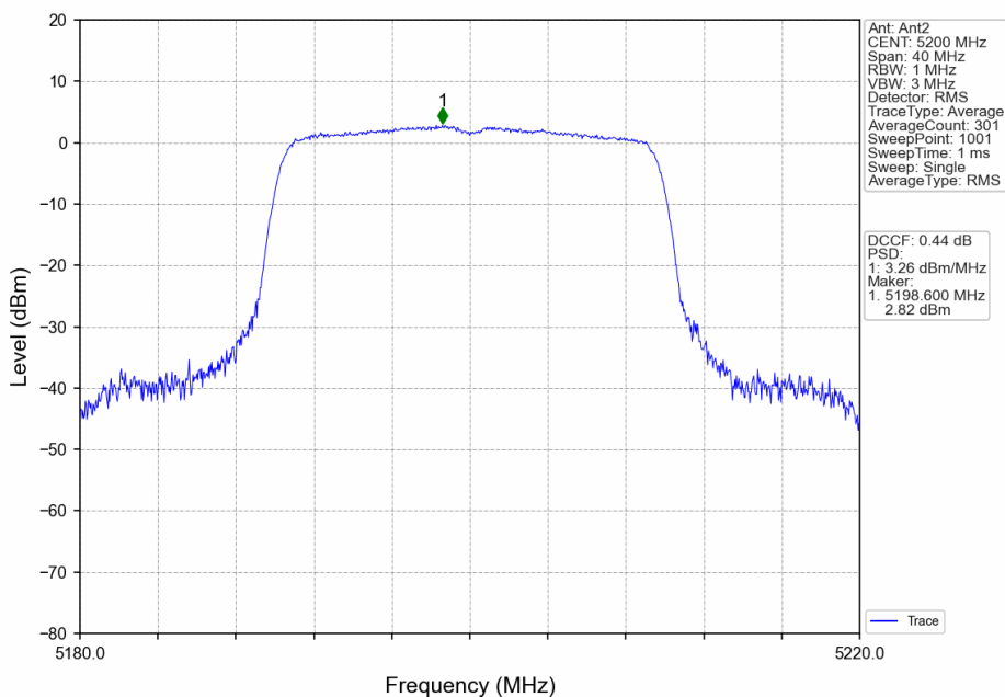
802.11ax(HEW20)_MCH_5200MHz_RU242_Left_MIMO_NTNV
