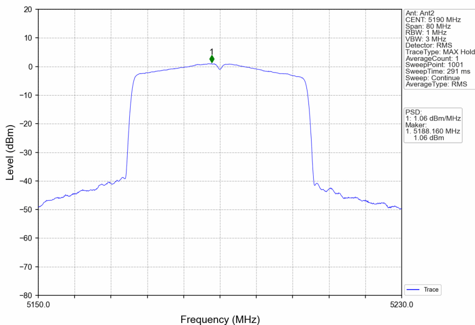
802.11ax(HEW40)_LCH_5190MHz_RU484_Left_MIMO_NTNV
