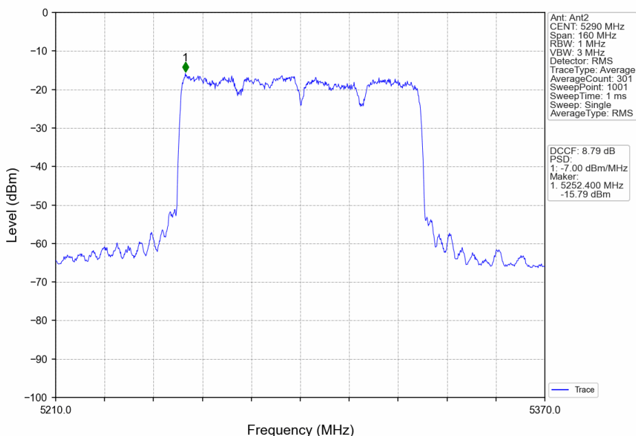
802.11ac(VHT80)_MCH_5290MHz_MIMO_NTNV
