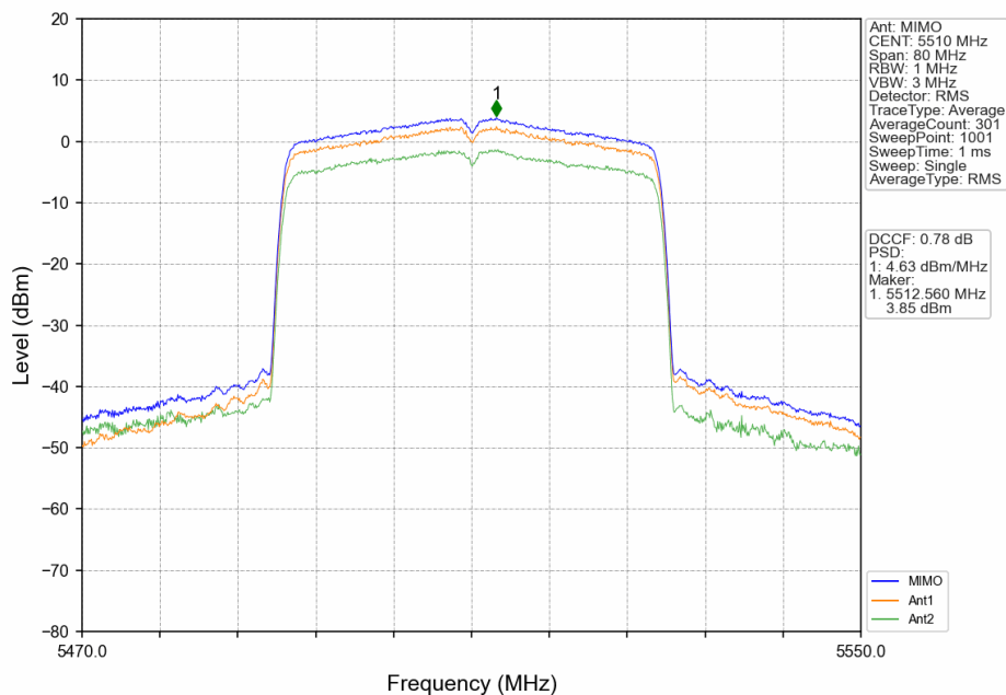
802.11ax(HEW40)_LCH_5510MHz_RU484_Left_MIMO_NTNV
