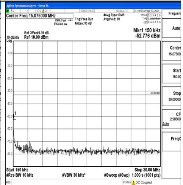
Band2_3MHz_QPSK_18615_1RB#0_0.15~30_0.15~30
