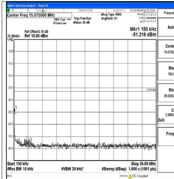
Band2_1.4MHz_16QAM_18900_1RB#0_0.15~30_0.1 5~30
