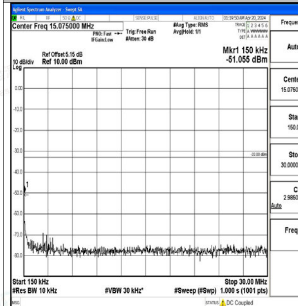
Band2_1.4MHz_16QAM_19193_1RB#0_0.15~30_0.15~30
