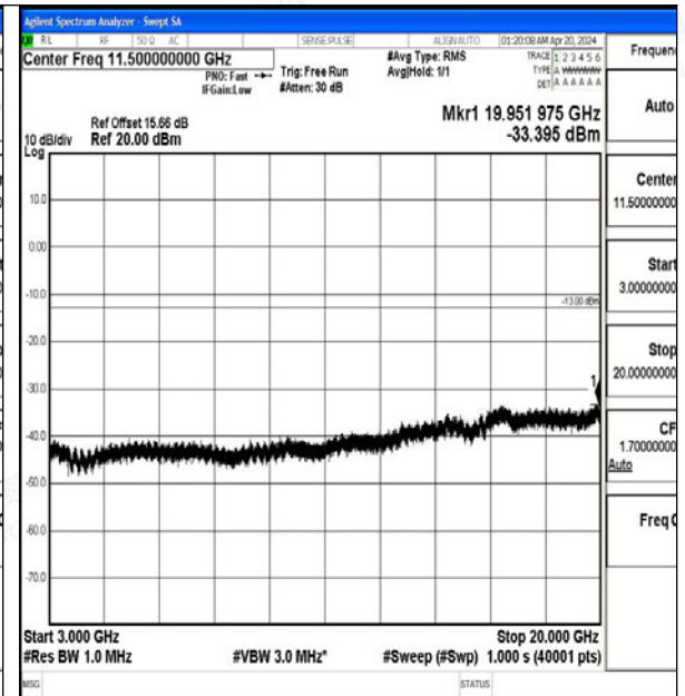
Band2_1.4MHz_16QAM_19193_1RB#0_3000~20000_3000~20000
