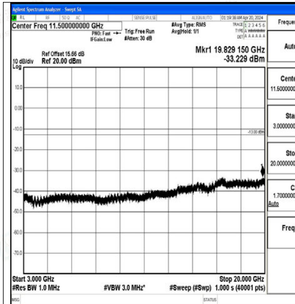
Band2_1.4MHz_QPSK_19193_1RB#0_3000~20000_3000~20000
