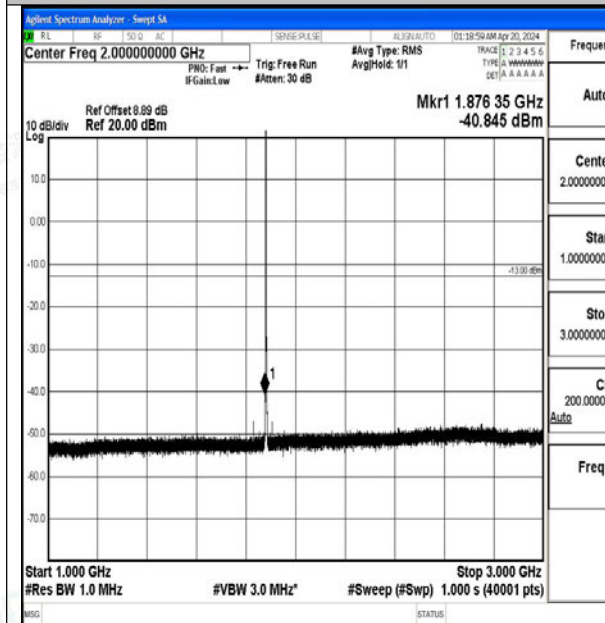
Band2_1.4MHz_16QAM_18900_1RB#0_1000~3000_ 1000~3000
