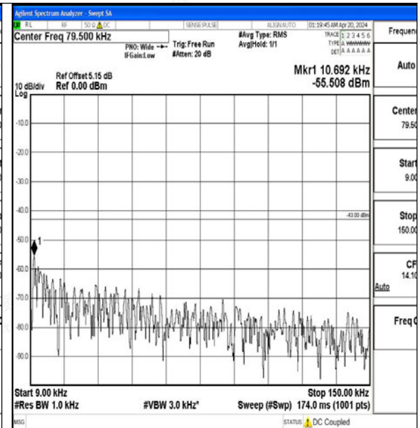
Band2_1.4MHz_16QAM_19193_1RB#0_0.009~0.15_0.009~0.15
