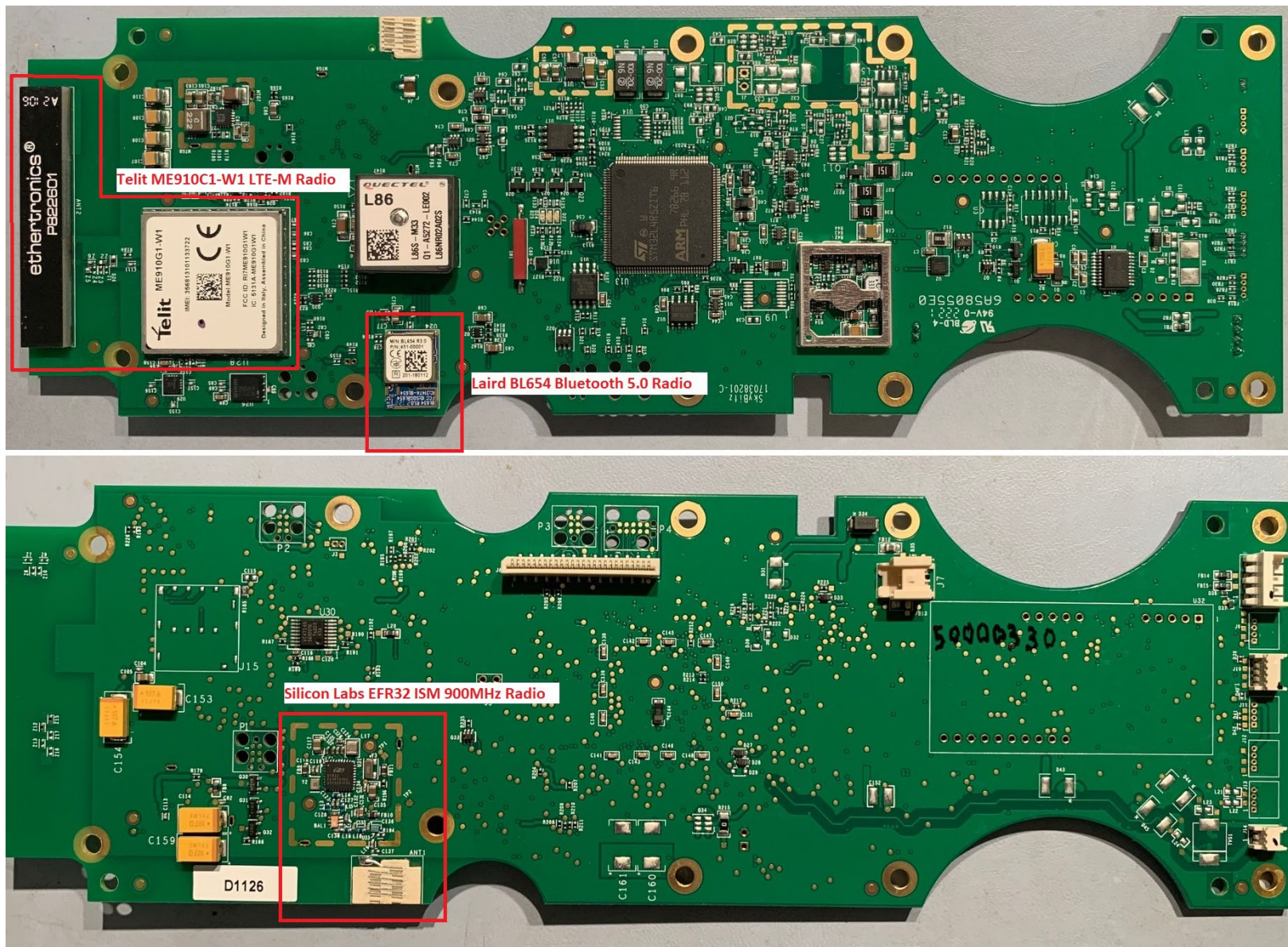
Figure 1: SHB6510 Internal Photo Showing Radio Locations
