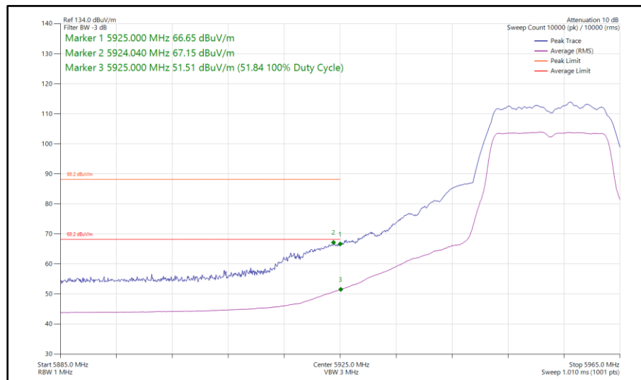
Figure 192 - 802.11a, SISO, Core 1 - 5955 MHz Band Edge Frequency 5925 MHz
