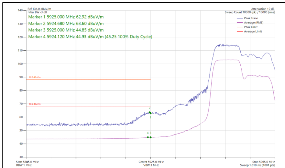
Figure 194 - 802.11ax HE20, RU 106-53, SISO, Core 1 - 5955 MHz Band Edge Frequency 5925 MHz
