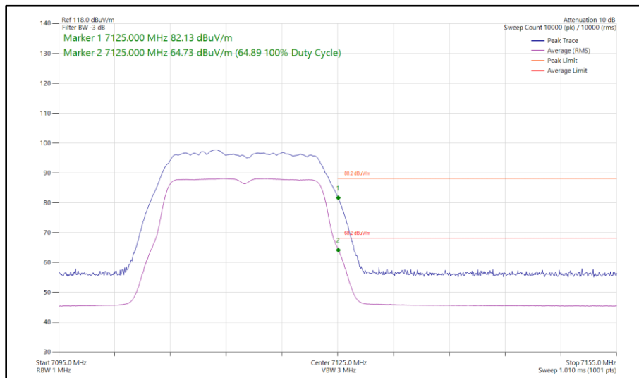
Figure 189 - 802.11a, SISO, Core 0 - 7115 MHz Band Edge Frequency 7125 MHz
