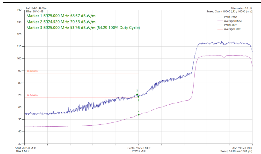
Figure 193 - 802.11ax HE20, SU, SISO, Core 1 - 5955 MHz Band Edge Frequency 5925 MHz
