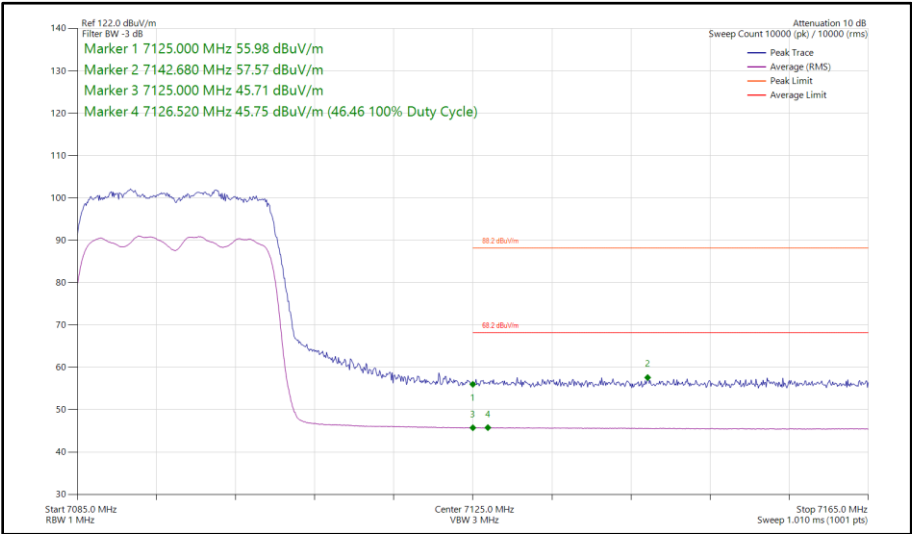
Figure 204 - 802.11ax HE20, SU, SDM, Core 0 - Core 1 - 7095 MHz Band Edge Frequency 7125 MHz
