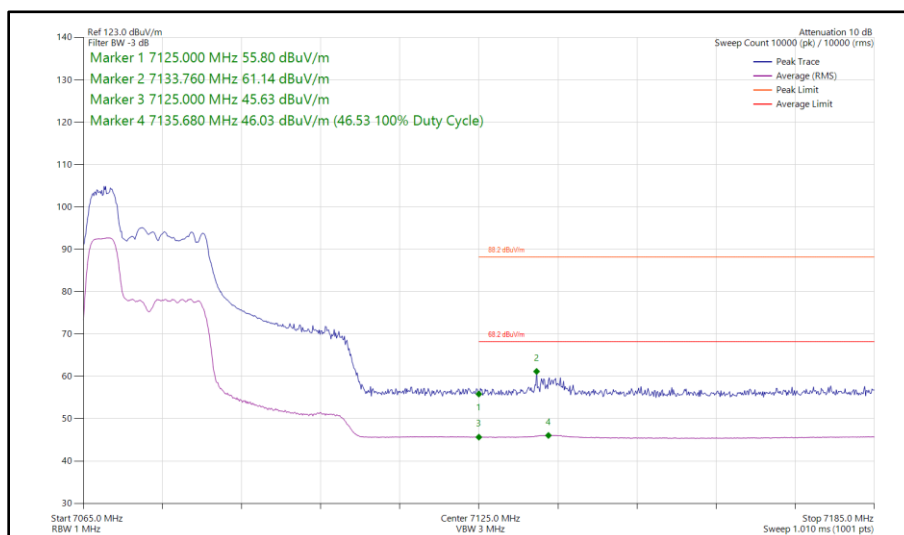
Figure 211 - 802.11ax HE40, RU 52-37, SISO, Core 0 - 7085 MHz Band Edge Frequency 7125 MHz
