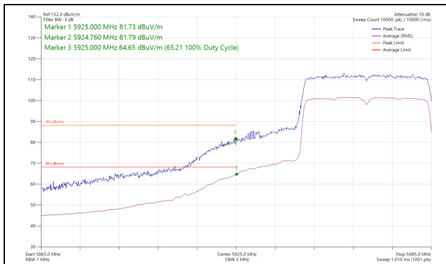
Figure 208 - 802.11ax HE40, SU, SISO, Core 0 - 5965 MHz Band Edge Frequency 5925 MHz
