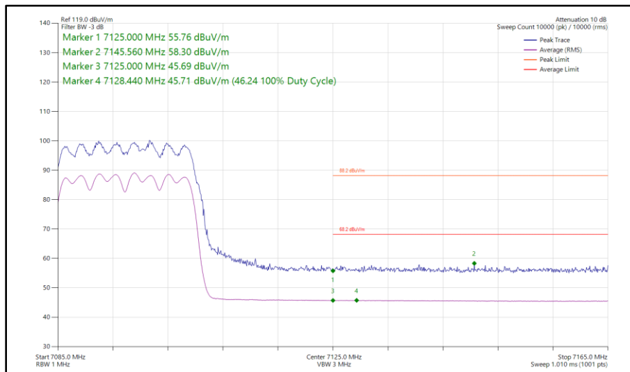
Figure 200 - 802.11ax HE20, SU, CDD, Core 0 - Core 1 - 7095 MHz Band Edge Frequency 7125 MHz
